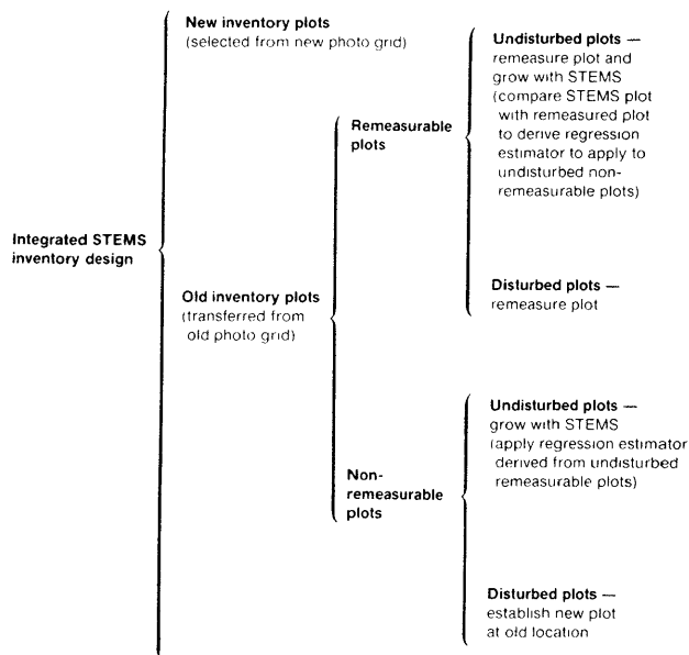
Figure 2.—Logic structure for the 1983 Wisconsin sample design.
