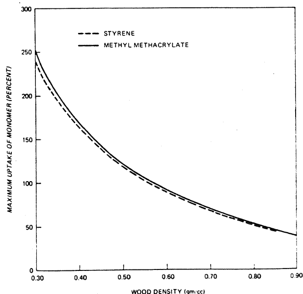
Figure 4.--Percent of maximum uptake of monomer for various wood densities.
