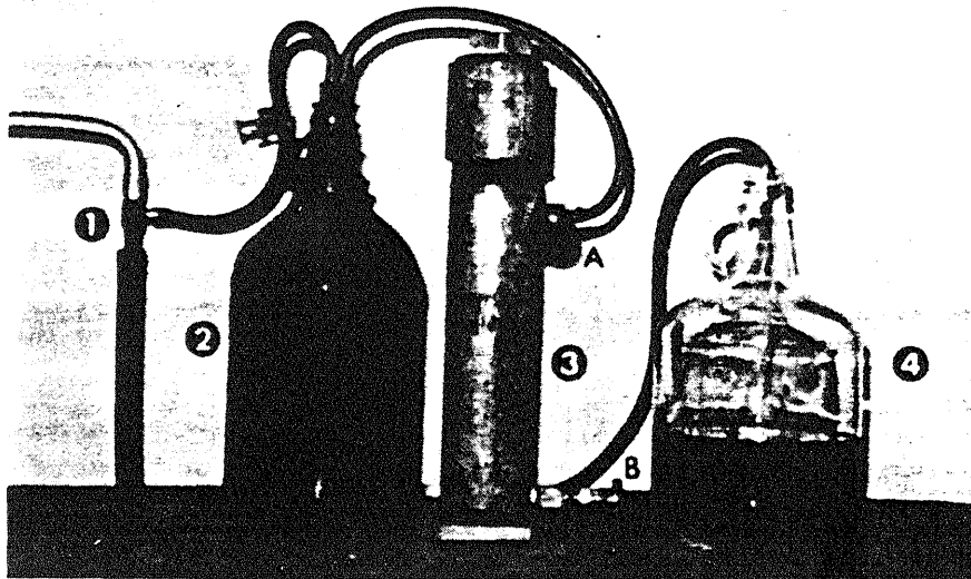
Figure 3.--Equipment arrangement for impregnation of monomer solution into the wood: (1) water aspirator, (2) surge tank, (3) impregnation tank, and (4) monomer supply tank.
