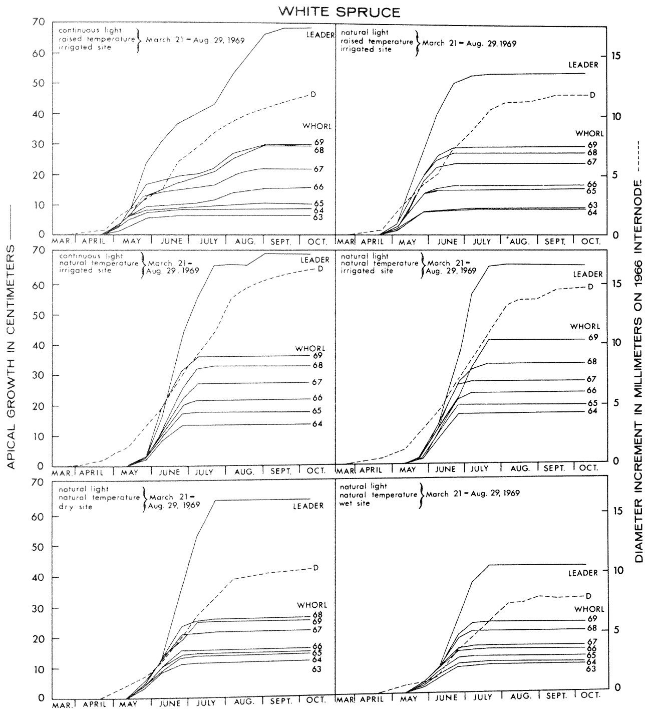
Figure 1.--Average leader (four trees per sample), lateral shoots (four branches per whorl), and diameter growth of 9-year-old white spruce grown under various combinations of photoperiod, thermoperiod, and soil moisture.
