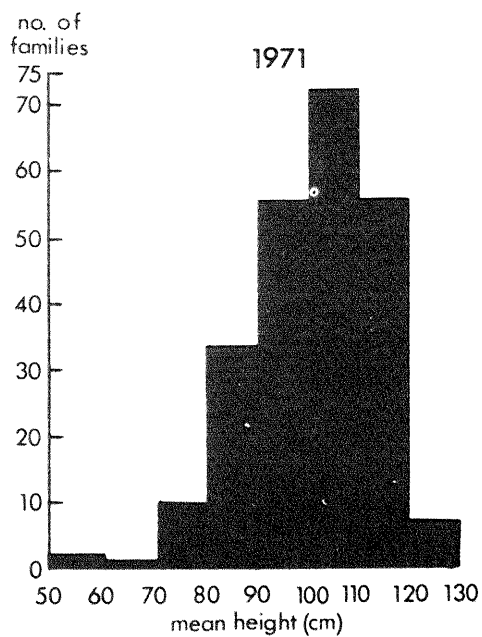
Figure 2.--Distributions of white spruce open-pollinated family means for height.
