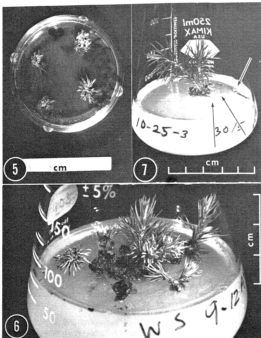
Figure 5.--Hypocotyl segments after a prolonged incubation on a medium containing high BAP and low NAA. Depletion of the growth regulators in the medium has allowed the scalelike outgrowths to elongate.
