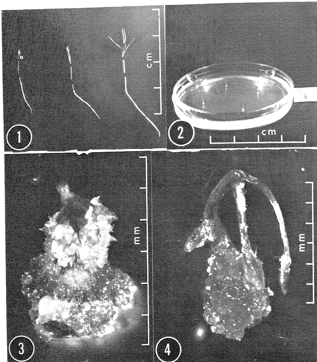
Figure 1.--Six to 12-day-old white spruce seedlings. A 5 to 7 mm segment of hypocotyl has been excised from each seedling taking care to exclude the apical meristem.
