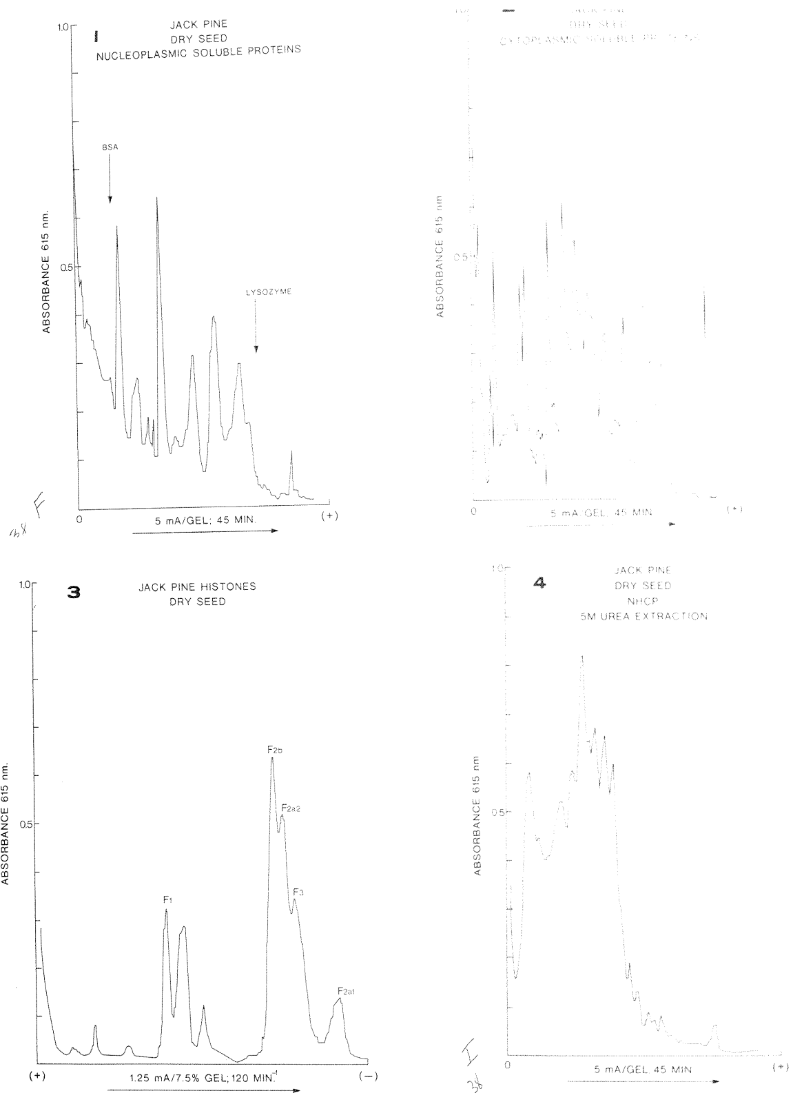
Fig. 1-4. Protein characterization of dry jack pine seed.
