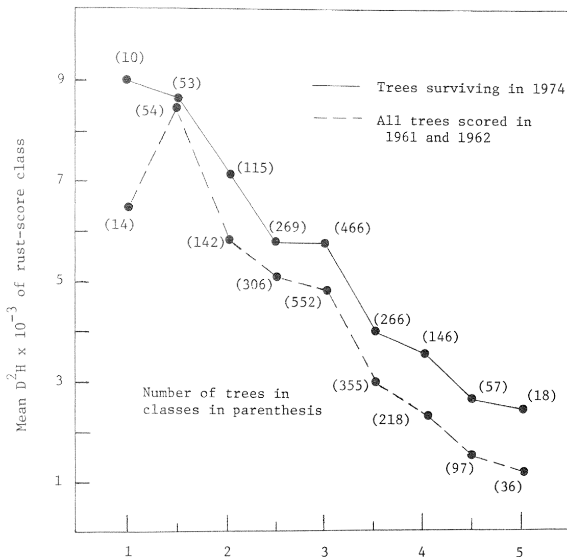
Figure 1.--Relation between Melampsora leaf-rust score and diameter squared x height of trees of Illinois seed origin in a 15-year-old plantation in central Illinois
