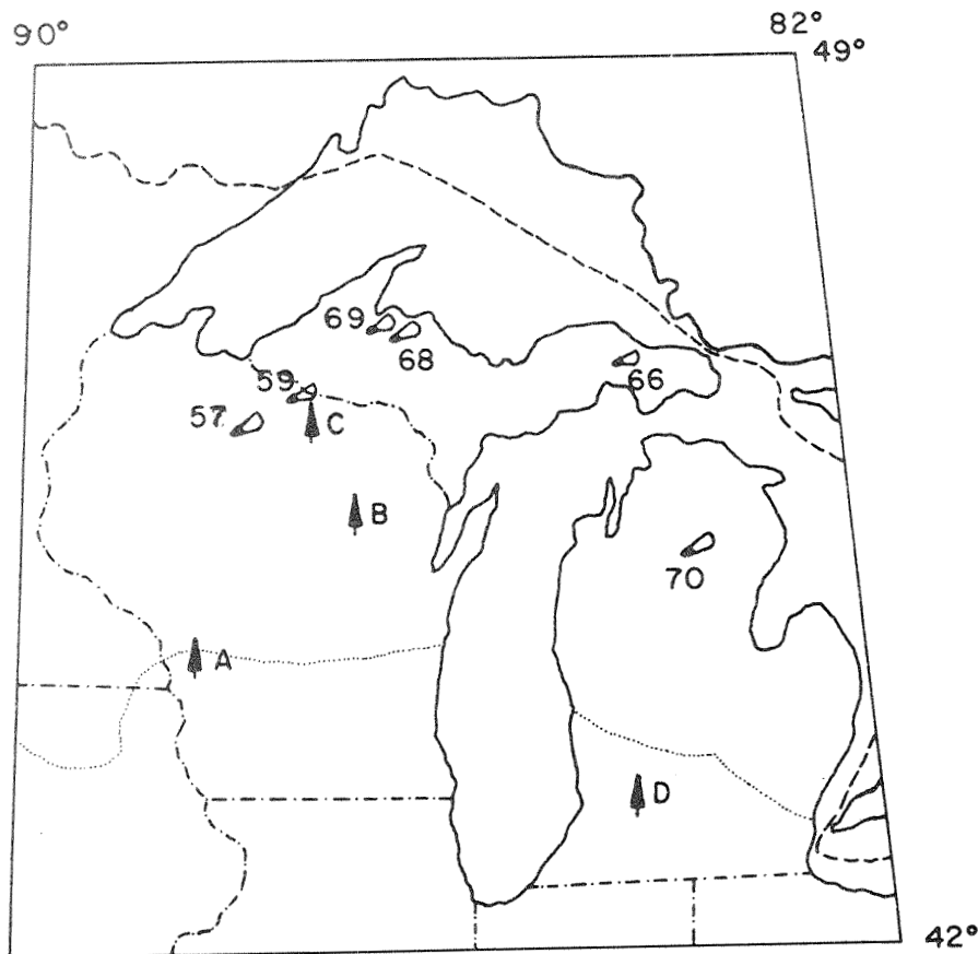
Figure 1.--Map of the study area with numbered provenance locations (●) and plantation locations (▲). The southern boundary of the botanical range of balsam fir is indicated by a dotted line.
