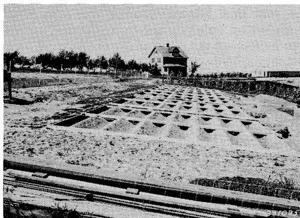
Figure 3.—Forest Service lysimeters during test period, Soil Erosion Station, 1934.
