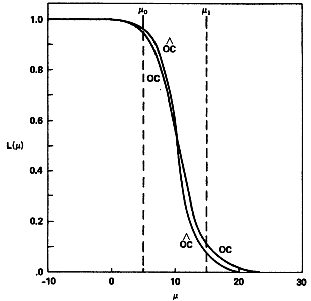
Figure 3. — Comparison of Wald's and the Monte Carlo Operating Characteristic (OC) functions for the lodgepole needleminer sequential sampling plan (table 4).
