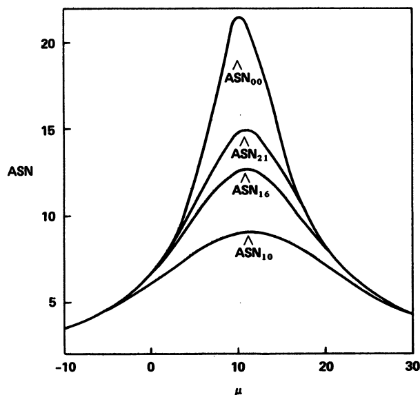
Figure 7. — Comparison of Monte Carlo Average Sample Number (ASN) functions for sequential sampling plans ( \mu_0 = 5 , \mu_1 = 15 , \sigma = 15.62 , \alpha = 0.05 , and \beta = 0.10 ) for truncation points of N = 10, 16, 21 , and \infty .
