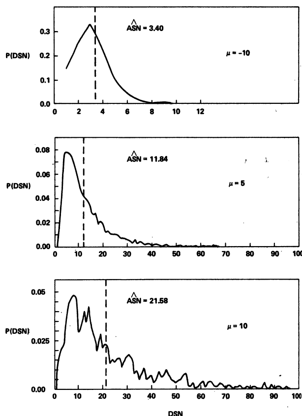
Figure 5. — Empirical distributions of the Decisive Sample Number (DSN) for three values of \mu for Wald's Sequential Probability Ratio Test (SPRT) with \alpha = 0.05 and \beta = 0.10 . The dashed line shows the mean Average Sample Number (ASN) for each DSN distribution.
