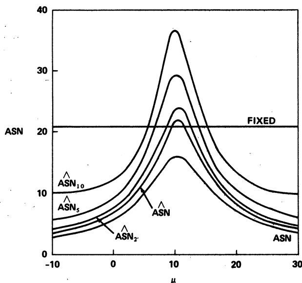
Figure 4. — Comparison of Monte Carlo Average Sample Number ( \hat{ASN} ) functions for sequential sampling plans with \mu_0 = 5 , \mu_1 = 15 , \sigma = 15.62 , \alpha = 0.05 , and \beta = 0.10 , for numbers of observations taken at each stage of the plan equal to 1, 2, 5, and 10. The ASN function for the fixed sample size plan with equal reliability is also shown.
