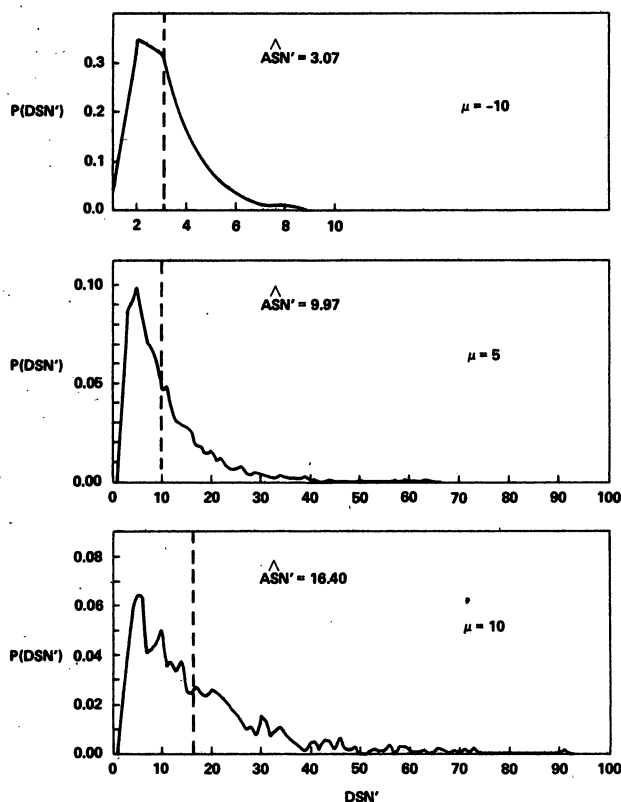
Figure 6. — Empirical distributions of the Decisive Sample Number (DSN') for three values of \mu for Wald's Sequential Probability Ratio Test (SPRT) with \alpha' = 0.0714 and \beta' = 0.1389 . The dashed line shows the mean Average Sample Number (ASN') for each DSN distribution.
