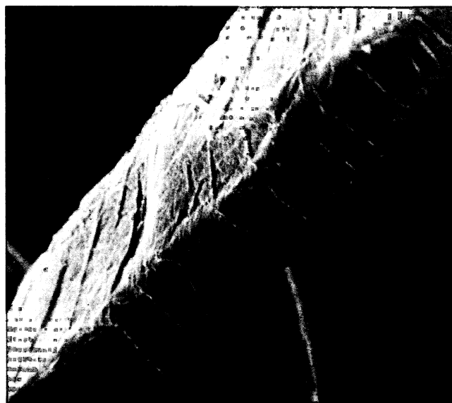
Scanning electron micrograph of a tension wood fiber from short rotation intensively cultured Populus tree. Surface dislocations (wrinkles) on the fiber affect subsequent paper strength properties (2000 X).
