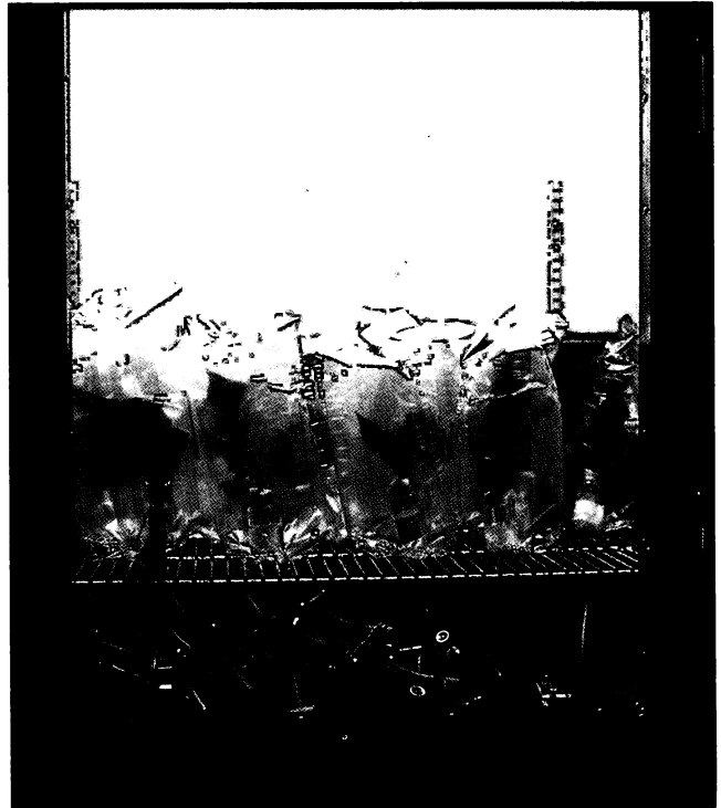
The \text{CO}_2 compensation point of excised Populus leaves is measured in the laboratory. Such information about physiological responses may be used to preselect clones before expensive field screening is conducted.
