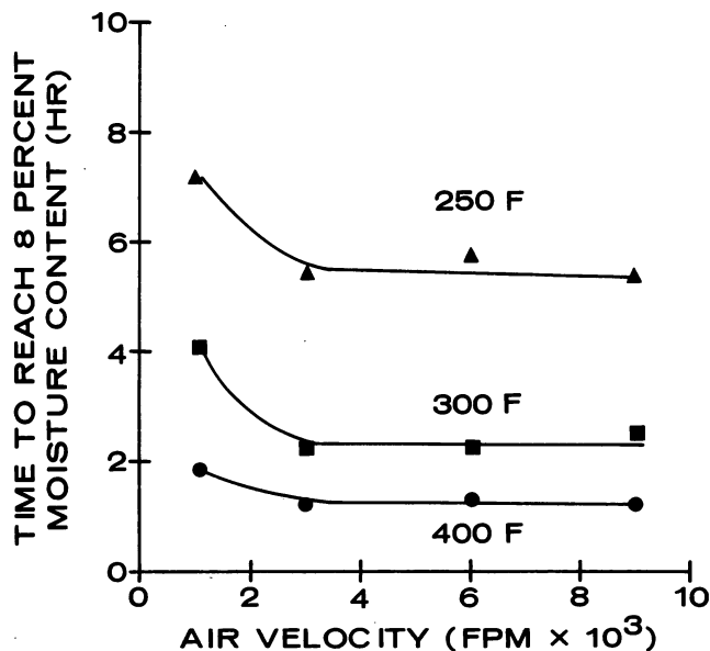
Figure 4.—Influence of air velocity on drying time of ¼-inch silver maple at various dry bulb temperatures (180°F wet bulb). Each point is the average of six boards.
