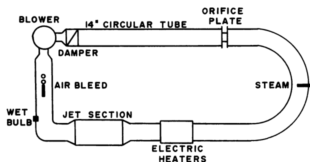
PROTOTYPE JET DRYER LAYOUT
