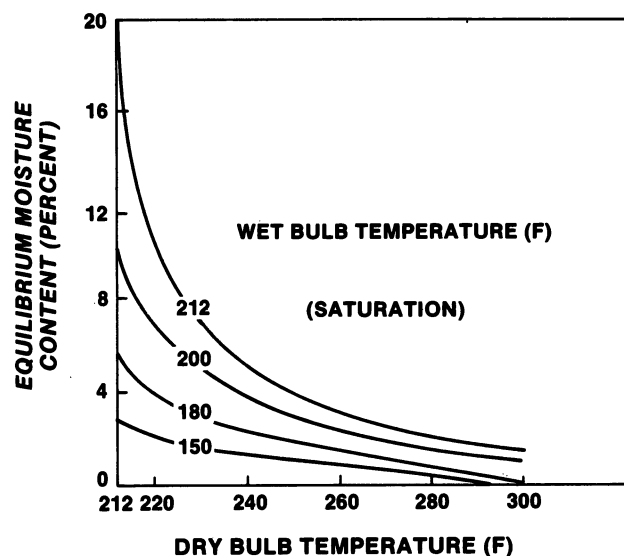
Figure 5.— High temperature equilibrium moisture content of air-water vapor mixtures at atmospheric pressure (Kauman 1956). The saturation curve at 212°F wet bulb is the maximum equilibrium moisture content obtainable at a given dry bulb temperature.
