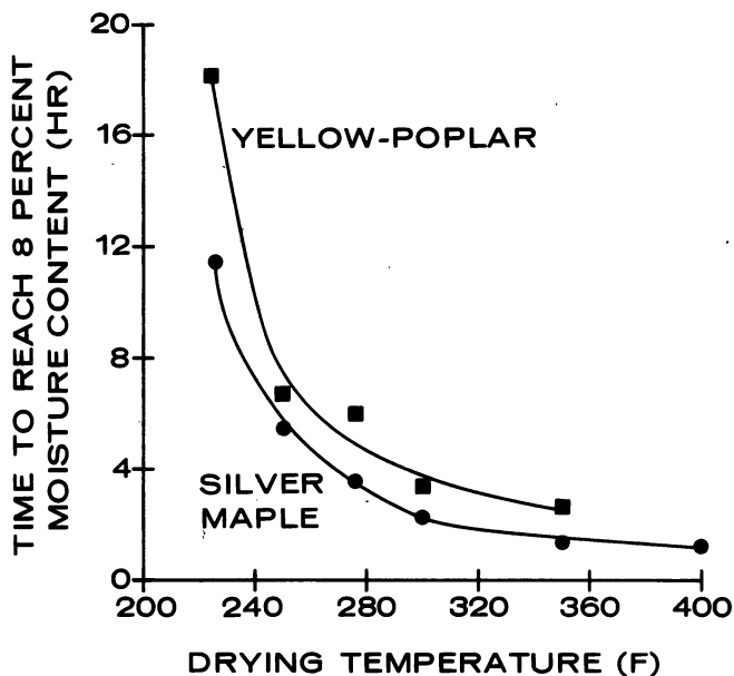
Figure 3.—Influence of temperature on drying time of ¼-inch silver maple and yellow-poplar at 3,000 fpm air velocity and 180°F wet bulb. Each point is the average of six boards.
