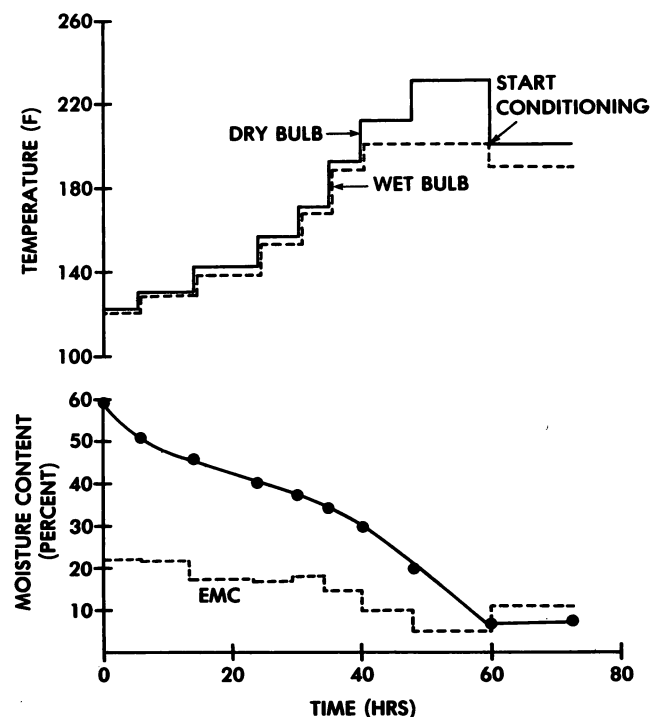
Figure 7.—Drying schedule and moisture contents for jet-dried \frac{3}{4} -inch black walnut. The top graph shows dry bulb (solid line) and wet bulb (dotted line) temperatures versus time. The bottom graph shows the moisture content (solid line—each point is an average of two boards) and the EMC (dotted line) associated with the dry and wet bulb temperatures of the top graph.
