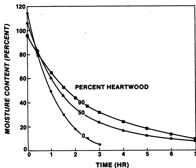
Figure 6.— Typical drying curves of \frac{1}{4} -inch yellow-poplar at 300°F (200°F wet bulb and 3,000 fpm air velocity), showing the influence of heartwood content of the wood on drying rate.
