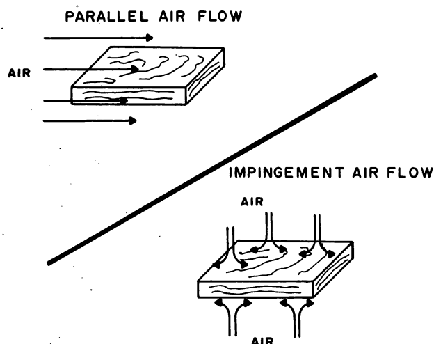
Figure 1.— Direction of flow relative to the board surface for impingement and parallel air flow.
