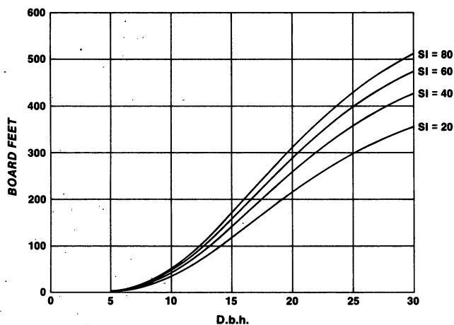
Figure 2.—Net board foot volume (International 1/4-inch rule) of desirable and acceptable basswood trees by d.b.h. and selected site index levels.
