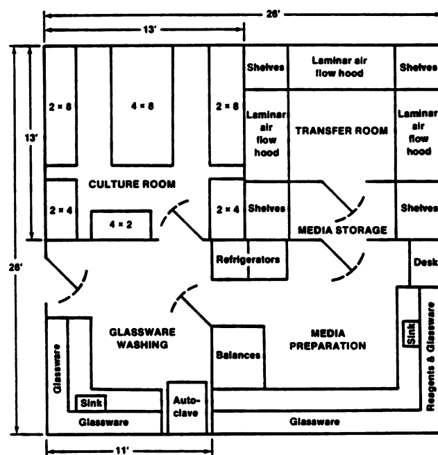
Figure 1.—Floor plan of a hypothetical laboratory facility for the propagation of plants through shoot apex culture.
