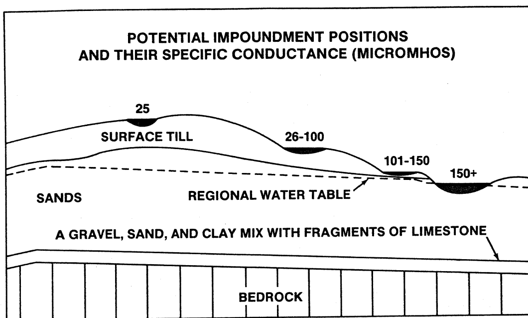
Figure 2.--A typical geologic setting for wetlands in north central Minnesota. Water supply to wetlands can be increased if the wetland water table is the same as the regional water table.
