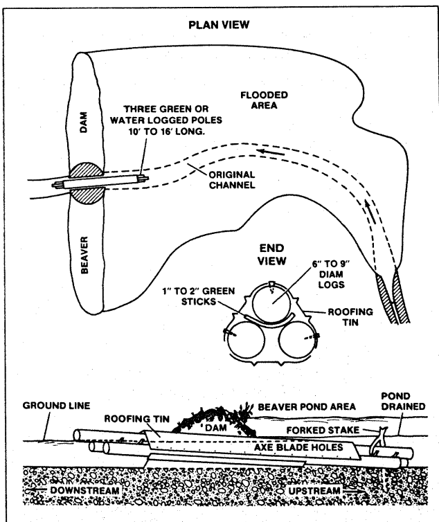
Figure 2.--The "3-log drain" proposed by Bailey (1927) for regulating water levels in beaver ponds.
