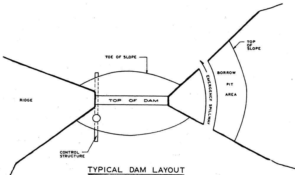
Figure 1.--Typical dam showing borrow pit and emergency spillway.
