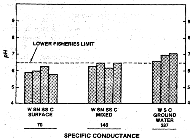
Figure 9.--pH means in impoundments during winter (W), summer-normal flow (SN), and summer-stagnant (SS) conditions; and nonimpounded control areas in all seasons (C). The three groups of data represent impoundments with different water sources. These are indexed on specific conductance values at summer-normal conditions: surface water only (70), an equal mixture of surface and groundwater (140), and groundwater dominated (287). Bars shaded the same are statistically equal at the 95 percent level of confidence within conductance groups.
