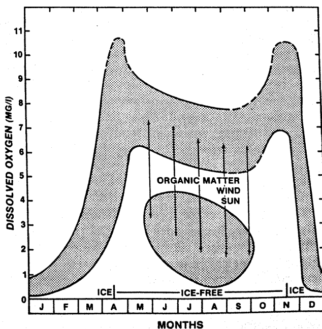
Figure 6.--Dissolved oxygen in shallow water impoundments (daytime, near surface measurements). During the summer concentrations move between the upper and lower shaded areas rapidly as organic matter is processed and wind mixing or photosynthesis occurs. Dashed lines depict areas of limited data.
