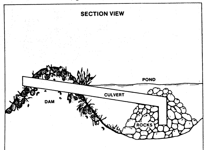
Figure 5.--A proposed culvert treatment for reducing problems with beaver.
