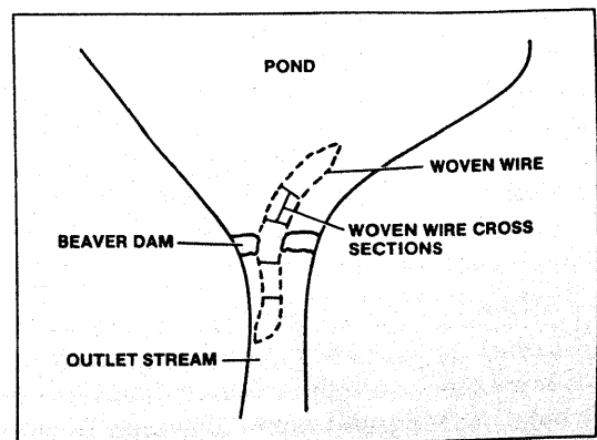
Figure 4.--The "beaver baffle", a fencing arrangement proposed by Guenther 1956 for regulating water levels in beaver ponds.
