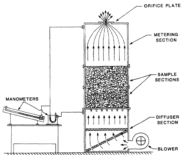
Figure 2.—Test setup diagram.
