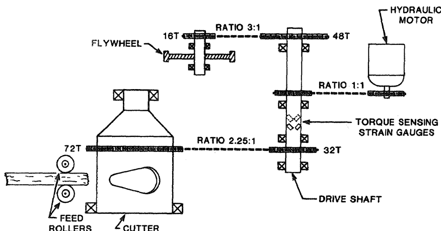
Figure 4.—Schematic of Teardrop Chunker drive train.
