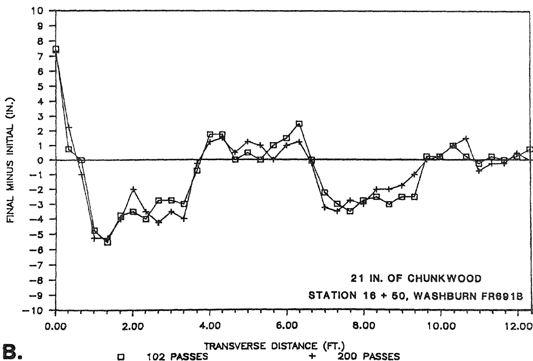
Figure 5.—Measurement of road rutting caused by test vehicle. A. Transverse profilometer board used to measure transverse road profile. B. Typical graphic representation of rutting in a roadbed profile.
