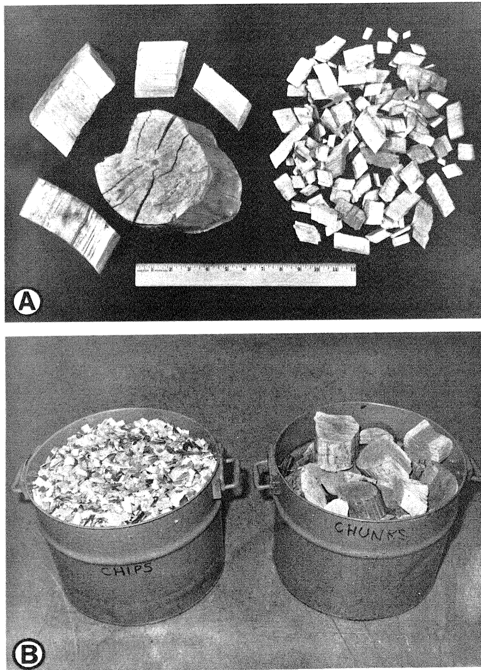
Figure 1.—A. Typical chunks and chips. B. Test setup for exploratory indoor natural convective air drying.
