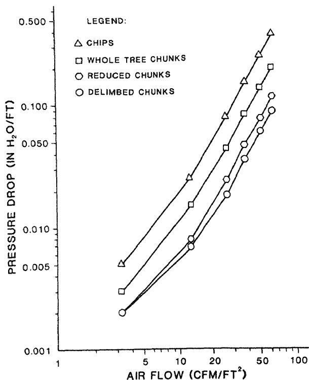
Figure 4.—Log-log plot of pressure drop versus airflow for chips and for whole-tree, delimbed, and reduced chunks. Each data point represents the mean value of six replications.
