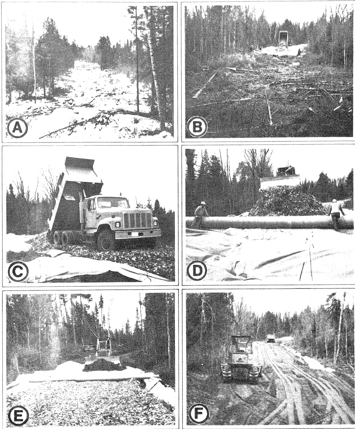
Figure 2.—Swamp crossing at FR 481 (Hayward site): A. Right-of-way clearing; B. Ungrubbed swamp in foreground; C. Dumping of chunkwood onto geotextile fabric; D. Installation of culvert; E. Application of geotextile fabric and gravel over chunkwood base; F. Nearing completion of swamp crossing.
