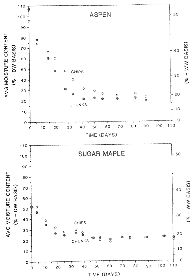
Figure 7.—Drying curves for outdoor air drying of aspen and sugar maple chunks and chips. (Based on the average of two replications.)
