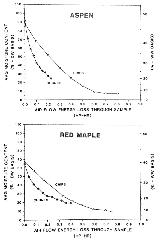
Figure 5.—Energy used in indoor forced air drying of aspen and red maple chunks and chips. (Based on the average of five repetitions.)
