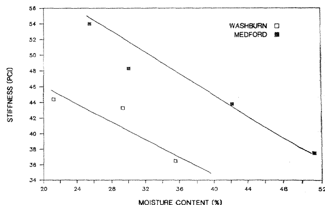
Figure 10.—Relationship between chunkwood sample stiffness and moisture content. WAS = Washburn site (sugar sand) and MED = Medford site (wet, silty clay).
