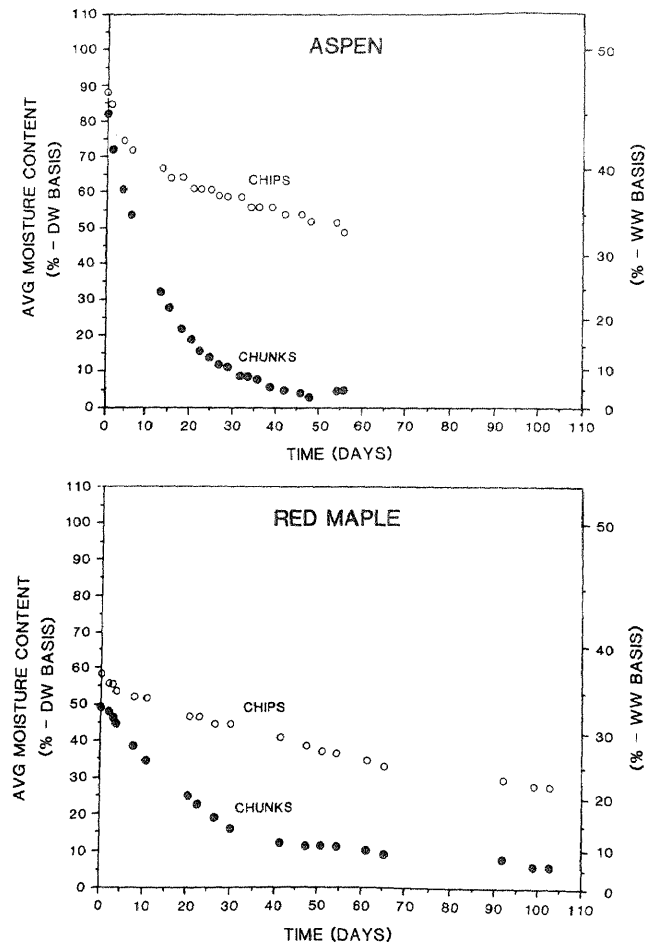
Figure 2.—Drying curves for indoor natural convective air drying of aspen and red maple chunks and chips.
