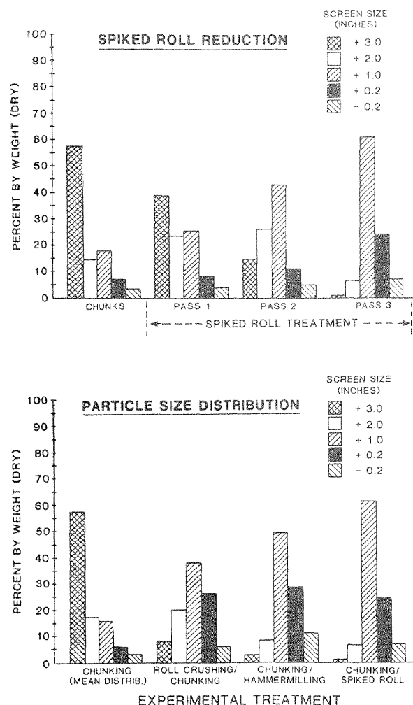
Figure 8.—Particle size distribution: A. After successive passes through the spiked roll assembly; B. By experimental treatment.
