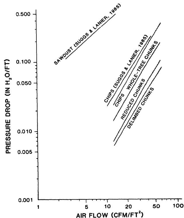
Figure 5.—Comparison of the pressure drop regression lines for the chunkwood and chips tested and those published by Suggs and Lanier (1985) for green chips and sawdust.
