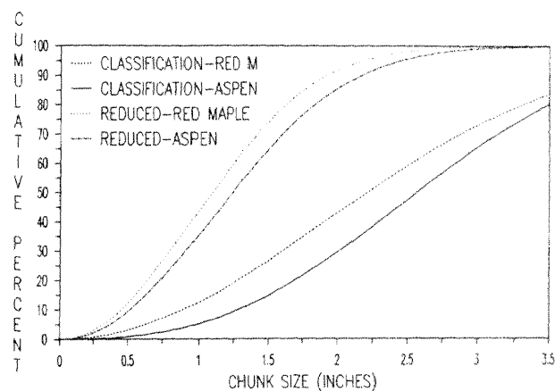
Figure 7.—Weibull curves for hammermill data.
