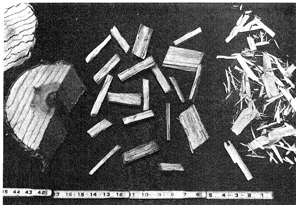
Figure 6.—Aspen chunks produced by the USDA Forest Service involuted disk chunking machine, fingerlings that were split from chunks in the Institute of Wood Research prototype chunkwood splitter, and ring flakes made from the fingerlings.
