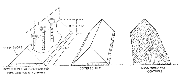
Figure 8.—Three windrow pile treatments for drying chunkwood.
