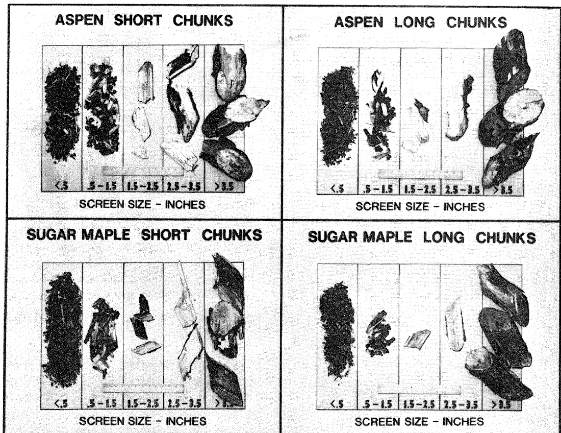
Figure 3.—Typical particles produced by the Teardrop Chunker using two species, aspen and sugar maple, and two chunk lengths, short and long. (Volumes shown are approximate proportions.)
