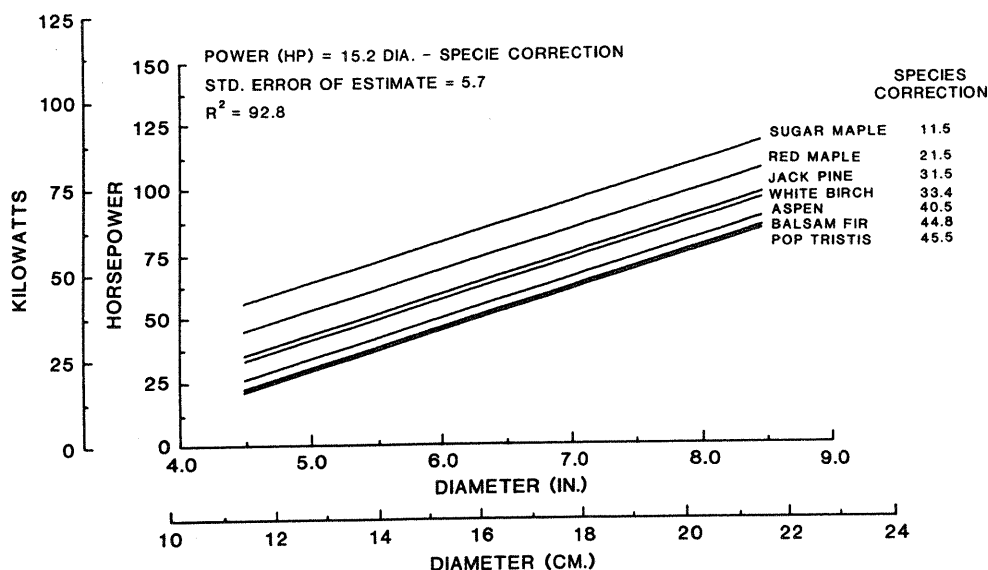
Figure 5.—Power required to chunk logs of different diameters from several tree species.
