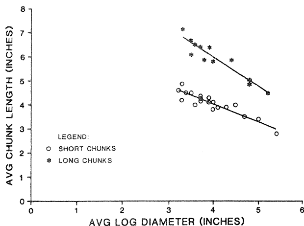
Figure 6.—Test data and the linear regression lines for average chunk lengths produced for short and long chunk production settings.
