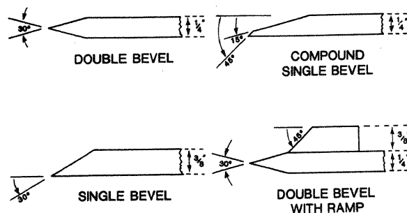
Figure 4.—Schematic of chunker blades.
