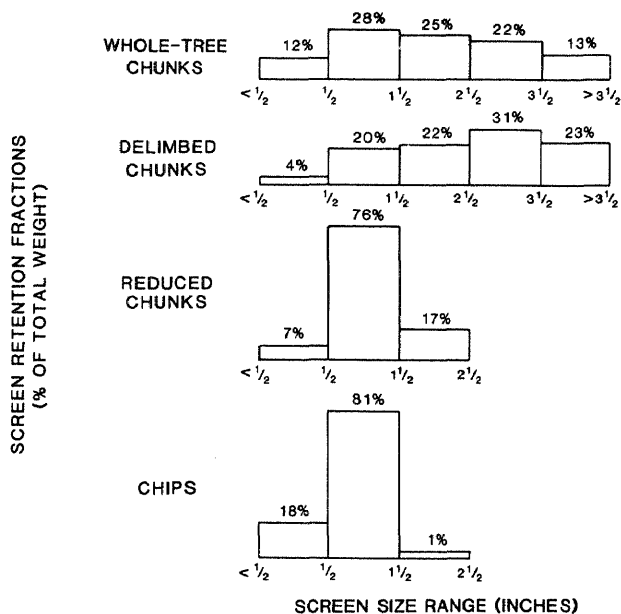
Figure 3.—Particle size distributions for the chunkwood and chips tested. Percent of total weight retained for five screen size ranges.
