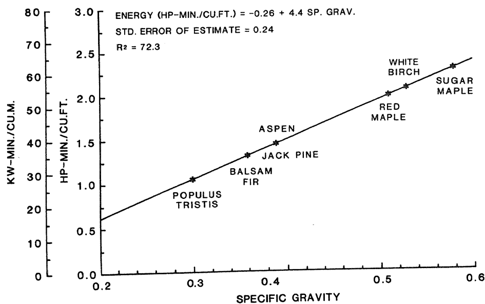
Figure 4. —Energy required to chunk wood from several tree species with different specific gravities.
