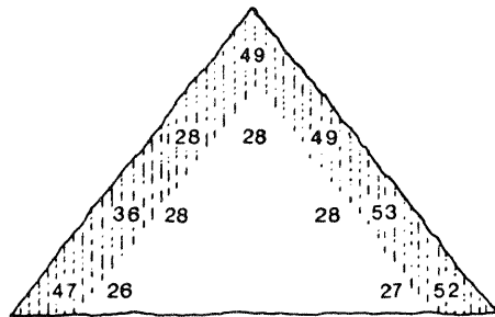
UNCOVERED PILE
