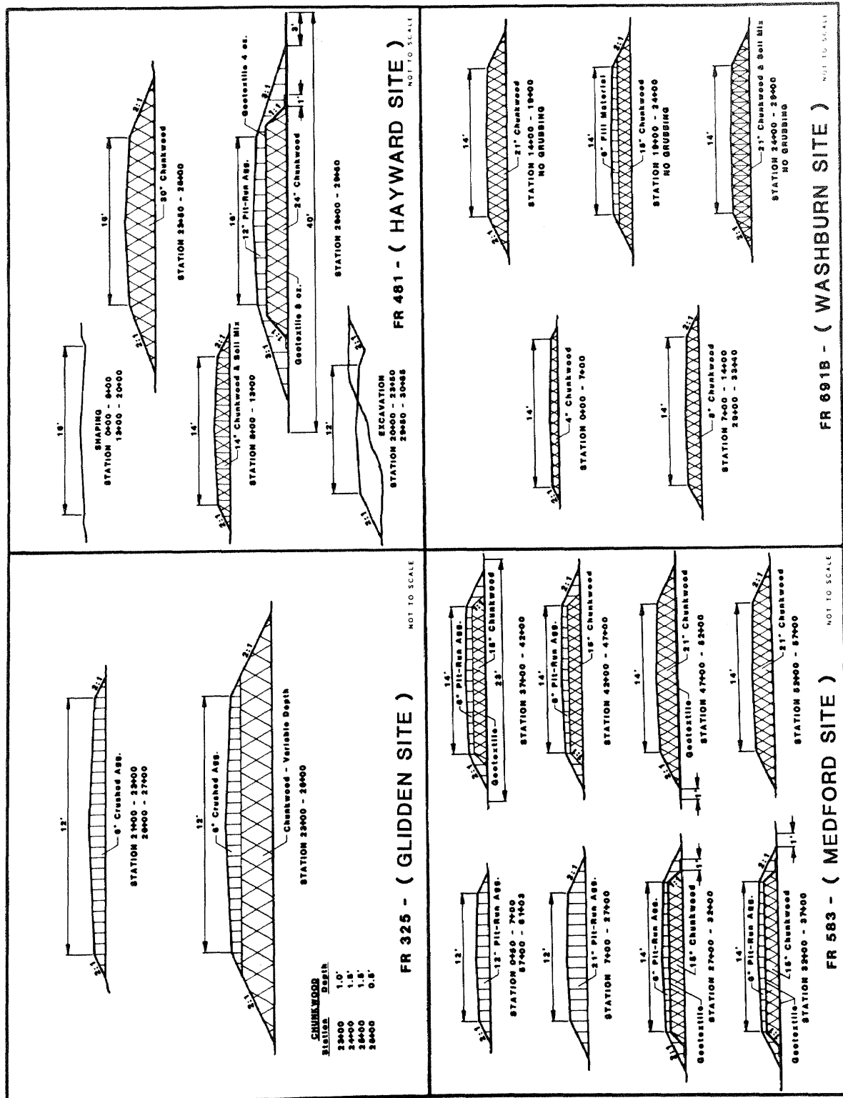
Figure 1.—Typical cross sections of chunkwood test demonstration roads.
