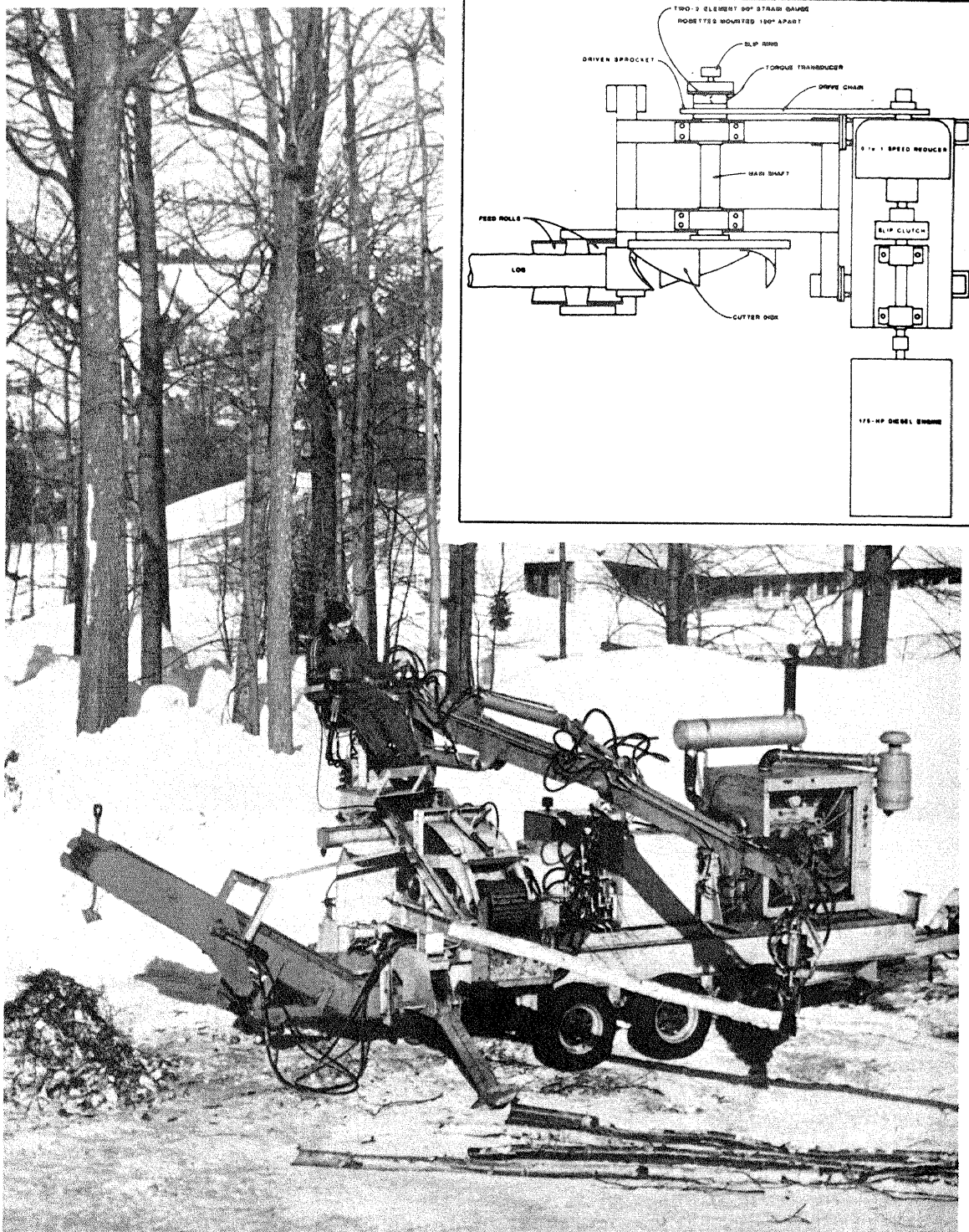
Figure 2.—Photo and schematic of chucker.
