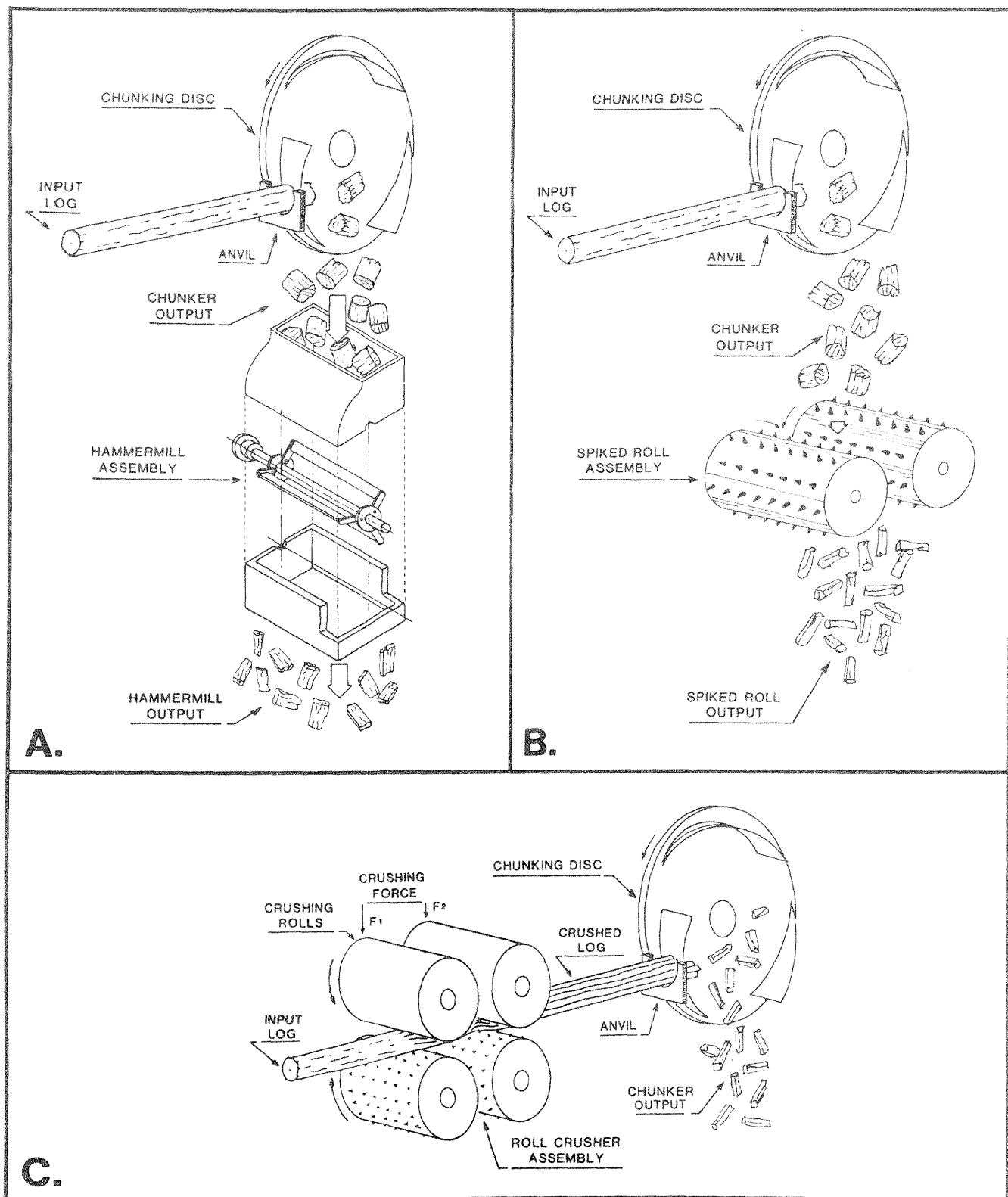
Figure 6.—Three experimental reduction methods used to obtain intermediate-sized particles.
