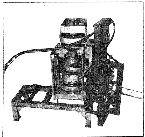
Figure 1.—The Multi-Product Wood Processor or “Teardrop Chunker.”
