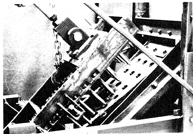
Figure 5.—Chunkwood splitter from the Institute of Wood Research at Michigan Technological University.
