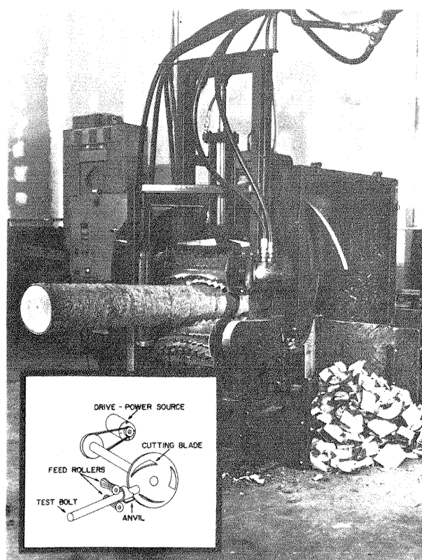
Figure 1.—Experimental involuted single-disc wood chunker with simplified schematic insert.
