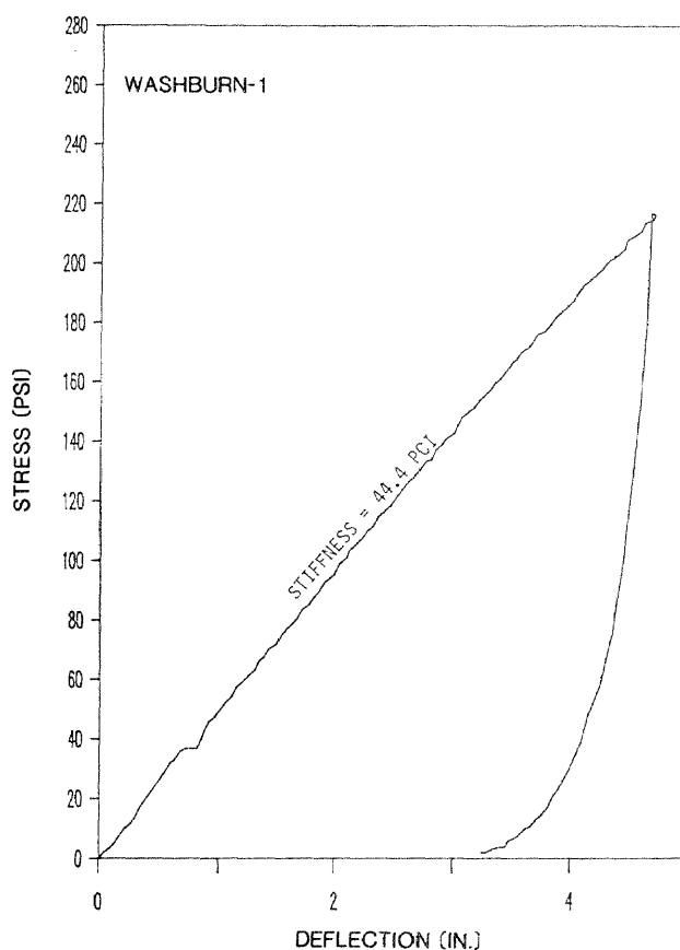
Figure 9.—Chunkwood stiffness index as illustrated by a typical plate load stress/displacement plot.
