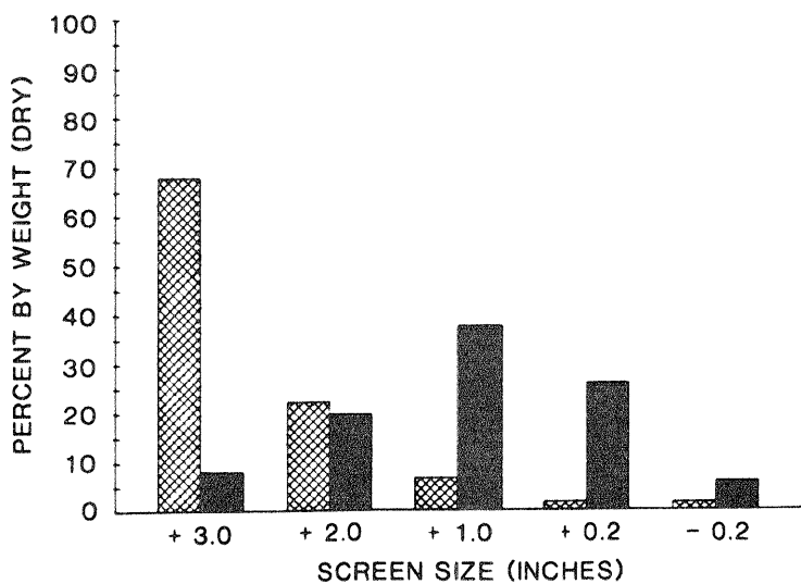
Figure 7.—Mean before-and-after particle size distribution for the three experimental reduction methods used.
