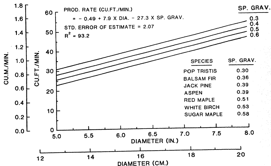
Figure 6.—Production rate of the experimental wood chunker when chunking logs with different diameters.
