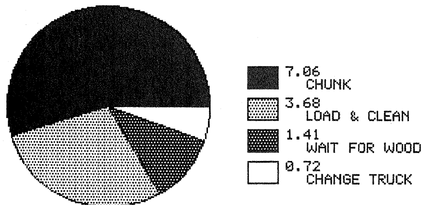
Figure 11.—Productivity and time breakdown when chunking with the Missoula field demonstration prototype.
