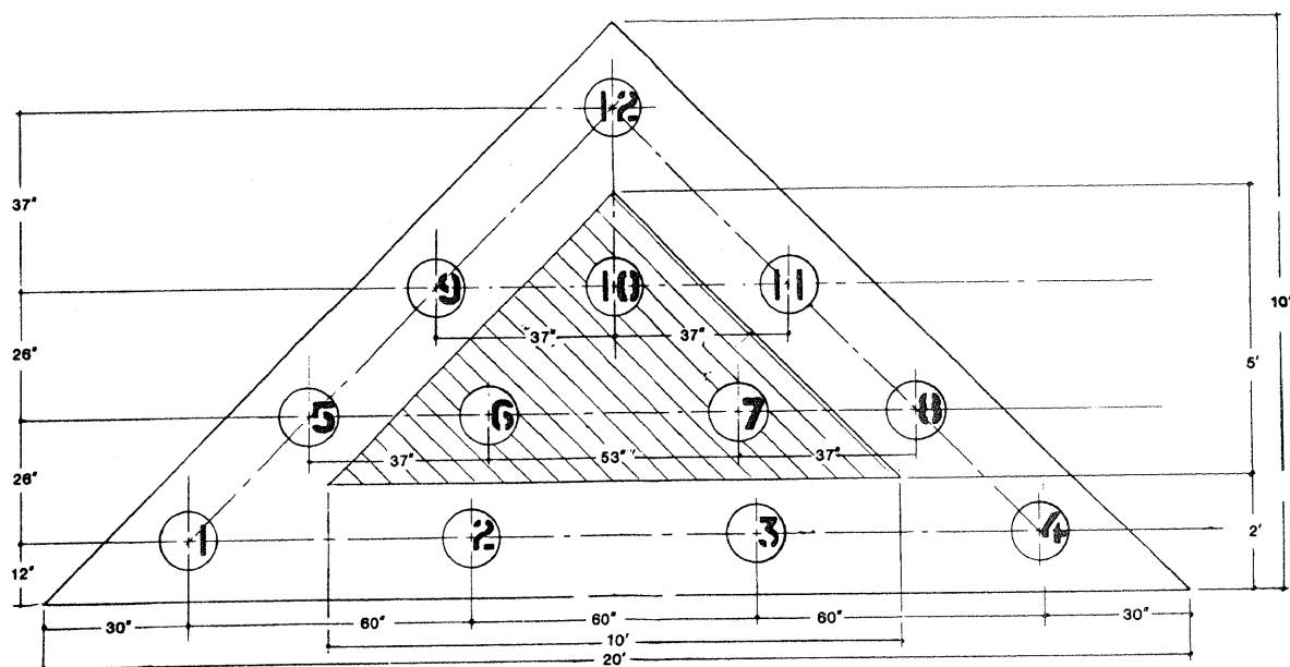
Figure 9.—Transverse pile locations of bags of chunkwood for moisture content determinations.
