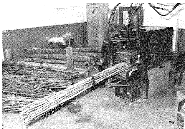
Figure 7.—Chunking bundled stems with the involuted single-disc wood chucker.
