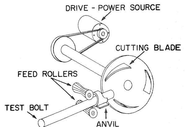
Figure 3.—Diagram of USDA Forest Service chunker.
