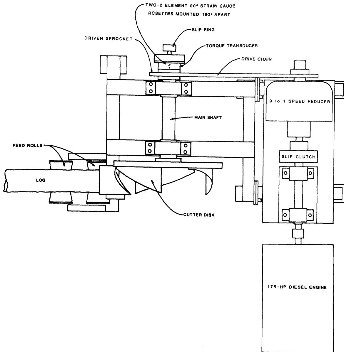
Figure 3.—Schematic of experimental wood chunker and drive system.
