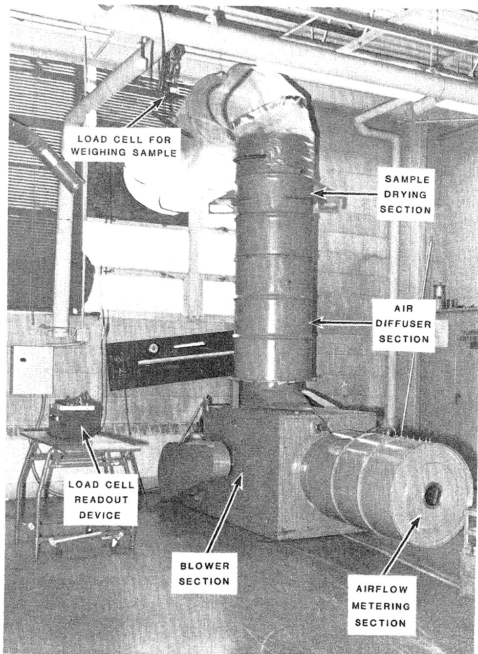
Figure 3.—Test setup for exploratory indoor forced air drying.
