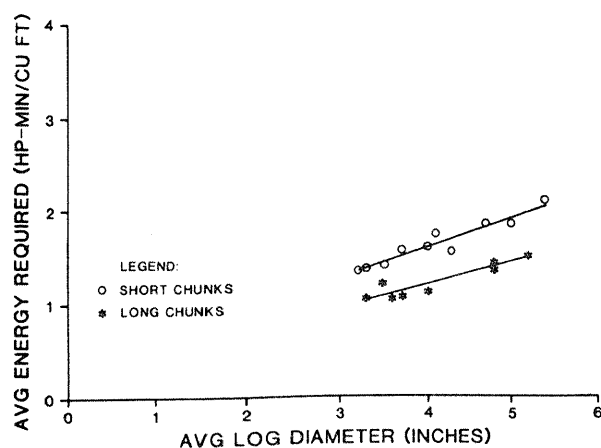
Figure 10.— Test data and the linear regression lines for average energy required to produce aspen short and long chunks.
