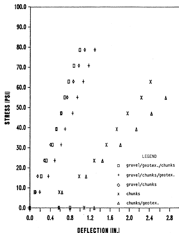
Figure 6.—Plate load test results for FR 583 (Medford) after 105 test truck passes over various chunkwood road test sections.
