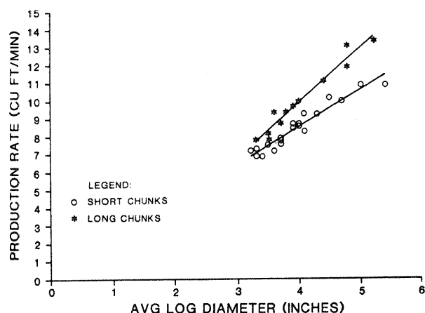
Figure 7.—Test data and the linear regression lines for production rates developed producing short and long chunks.
