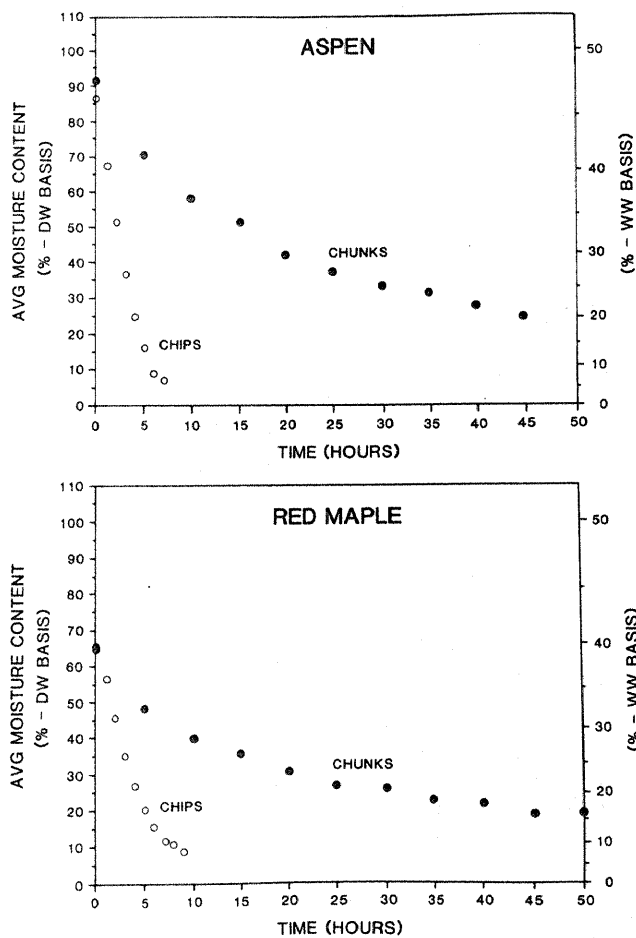
Figure 4.—Drying curves for indoor forced air drying of aspen and red maple chunks and chips. (Based on the average of five repetitions.)
