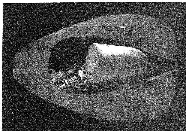
Figure 5.—Teardrop-shaped cutter opening on the Teardrop Chunker.
