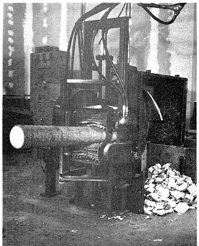
Figure 2.—USDA Forest Service chunker.
