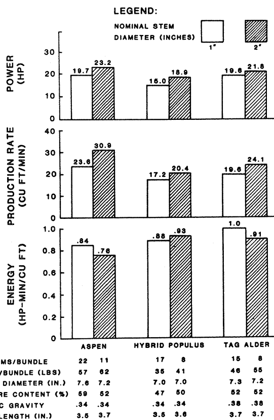
Figure 8.—Power, energy, and production rates for chunking bundled stems of three species with the involuted single-disc wood chucker.
