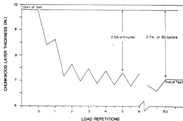
Figure 7.—Typical laboratory compaction record illustrating the characteristic behavior of confined chunkwood to repeated loadings.
