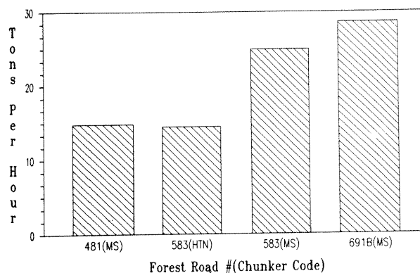
Figure 4.—Mean chunkwood production rates. (MS and HTN indicate the Forest Service Missoula and Houghton prototype chunkwood machines.)
