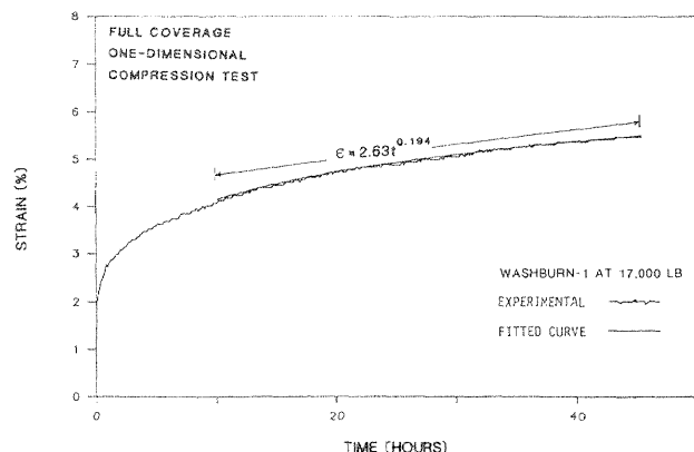
Figure 8.—Compressibility of chunkwood as illustrated by a typical full coverage, one-dimensional compression test result.
