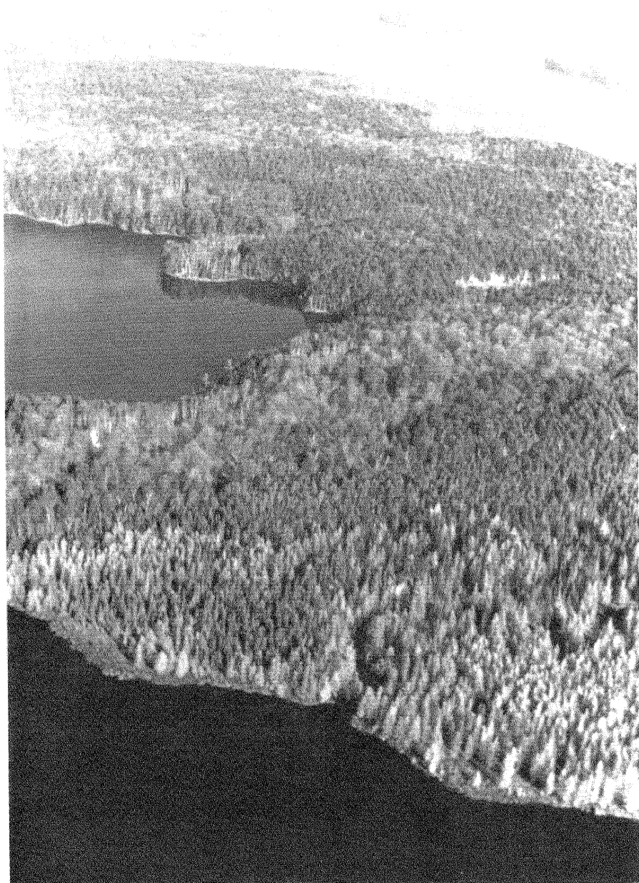
Figure 26.—Subsection IX.5: Plum Lake-Star Lake Hemlocks, Vilas County, Wisconsin. The pitted outwash forms a landscape of kettle lakes and fire-dependent forests of white pine, red pine, red oak, and paper birch growing on flat, sandy plains. From the air, this landscape superficially resembles that of the Winegar moraine (sub-subsection IX.3.2) immediately to the north. Upon closer examination, the forests of the steep, irregular Vilas moraine are dominated by northern hardwoods and eastern hemlock. Photo by E. Epstein.
