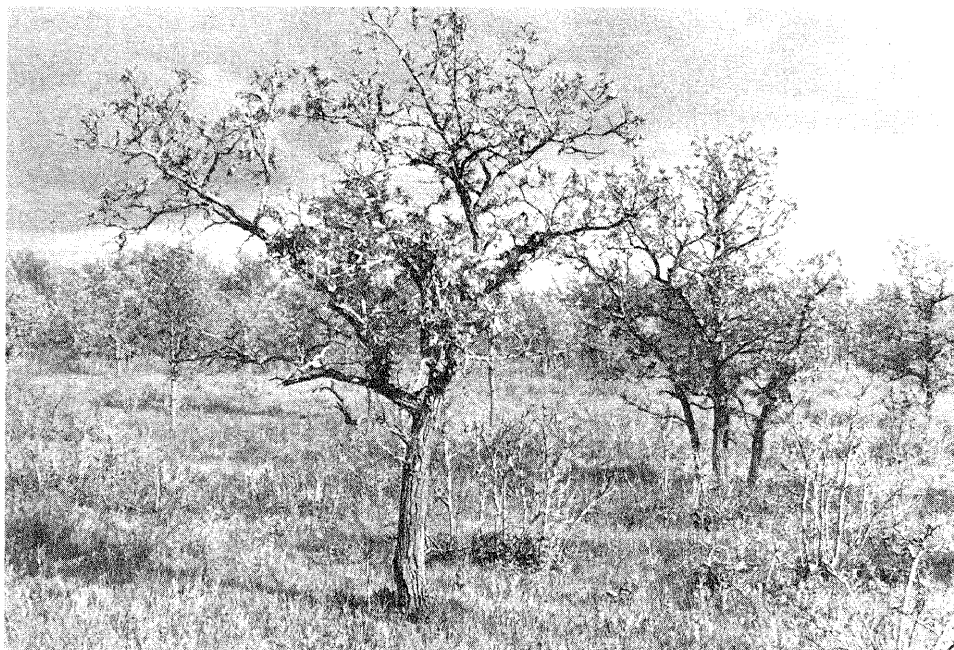
Figure 36.—Subsection XI: Twin Lakes Wildlife Management Area, Kittson County, Minne- sota. Stunted bur oak grow on a gravelly beach ridge of Glacial Lake Agassiz. Bur oak dominates the driest sites as long as fires occur frequently. Trembling aspen is more common on more mesic sites and replaces bur oak when fires are eliminated. Minnesota Department of Natural Resources photo by C.K. Con- verse.
