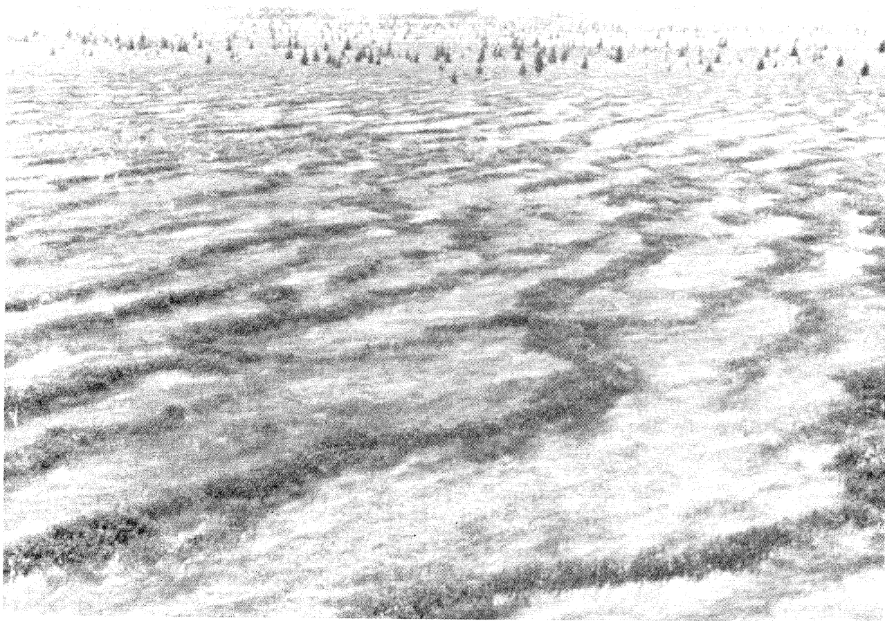
Figure 35.—Subsection X.12: Winter Road Lake Peatland State Natural Area, Lake of the Woods County, Minnesota. Large patterned peatlands occupy the flat, poorly drained topography of Glacial Lake Agassiz. The wetter portions of the peatland, called flarks, are dominated by Carex lasiocarpa and other sedges, while the drier portions, called strings, are dominated by shrubs. Scattered small black spruce and tamarack occur within the peatland, often where there are low ridges of mineral soil. Minnesota Department of Natural Resources photo by B. Coffin.
