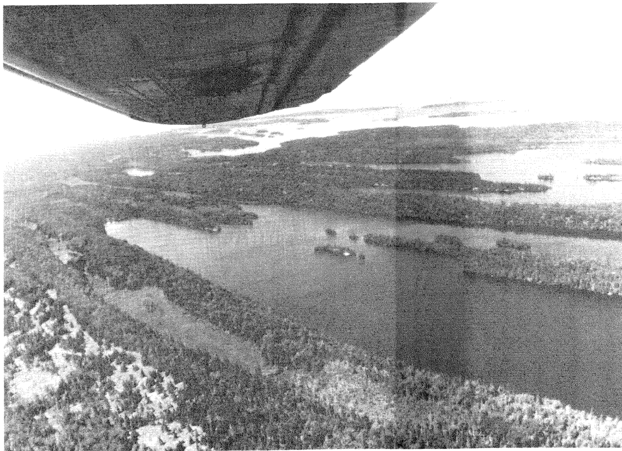
Figure 27.—Sub-subsection IX.7.3: Isle Royale Wilderness Natural Park, Michigan. Isle Royale was formed from the extensive Keweenaw-age lava flows. The lava flows more resistant to erosion by waves and ice remain as small islands off the coast of Isle Royale; the less resistant flows have been eroded away. The lava, which was laid down as numerous, thin horizontal layers on land, has been greatly deformed; the layers now slope at 30 to 40 degrees from the horizontal. Photo by P. Melhop.
