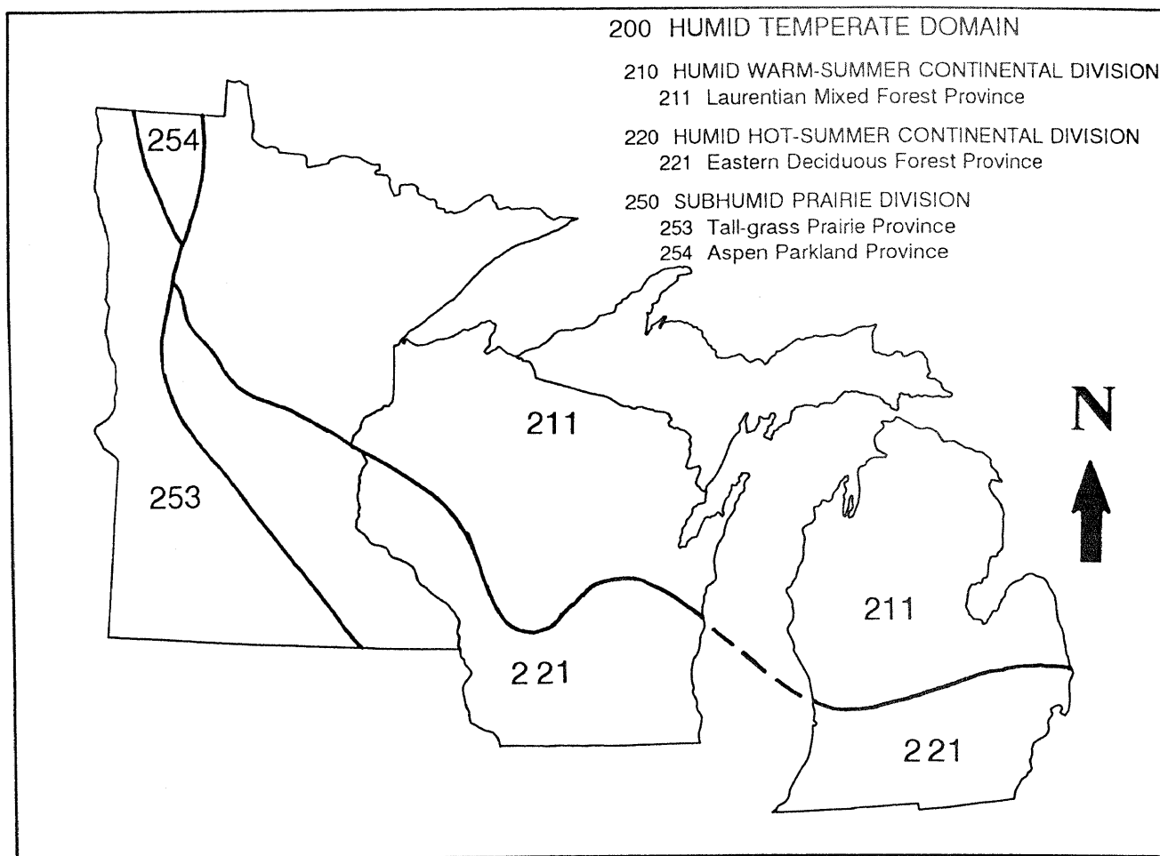
Figure 2.—A portion of Bailey and Cushwa's (1981) map of ecoregions of North America.
