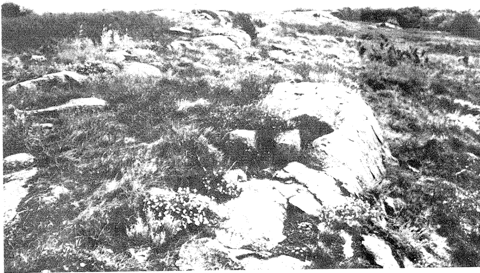
Figure 10.—Subsection II.1: Outcrops of granitic bedrock in the Minnesota River Valley near Ortonville, Minnesota, provide a fire-protected, dry habitat which supports cactus species. Heavy grazing in surrounding prairie has allowed exotic grasses to become the dominant vegetation. Minnesota Department of Natural Resources photo by R. Dana.
