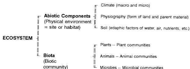
Figure 1.— Diagrammatic illustration of the biotic and abiotic components of the landscape ecosystem. The dynamic interactions among components are not shown. (Courtesy of B.V. Barnes.)
