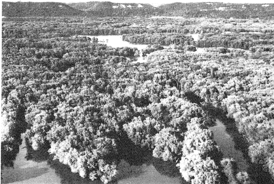
Figure 17.—Sub-subsection IV.3.3: Extensive flood plain forest occupies the broad flood plain of the Mississippi River in the foreground. The highly dissected slopes of the Driftless Area (Paleozoic Plateau) are in the background. Minnesota Department of Natural Resources photo by H. Dunevitz.
