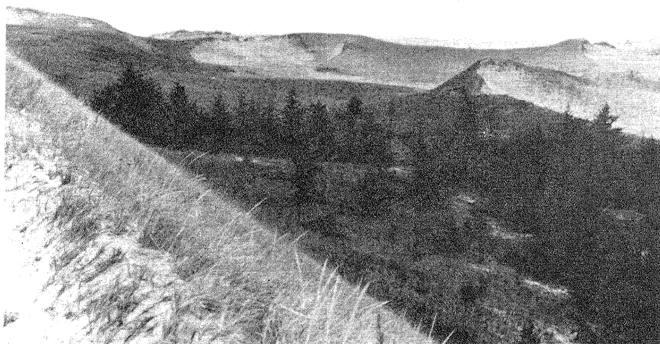
Figure 21.—Subsection VII.4: Steep sand dunes, as high as 600 feet, form a narrow band along much of the Lake Michigan shoreline. These dunes, which date from the low-water Nipissing Stage of the Great Lakes from approximately 4,000 years ago, also occur along the shoreline of Lake Michigan and eastern Lake Superior in other subsections and sub-subsections. Near the shoreline, large areas of the dunes have open, shifting sands, but farther inland, where there is protection from offshore winds, forests stabilize the dune sands. Photo by D. Albert.
