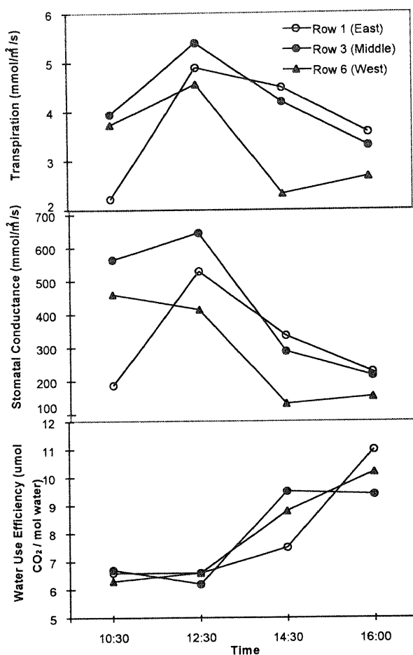
Figure 4.—Diurnal pattern of transpiration, stomatal conductance, and water use efficiency in different corn rows.
