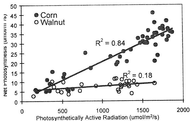
Figure 3.—Photosynthesis in corn and black walnut as related to PAR.
