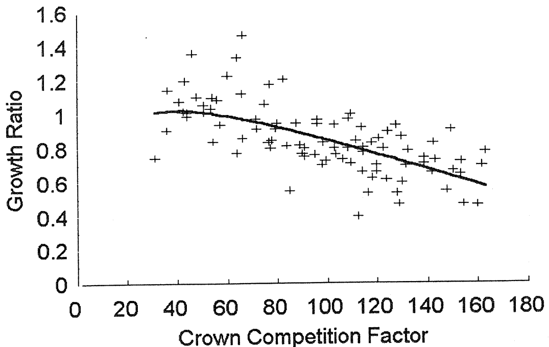
Figure 1.—Relation between normalized growth and degree of crowding.
