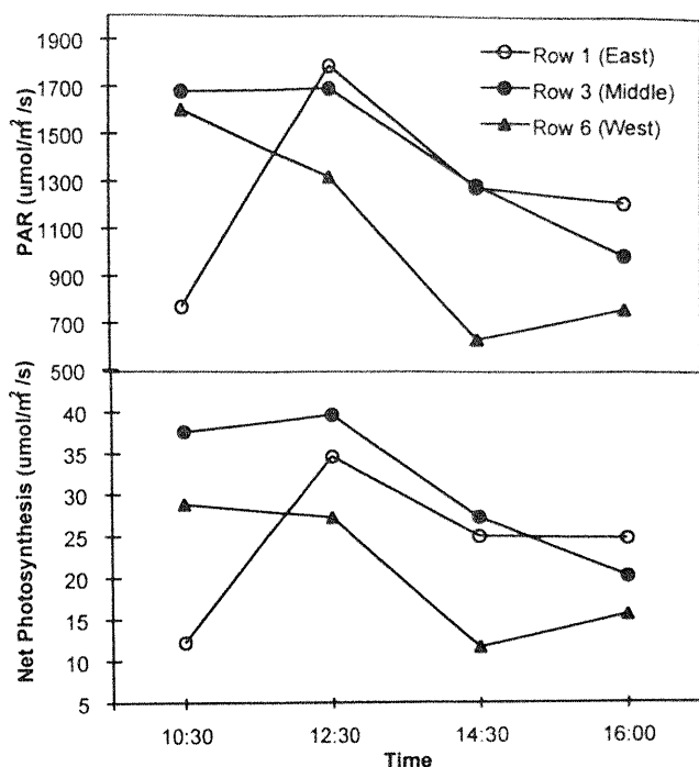
Figure 2.—Diurnal pattern of incident PAR and net photosynthesis in different corn rows.
