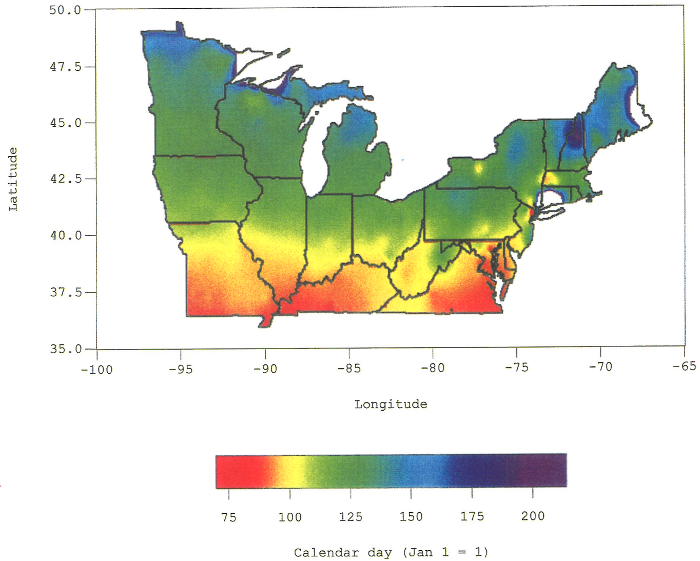
Average calendar day of freezes after 200 GDD (base 5 C)
