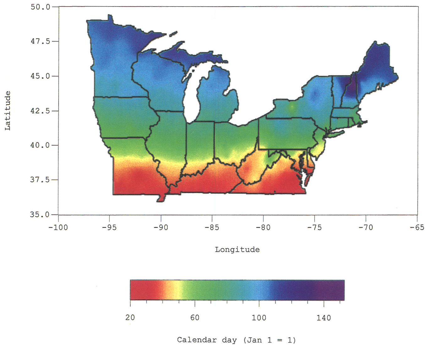
Average calendar day for reaching 50 GDD (base 5 C)
