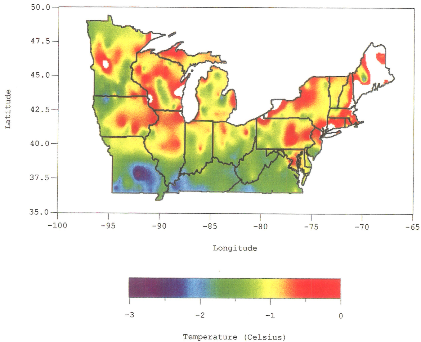
Average temperature of freezes after 300 GDD (base 5 C)
