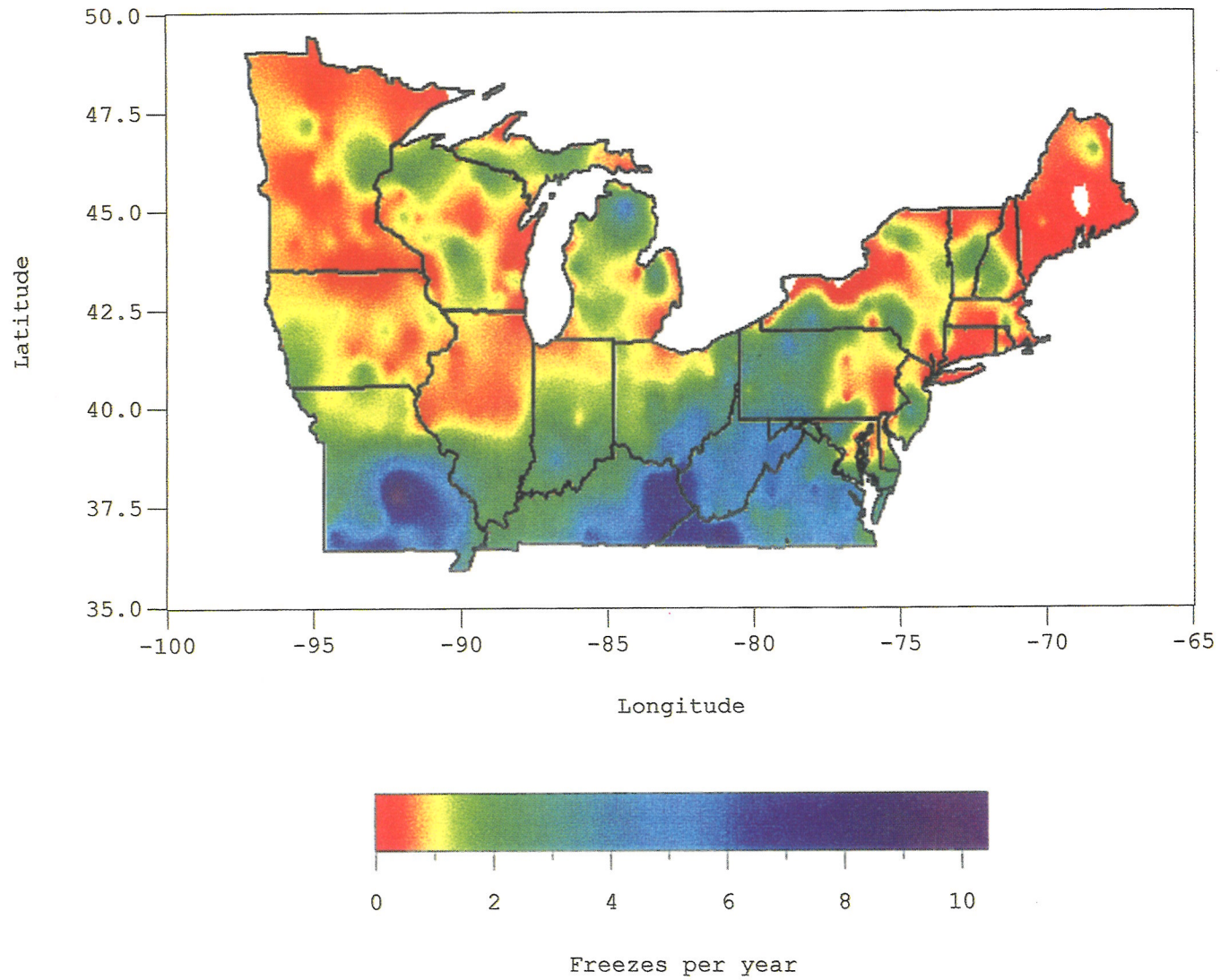
Average number of freezes following 250 GDD (base 5 C)
