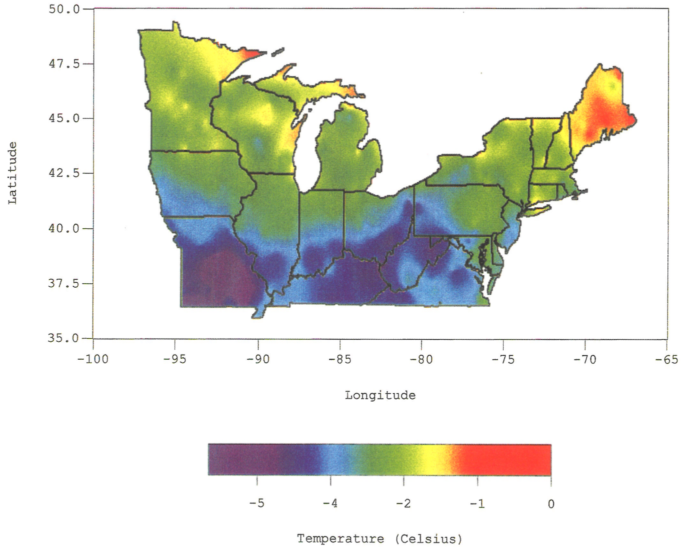
Average temperature of freezes after 50 GDD (base 5 C)
