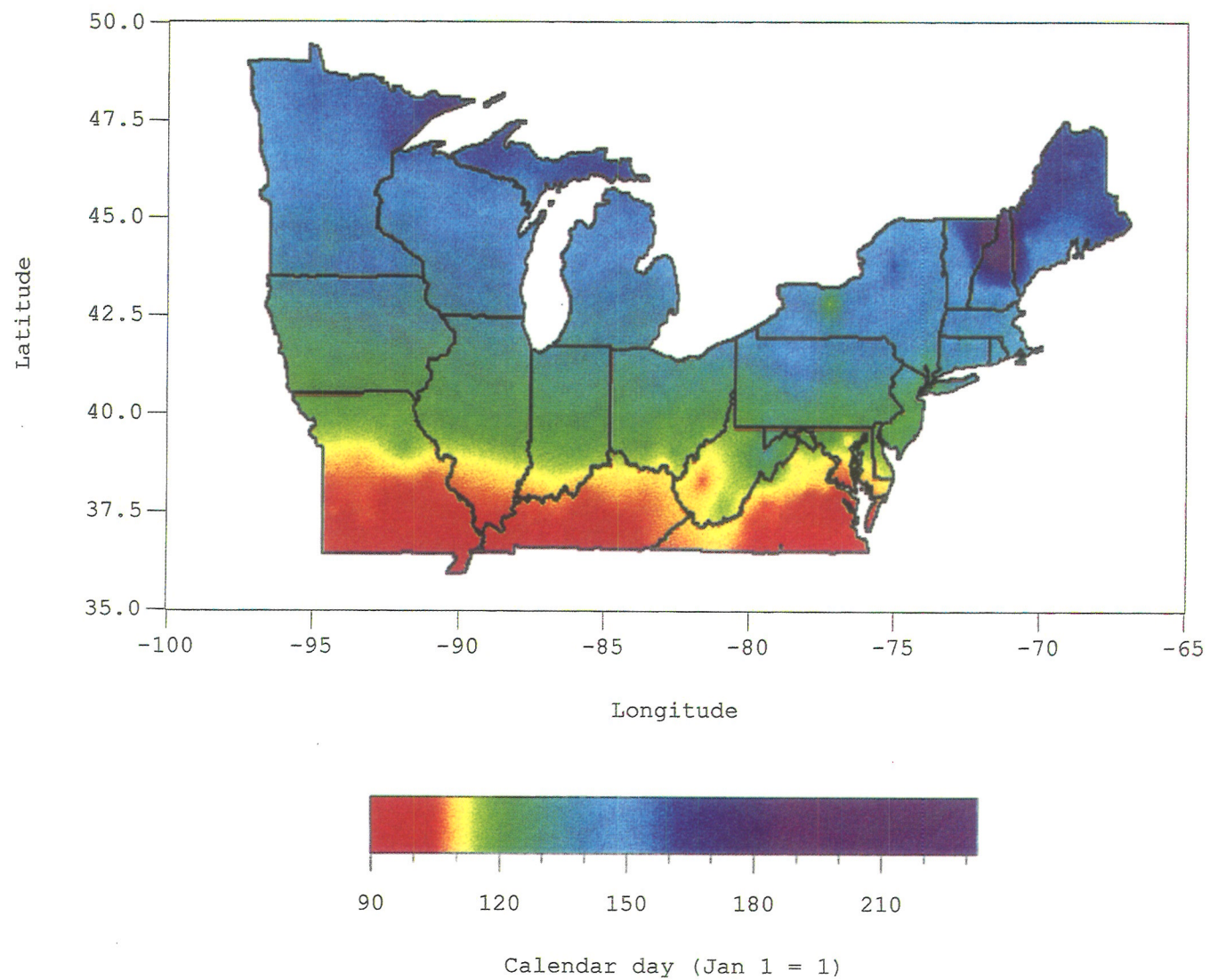
Average calendar day for reaching 350 GDD (base 5 C)
