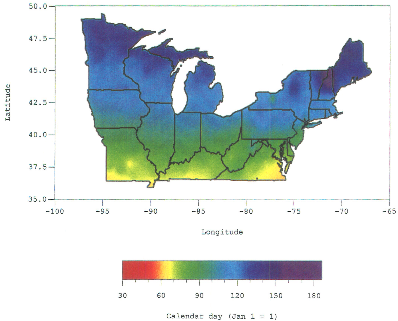
Average calendar day for reaching 150 GDD (base 5 C)
