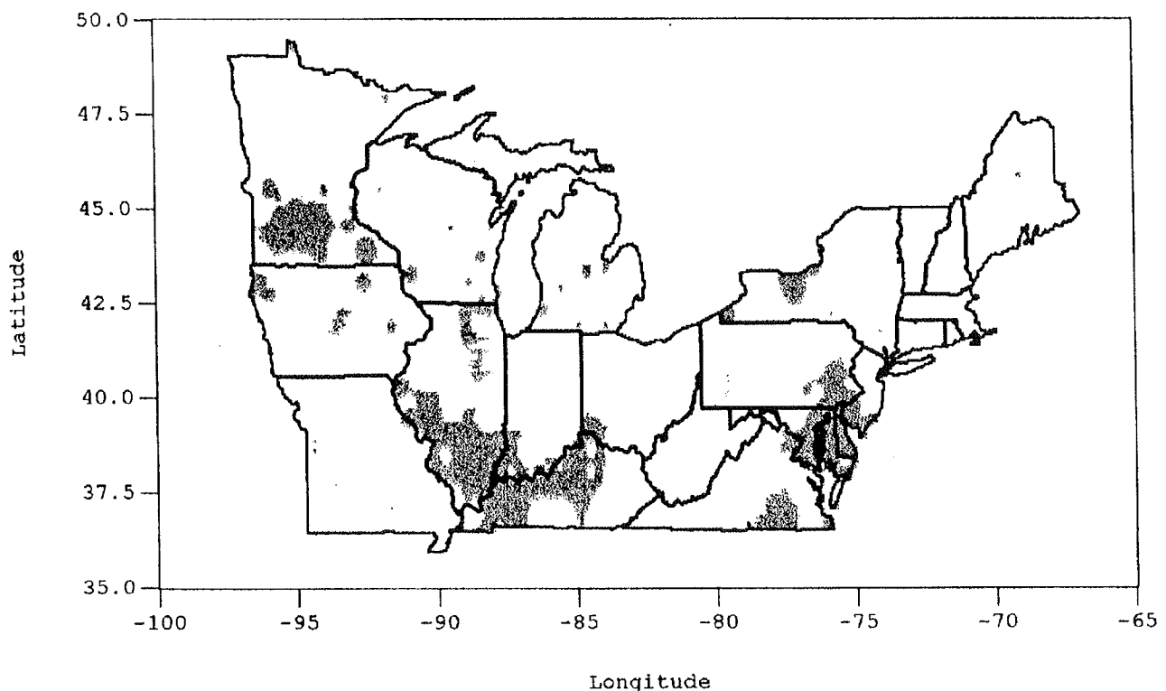
Figure 2.—Regions where average day of freeze occurrence following 200 growing degree days precedes average day for attaining 200 growing degree days, shaded.
