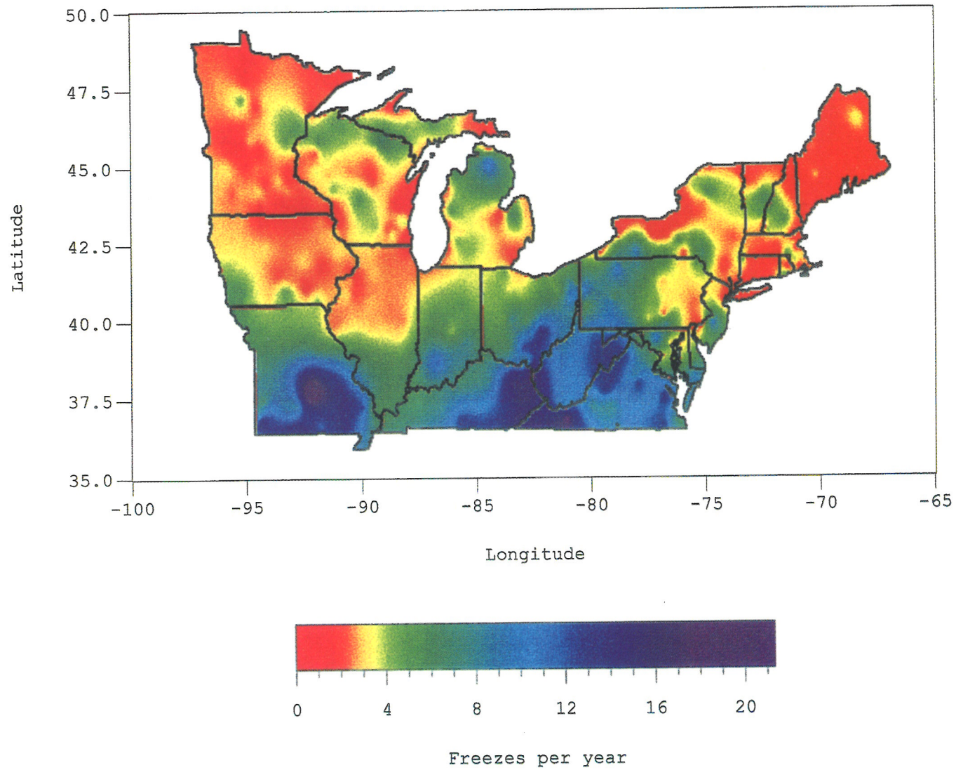
Average number of freezes following 150 GDD (base 5 C)
