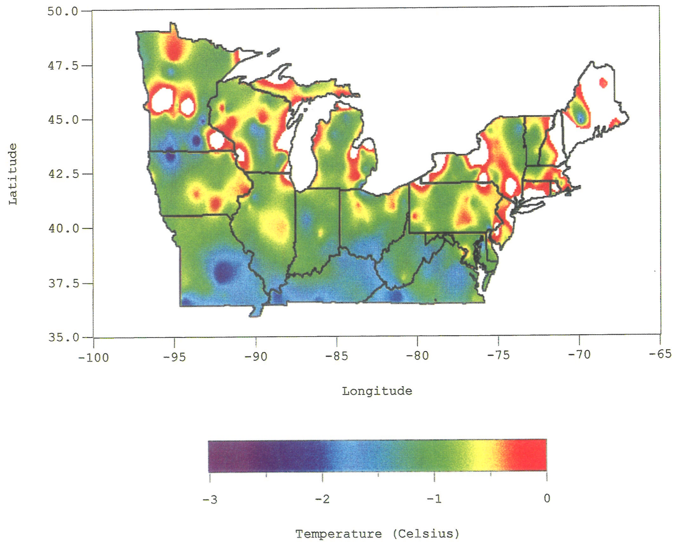
Average temperature of freezes after 350 GDD (base 5 C)
