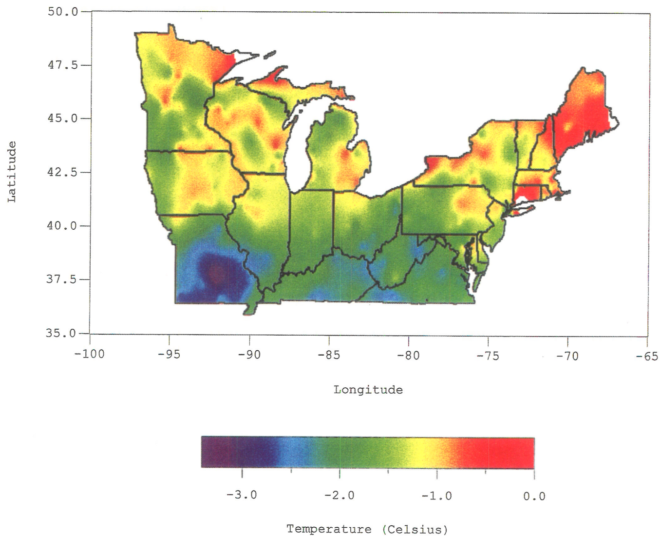
Average temperature of freezes after 200 GDD (base 5 C)
