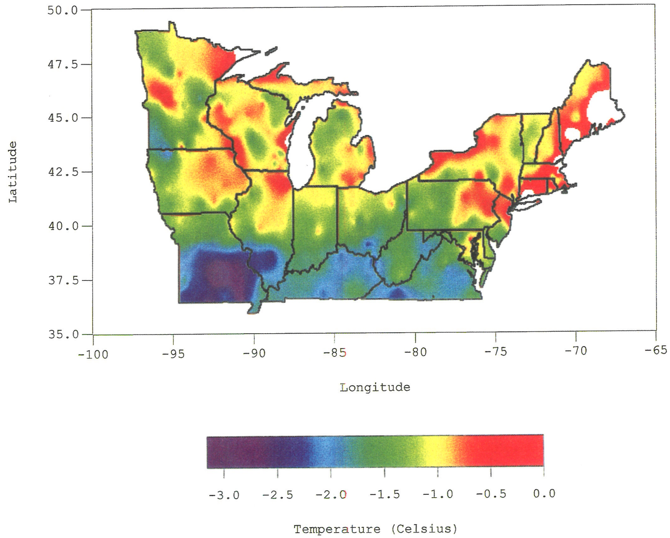
Average temperature of freezes after 250 GDD (base 5 C)
