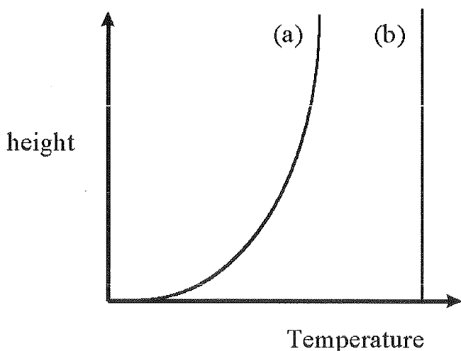
Figure 1.—Typical temperature profiles for (a) radiation-driven freeze and (b) air-mass freeze.
