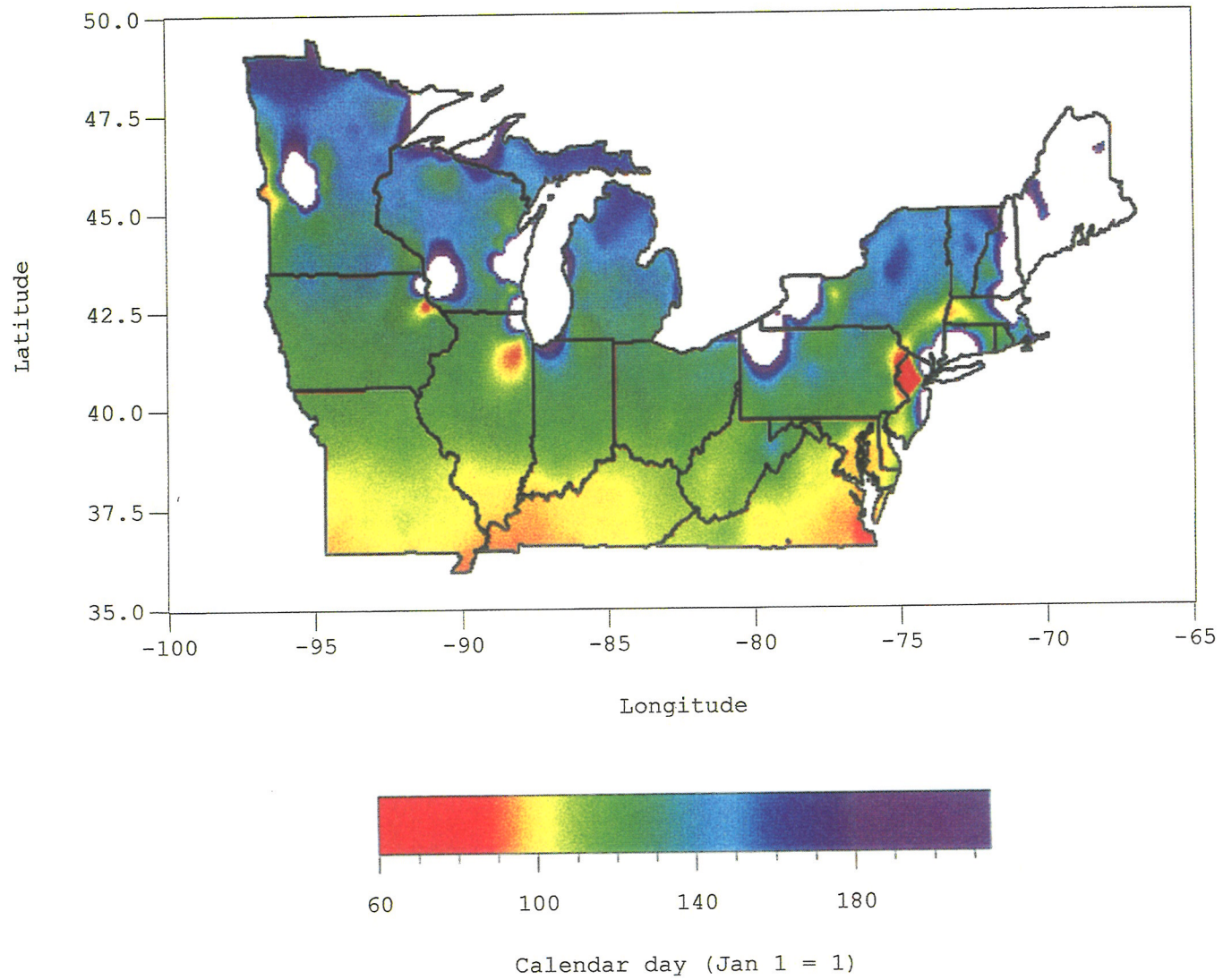
Average calendar day of freezes after 300 GDD (base 5 C)
