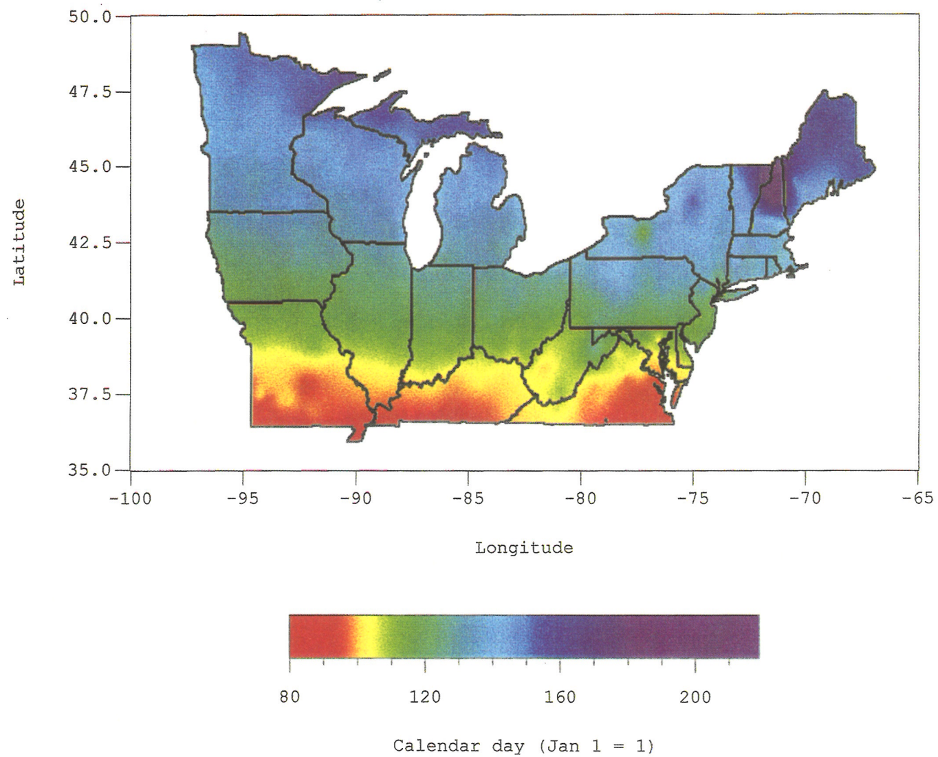
Average calendar day for reaching 300 GDD (base 5 C)
