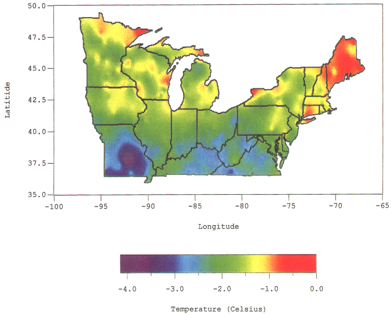
Average temperature of freezes after 150 GDD (base 5 C)
