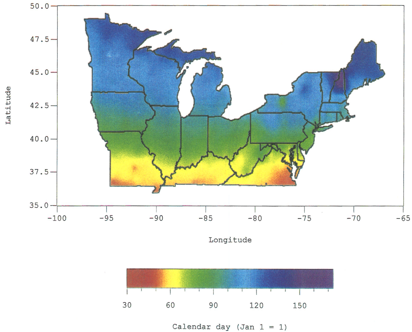
Average calendar day for reaching 100 GDD (base 5 C)
