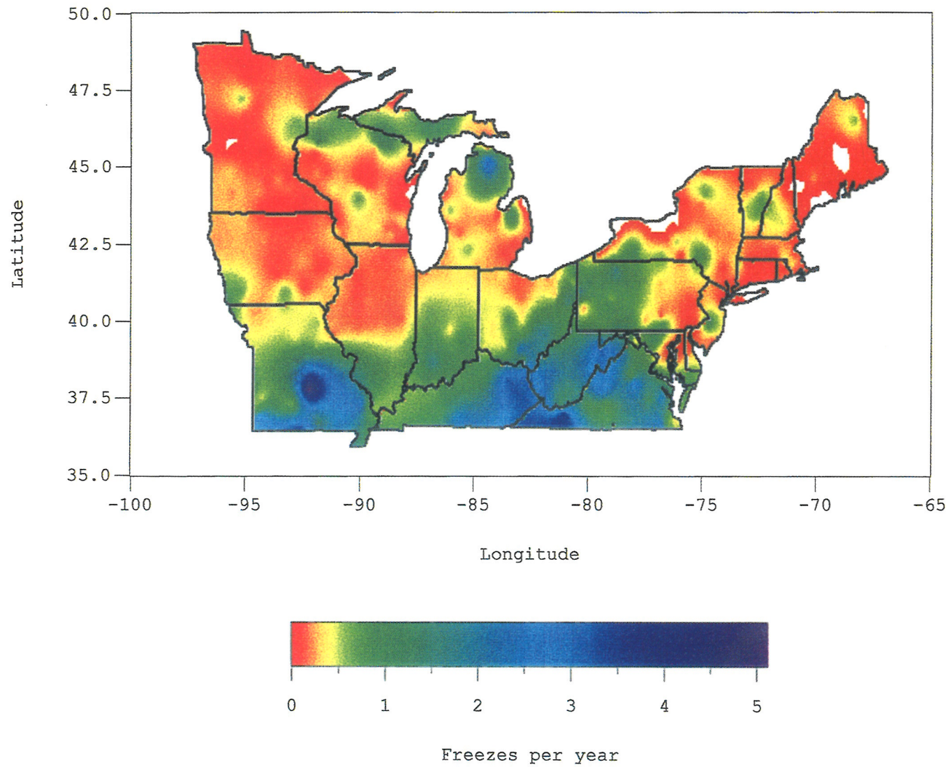
Average number of freezes following 350 GDD (base 5 C)
