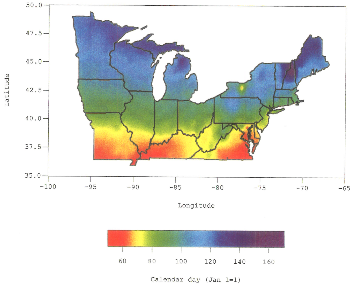
Average calendar day of freezes after 50 GDD (base 5 C)
