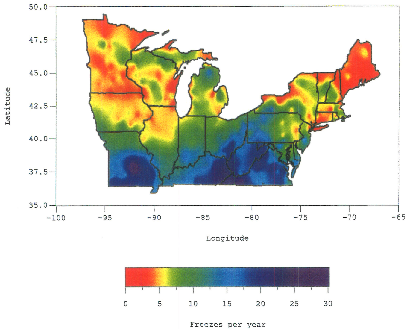
Average number of freezes folloowing 100 GDD (base 5 C)
