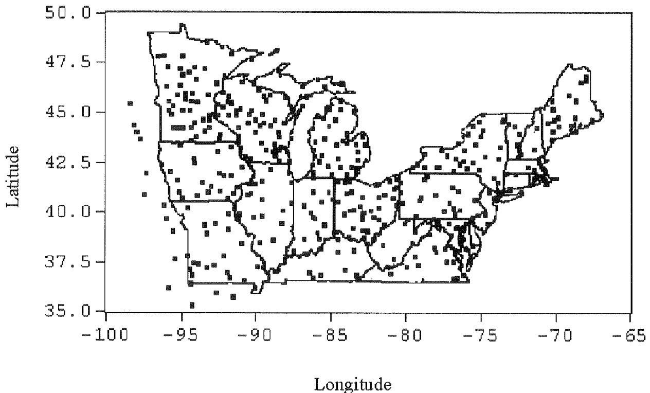
Figure A1.—Locations of stations used to produce the maps in this study.
