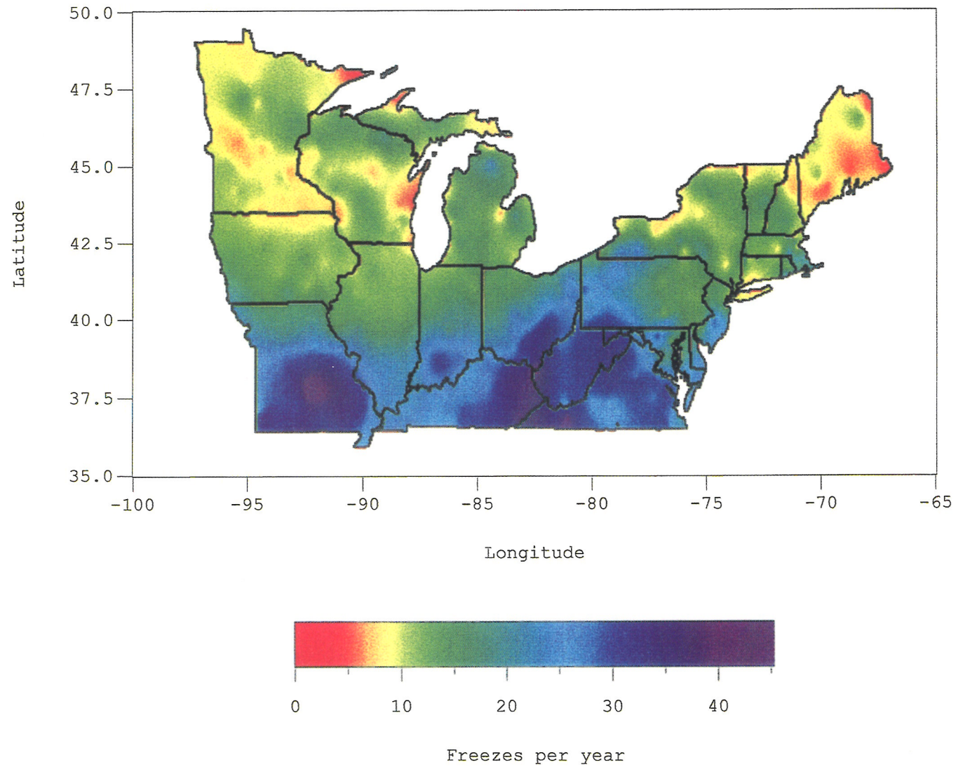
Average number of freezes following 50 GDD (base 5 C)
