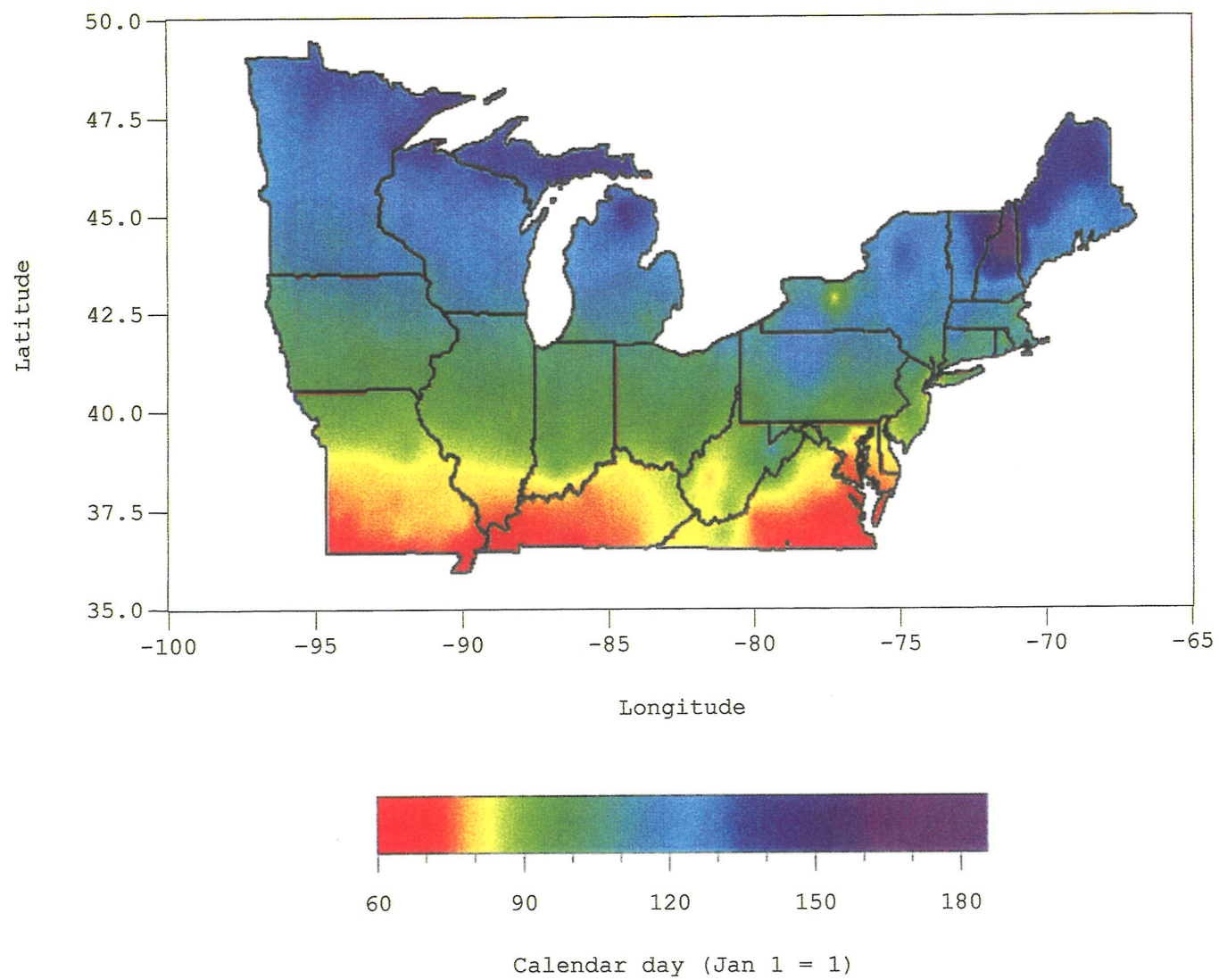
Average calendar day of freezes after 100 GDD (base 5 C)
