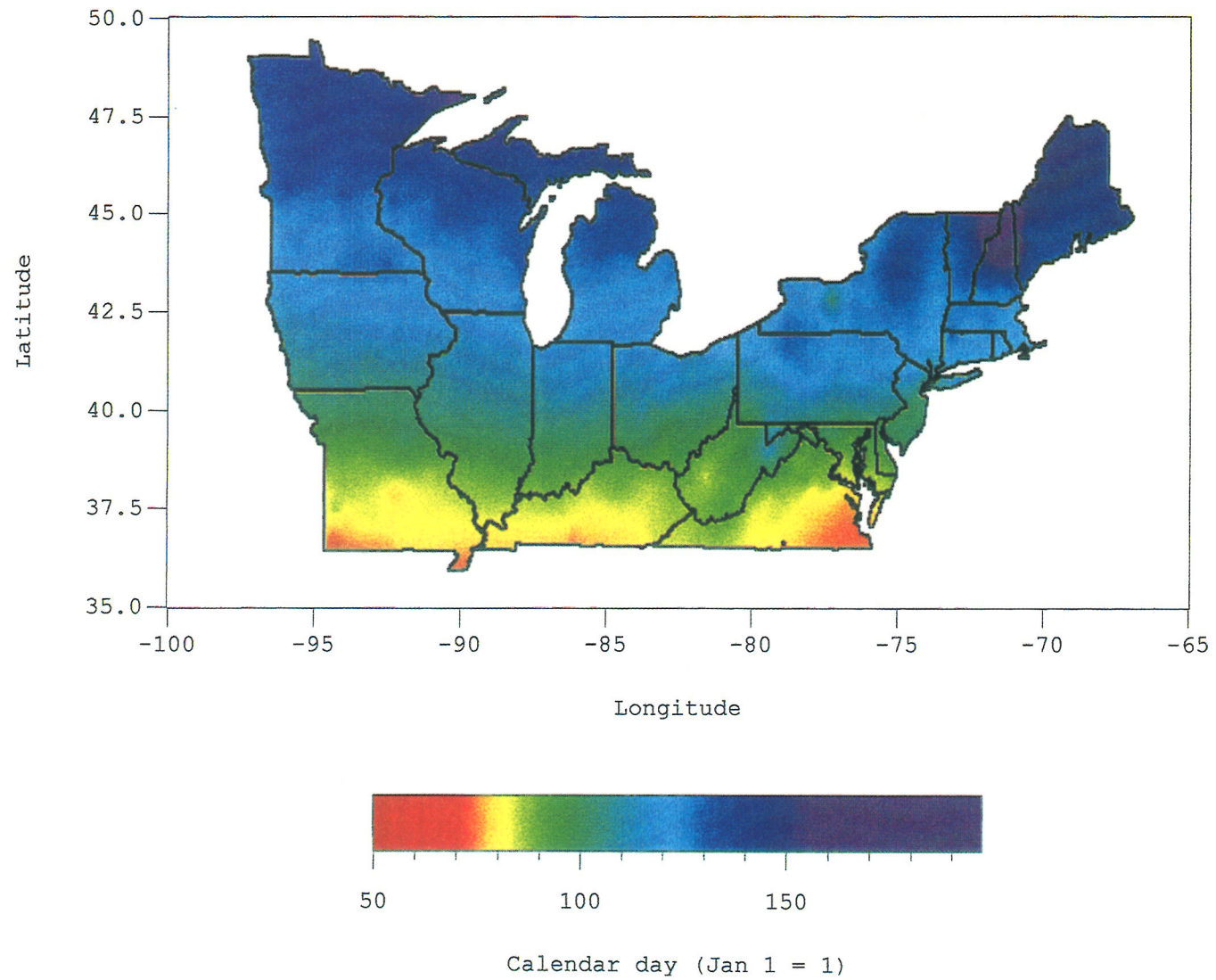
Average calendar day for reaching 200 GDD (base 5 C)
