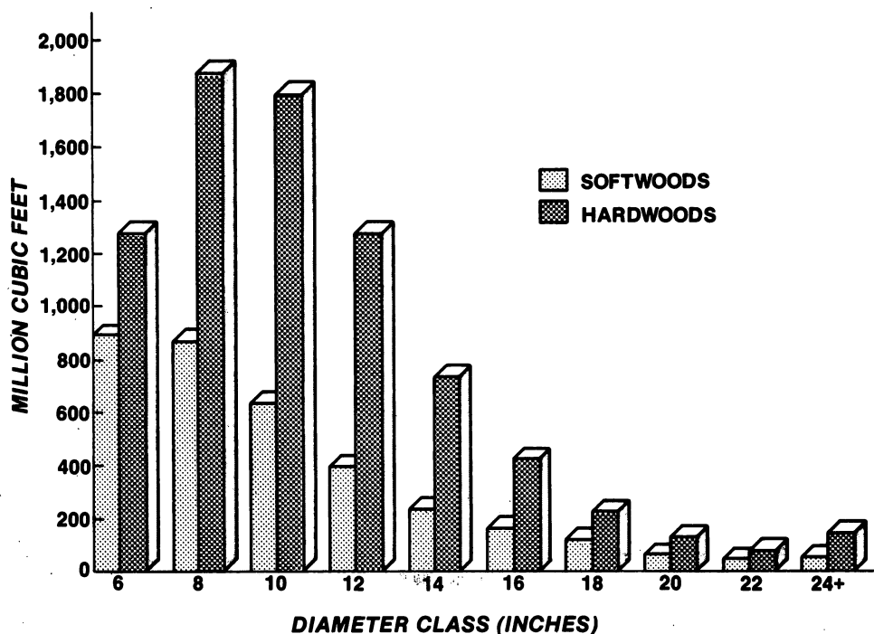
Figure 4.—Net volume of growing stock on commercial forest land by softwoods and hardwoods and diameter class, Minnesota, 1977.
