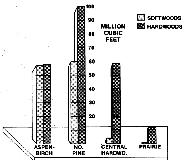
Figure 7. — Net annual growth of growing stock on commercial forest land by softwoods and hardwoods and Forest Survey Unit, Minnesota, 1976.
