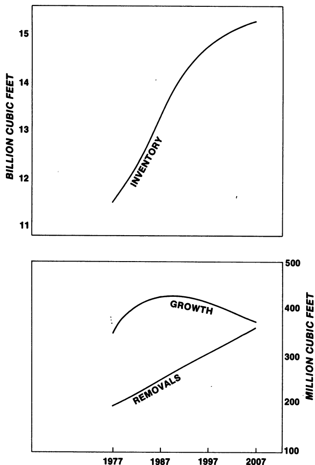
Figure 10.—Removals, net growth, and inventory of growing stock in Minnesota, 1977, and low removals option projection for 1977-2007.
