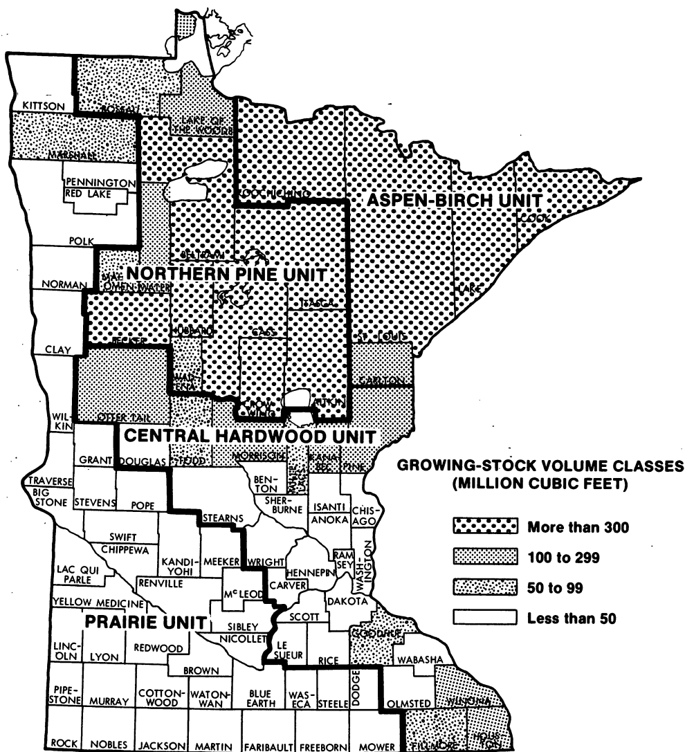
Figure 2.—Growing-stock volume in Minnesota counties, 1977.
