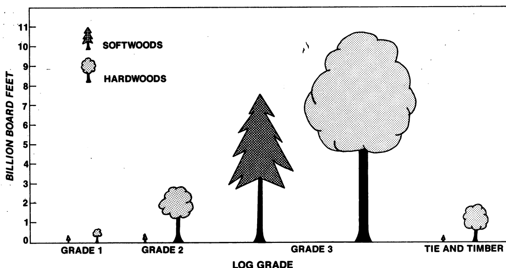
Figure 6.—Net volume of sawtimber on commercial forest land by log grade and softwoods and hardwoods, Minnesota, 1977.
