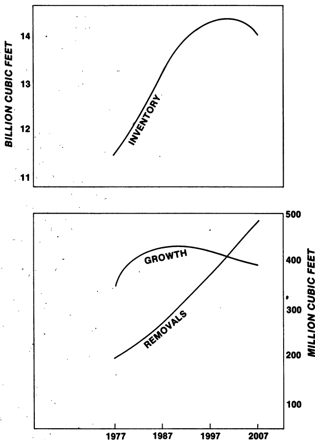
Figure 11.— Removals, net growth, and inventory of growing stock in Minnesota, 1977, and high removals option projection for 1977-2007.
