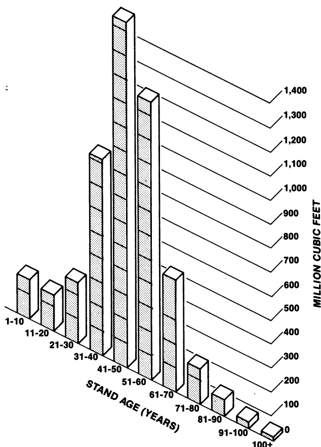
Figure 5.— Net volume of growing stock in the aspen forest type on commercial forest land by stand-age class, Minnesota, 1977.
