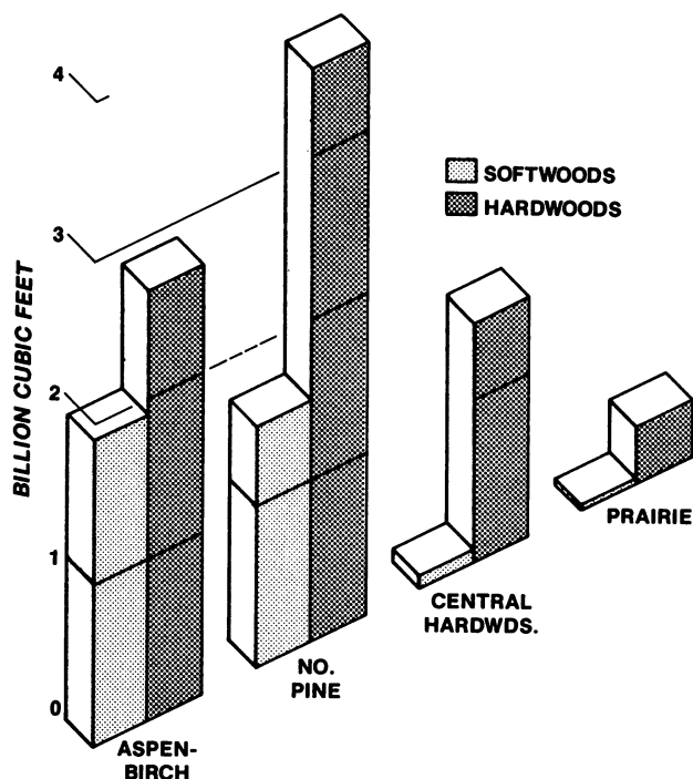
Figure 1.—Net volume of growing stock on commercial forest land by softwoods and hardwoods and Forest Survey Unit, Minnesota, 1977.
