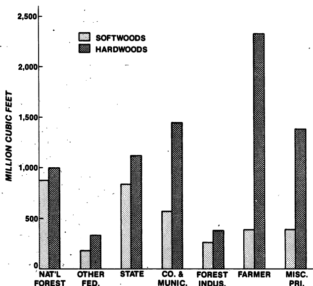
Figure 3.—Net volume of growing stock on commercial forest land by softwoods and hardwoods and ownership class, Minnesota, 1977.
