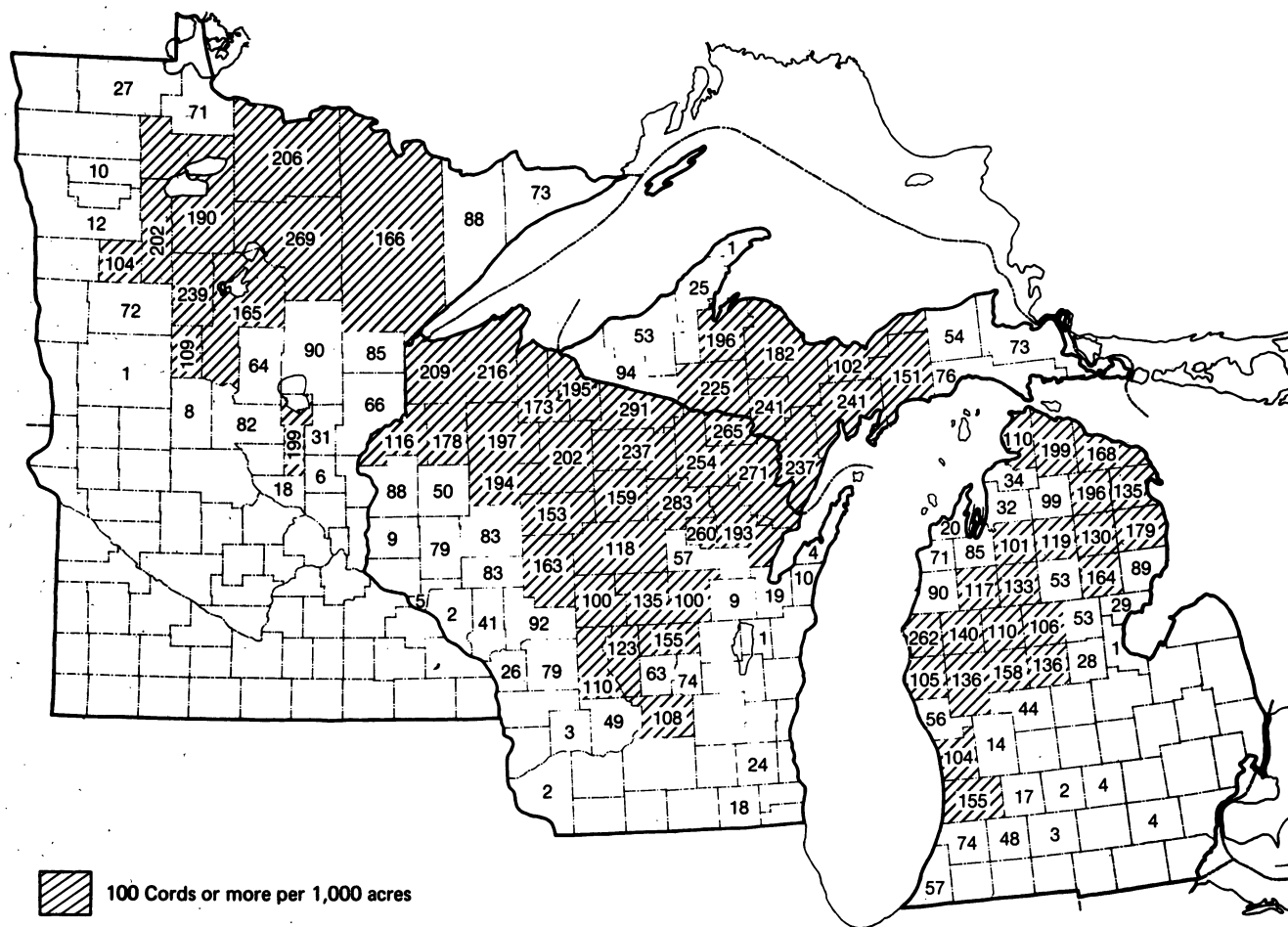
Figure 2.--Cords of pulpwood cut per 1,000 acres of stocked commercial forest land in principal pulpwood-producing counties, 1983. Acres of stocked commercial forest land were determined during the last forest inventory in each State.
