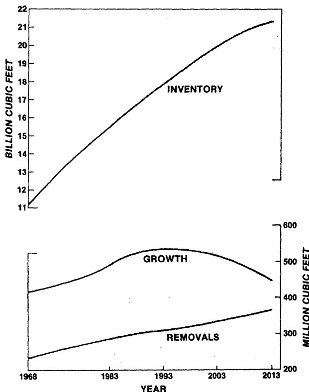
Figure 7. — Removals, net growth, and inventory of growing stock in Wisconsin, 1968-1983, and low removals option projection for 1984-2013.
