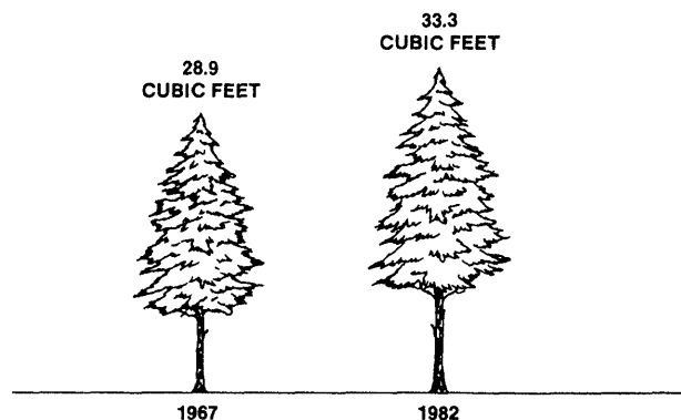
Figure 6. — Average net annual growth per acre of growing stock on timberland, Wisconsin, 1967 and 1982.
