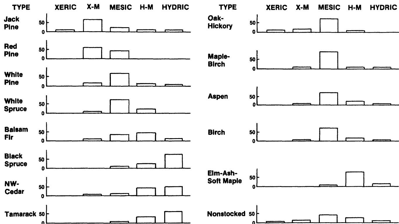
Figure 15. — Distribution of timberland (in percent) by forest type and physiographic class, Wisconsin, 1983.
