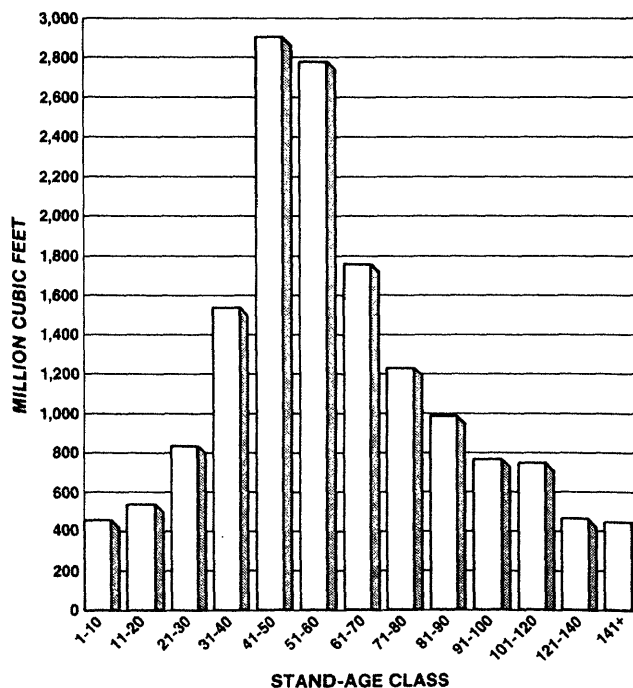
Figure 4. — Net volume of growing stock on timberland by stand-age class, Wisconsin, 1983.
