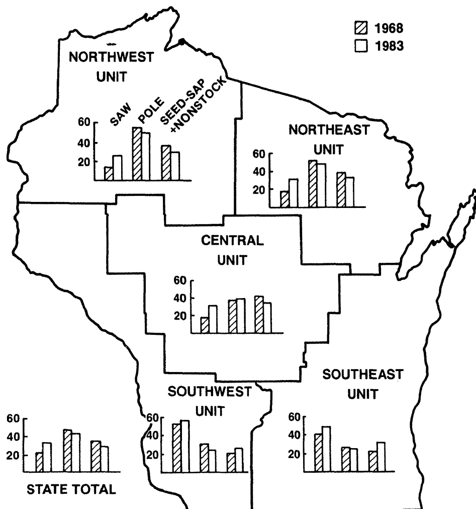
Figure 14. — Distribution of timberland (in percent) by Survey Unit, survey year, and stand-size class.
