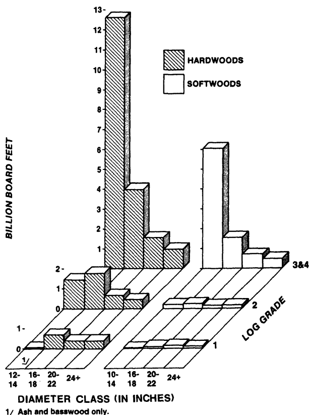
Figure 5. — Net volume of sawtimber on timberland by log grade, diameter class of sawtimber tree, and softwoods and hardwoods, Wisconsin, 1983.
