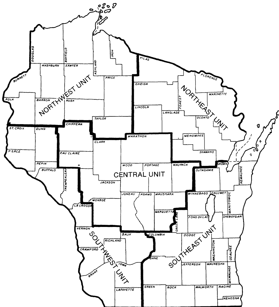
Figure 1. — Wisconsin Survey Units.
