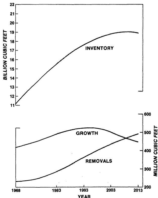
Figure 8. — Removals, net growth, and inventory of growing stock in Wisconsin, 1968-1983, and high removals option projection for 1984-2013.
