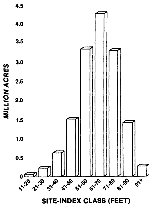
Figure 16. — Area of timberland by site-index class, Wisconsin, 1983.
