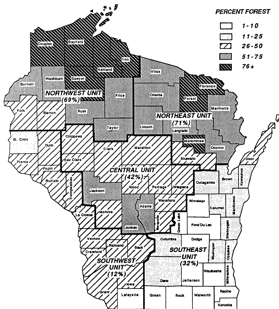
Figure 12. — Wisconsin Forest Survey Units and percent forest cover by county, 1983.
