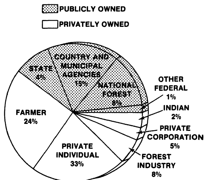
Figure 13. — Area of timberland by ownership class, Wisconsin, 1983.
