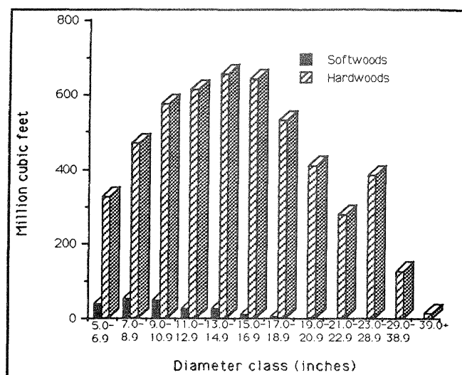
Figure 13.— Volume of growing stock on timberland by softwoods and hardwoods, and diameter class, Indiana, 1986.
