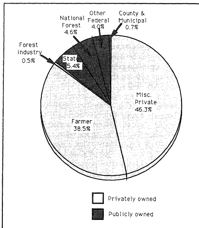
Figure 15.—Percent of growing-stock volume on timberland by owner class, Indiana, 1986.
