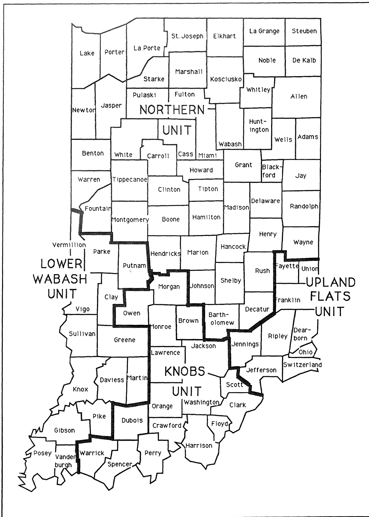
Figure 4.—Location of Forest Survey Units in Indiana.
