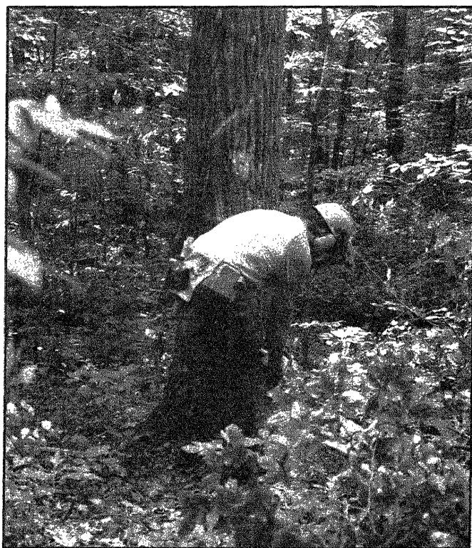
Figure 17.—Sawtimber removals in 1985 were 34 percent higher than in 1966.
