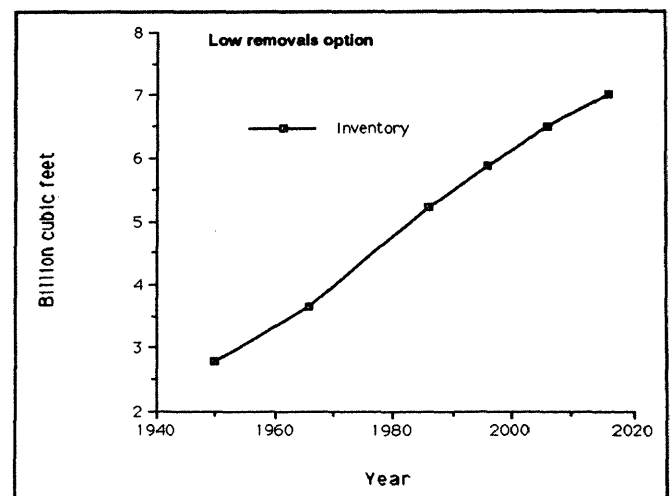
Figure 18.—Removals, net growth, and inventory of growing stock in Indiana, 1950-1986, and low removals projection for 1987-2016.
