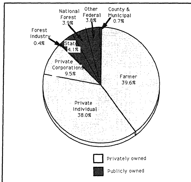
Figure 8.—Area of timberland by ownership class, Indiana, 1986.
