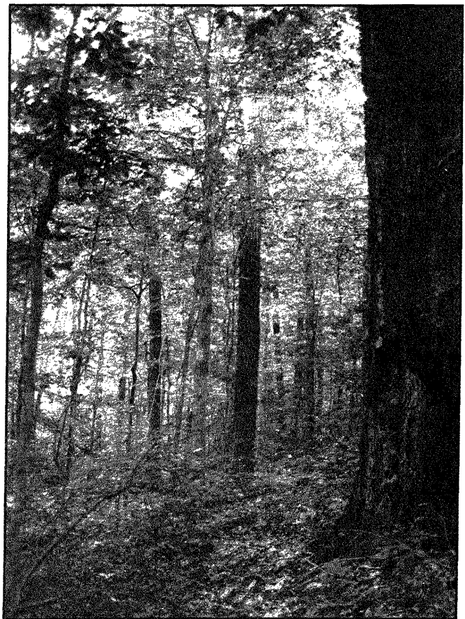
Figure 1.—The area of timberland in the State increased an average of 21,000 acres per year between 1967 and 1986.
