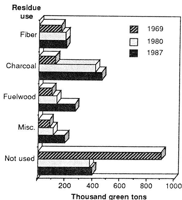
Figure 6.—Disposition of mill residues by major use in Missouri, 1969, 1980, and 1987.
