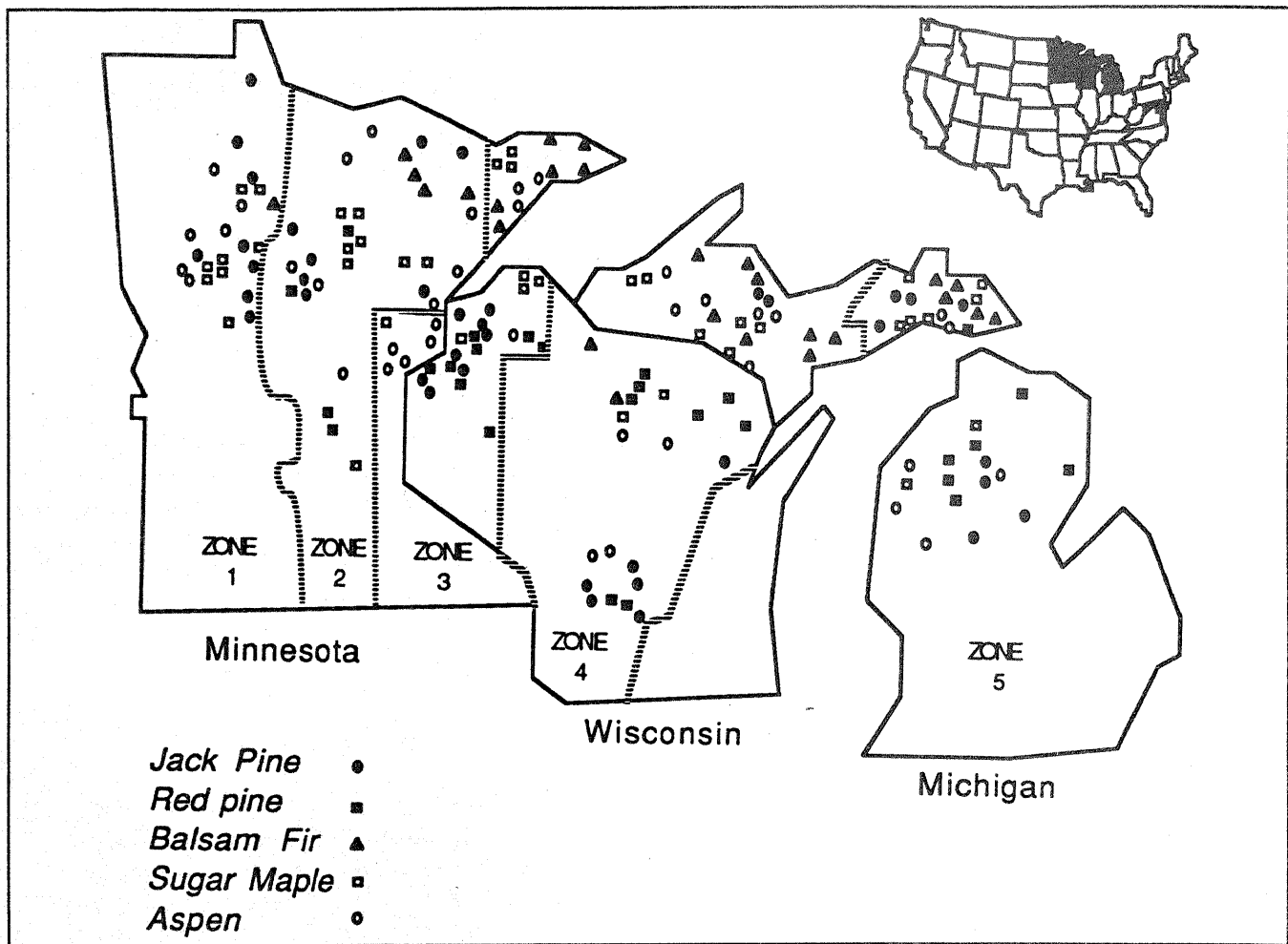
Figure 1.—Distribution of plots sampled along an acid sulfate deposition gradient across the Lake States.
