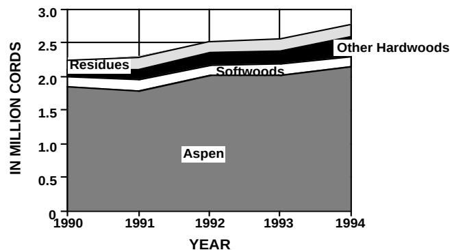
Figure 15.—Pulpwood production for particleboard in the Lake States, 1990-1994.
