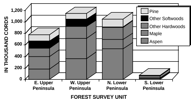
Figure 6.—Michigan roundwood pulpwood production by Forest Survey Unit and species groups, 1994.
