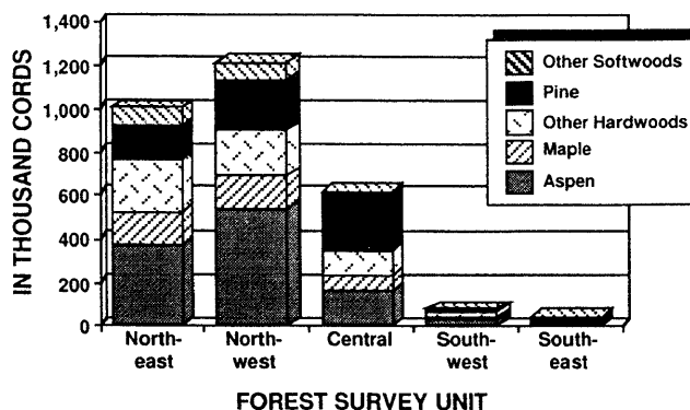
Figure 10.—Wisconsin roundwood pulpwood production by Forest Survey Unit and species group, 1996.
