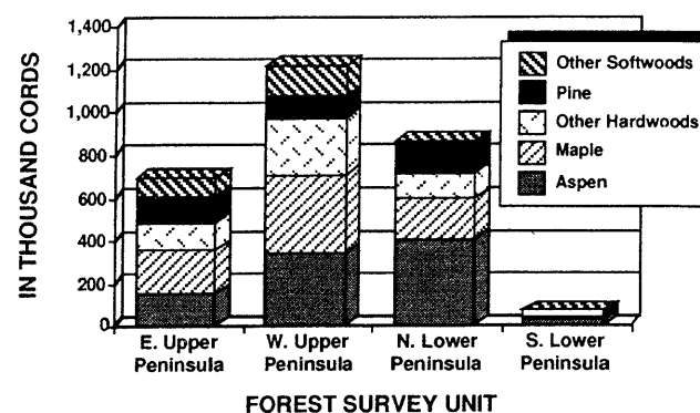
Figure 6.—Michigan roundwood pulpwood production by Forest Survey Unit and species groups, 1996.
