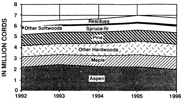
Figure 14.—Pulpwood production in the Lake States for pulp by species group and residues, 1992-1996.
