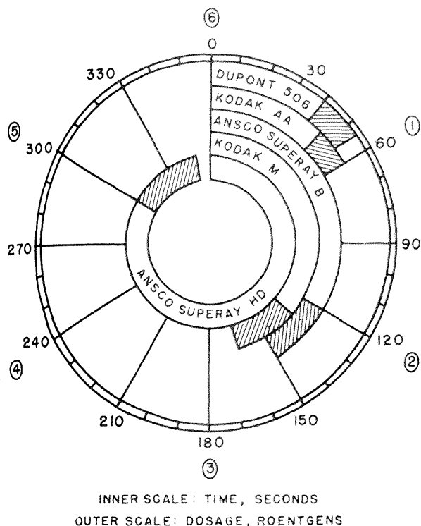
FIGURE 5. — Optimum exposure times for high definition in white pine seed radiographs, with dosage levels, using various films at 15 kvp, 3 ma and 28 inches focus-film distance (GE CSI-25 tube, 2 mm. focal spot, 0.030 beryllium filtration).
