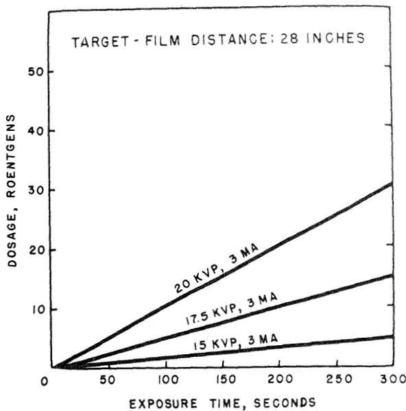
FIGURE 2. — The relationship of radiation intensity at the film plane to exposure time and kvp, at 3 ma and 28 inches target-film distance (GE CSI-25 tube, 2 mm. focal spot, 0.030 beryllium filtration).
