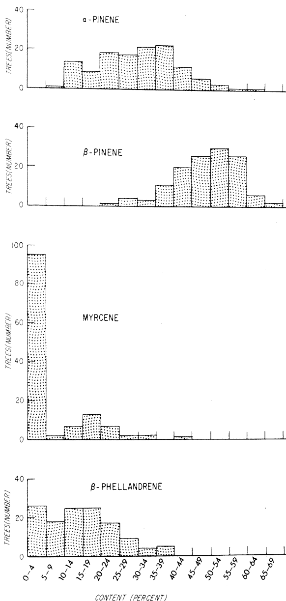
FIGURE 1. — Frequency distributions for the major constituents of turpentine in cortex gum. Basis, 129 trees.
