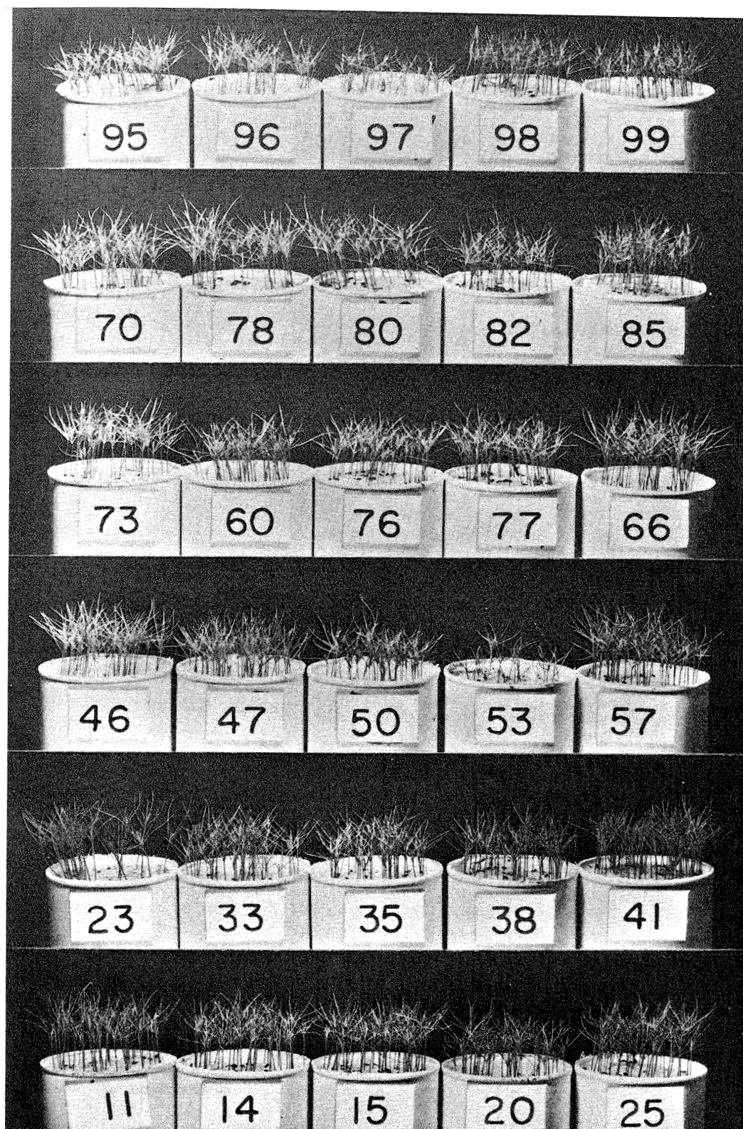
FIGURE 2. — Jack pine germinants of 30 provenances ranging from East (bottom) to West (top).
