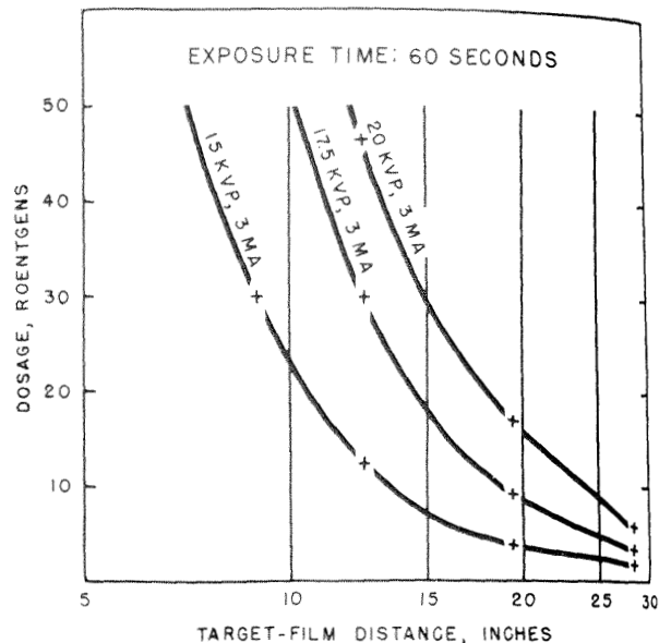
FIGURE 3. — The relationship of radiation intensity at the film plane to target film distance and kvp, at 3 ma with a 60-second exposure (GE CSI-25 tube, 2 mm. focal spot, 0.030 beryllium filtration).
