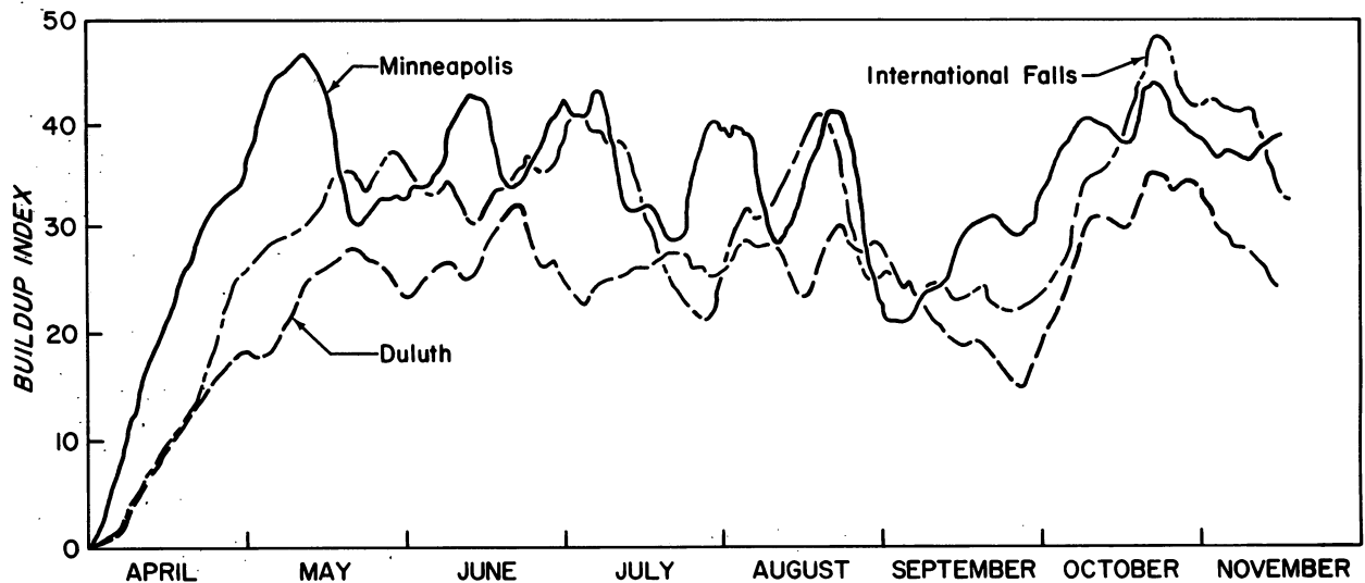
FIGURE 3. — Buildup Index trend over the season for Minneapolis, Duluth, and International Falls.
