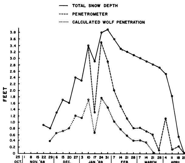
Figure 3.—Snow depth and penetrability by deer and wolves near Isabella, Minnesota, 1968-69.
