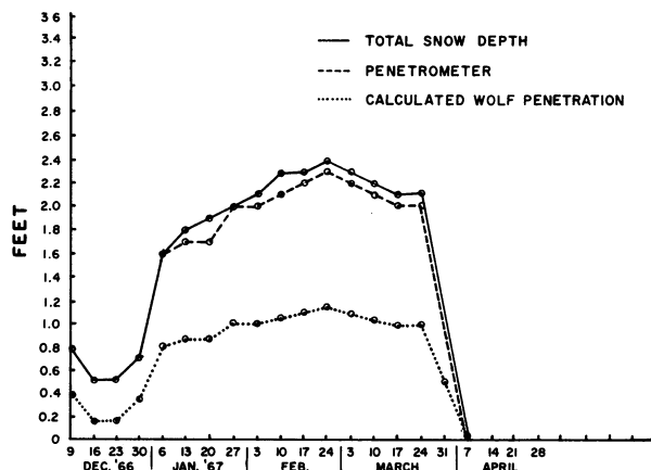
Figure 1.—Snow depth and penetrability by deer and wolves near Isabella, Minnesota, 1966-67.
