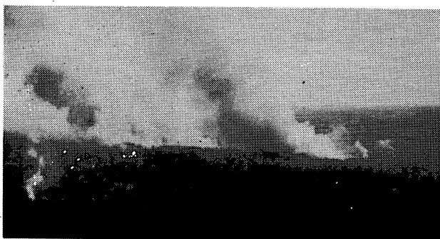
Figure 5.— Spotting well in advance of the main flame front.
