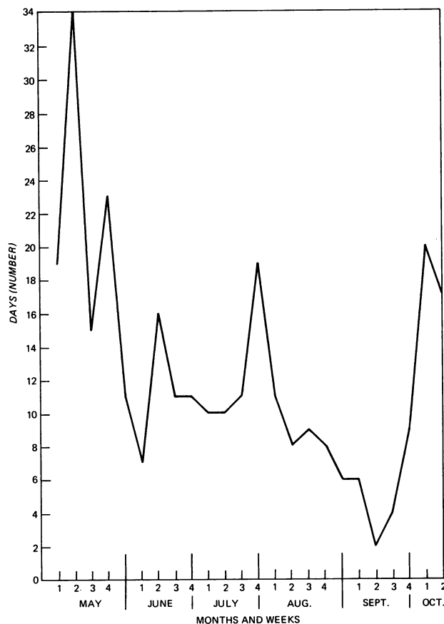
Figure 1.—Frequency of occurrence of class four, fire-danger (very high) days at Ely, Minnesota, during 1936-70, grouped by weeks.
