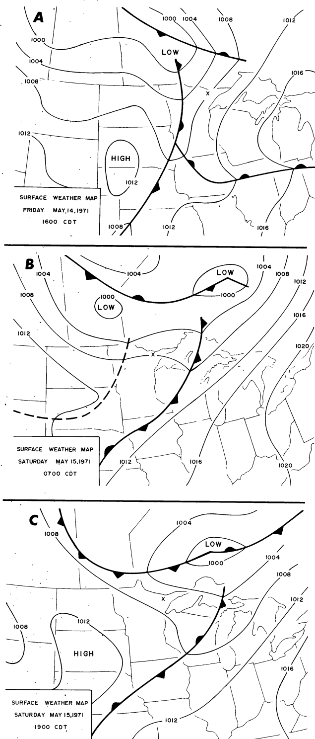
Figure 3. — Surface weather features occurring (A) during the period of initial attack and the first fire run, (B) before the second major fire run, and (C) during the third major fire run. An "X" designates the fire location.
