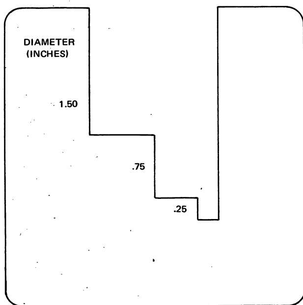
Figure 3. Sheet metal or plastic go-no-go gage may be used to determine fine fuel diameter classes.
