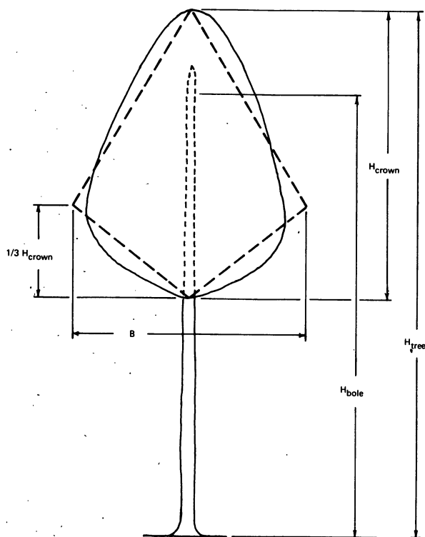
Figure 2.--Mathematical model of a tree with the bole as a truncated cone and the crown as a bicone.
