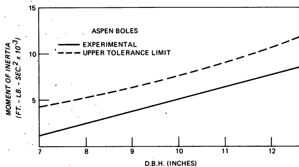
Figure 6.--Moment of inertia prediction equation plus its 95-percent upper tolerance limit for aspen boles obtained from trees in the 70-foot height class.
