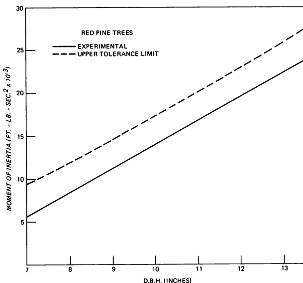
Figure 7.--Moment of inertia prediction equation plus its 95-percent upper tolerance limit for red pine trees in the 70-foot height class.
