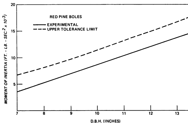
Figure 8.--Moment of inertia prediction equation plus its 95-percent upper tolerance limit for red pine boles obtained from trees in the 70-foot height class.
