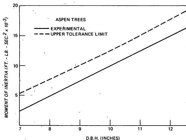
Figure 5.--Moment of inertia prediction equation for aspen trees in the 70-foot height class. The dashed line is the 95-percent upper tolerance limit.
