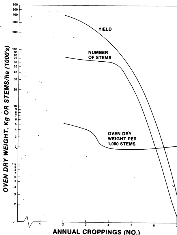
Figure 1.— Regeneration and oven-dry above-ground yield of aspen coppice (except leaves) on successive 1-year croppings. The first cropping was omitted because it was at age 2.
