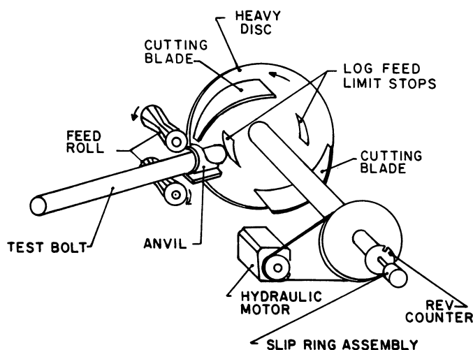
Figure 2. — Simplified illustration of experimental involuted disc chucker.
