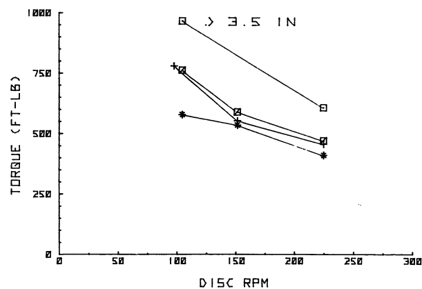
Figure 5. — Torque for large and small diameter logs (left, unfrozen; right, frozen).
