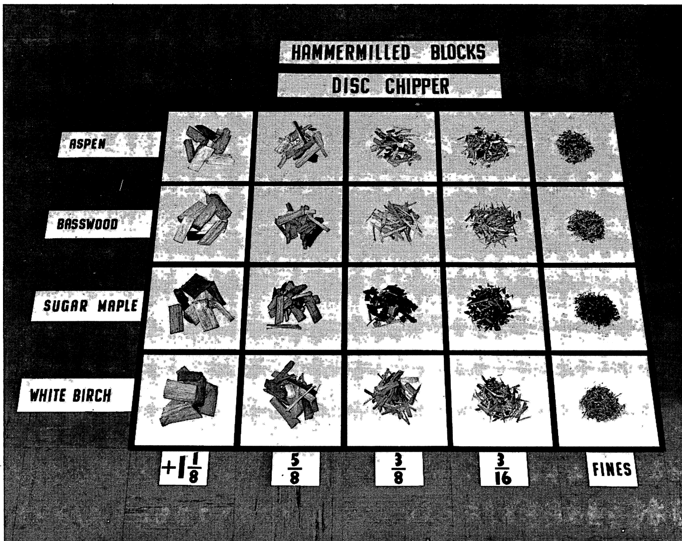
Figure 9. — Sample particles after hammermilling of chunks.
