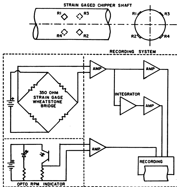
Figure 3. — Schematic of instrumentation system.
