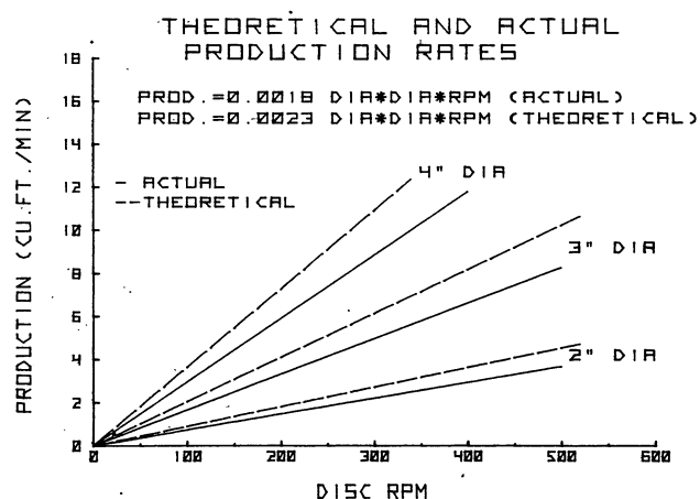
Figure 4. — Comparison of chipping rates with 2- to 4-inch-diameter logs.
