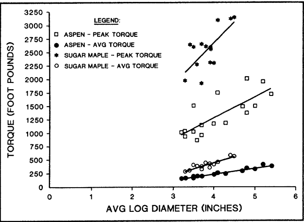
Figure 8.—Test data and the linear regression lines for aspen and sugar maple peak and average torque.
