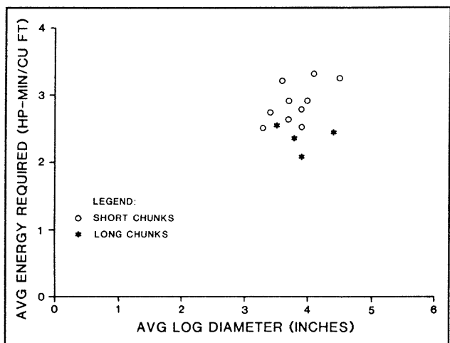
Figure 11.—Average energy required to produce sugar maple short and long chunks.
