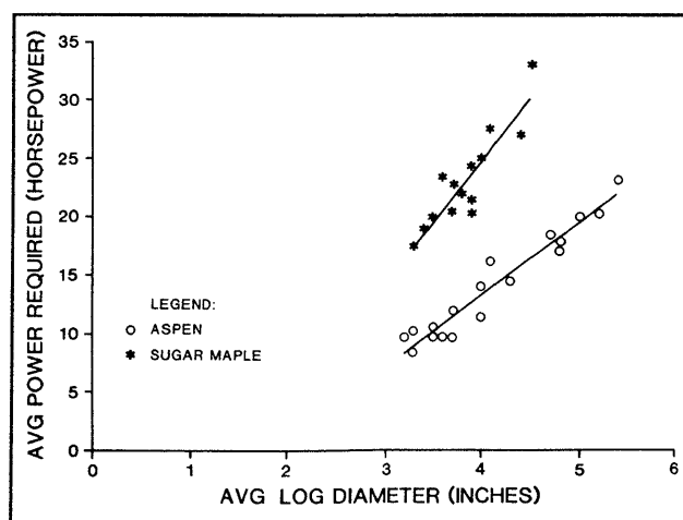
Figure 9.—Test data and the linear regression lines for average power required to produce aspen and sugar maple chunks.
