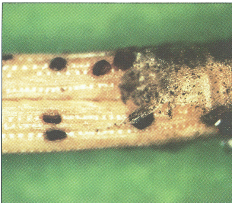
Figure 10.—Fruit bodies of Sirococcus conigenus at base of infected 1-year-old needle.
