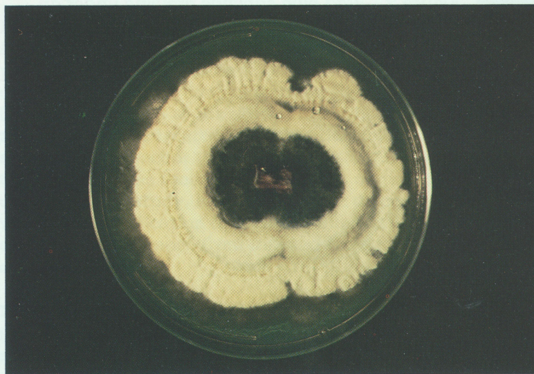
Figure 7.—Culture of Sirococcus conigenus obtained by placing sections of infected shoots on potato-dextrose agar.
