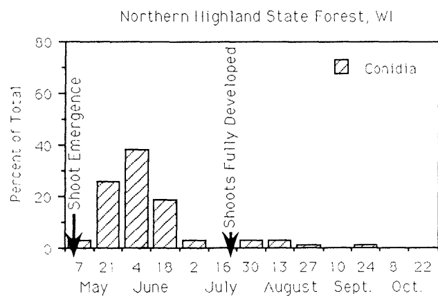
Figure 3.— Sirococcus conigenes conidia dispersal and red pine shoot growth, 1973.
