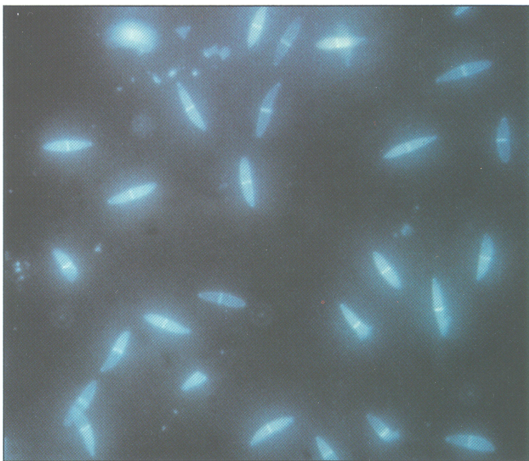
Figure 11.— Two-celled Sirococcus conigenus conidia labeled with a fluorescent brightner and photographed under ultraviolet light (400X).
