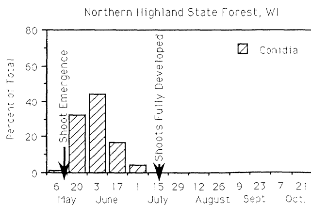
Figure 4.— Sirococcus conigenes conidia dispersal and red pine shoot growth, 1974.
