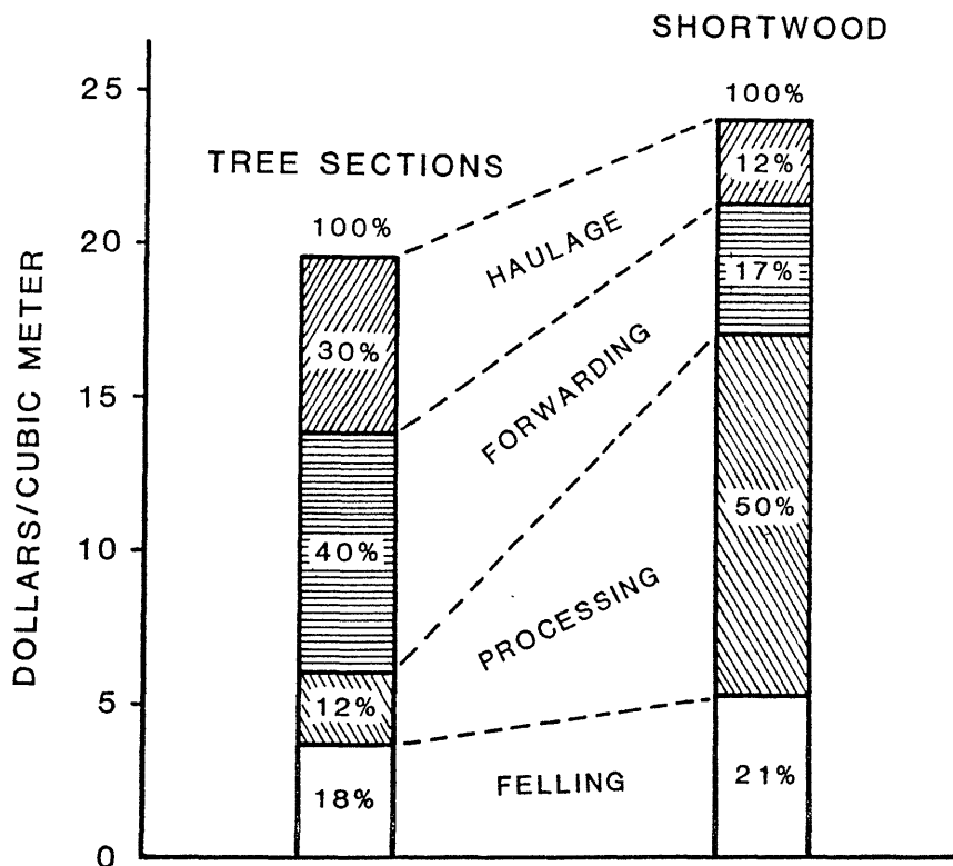
Figure 1.—Cost estimates for tree-section harvesting versus conventional shortwood harvesting in Sweden (from Danielsson 1983).
