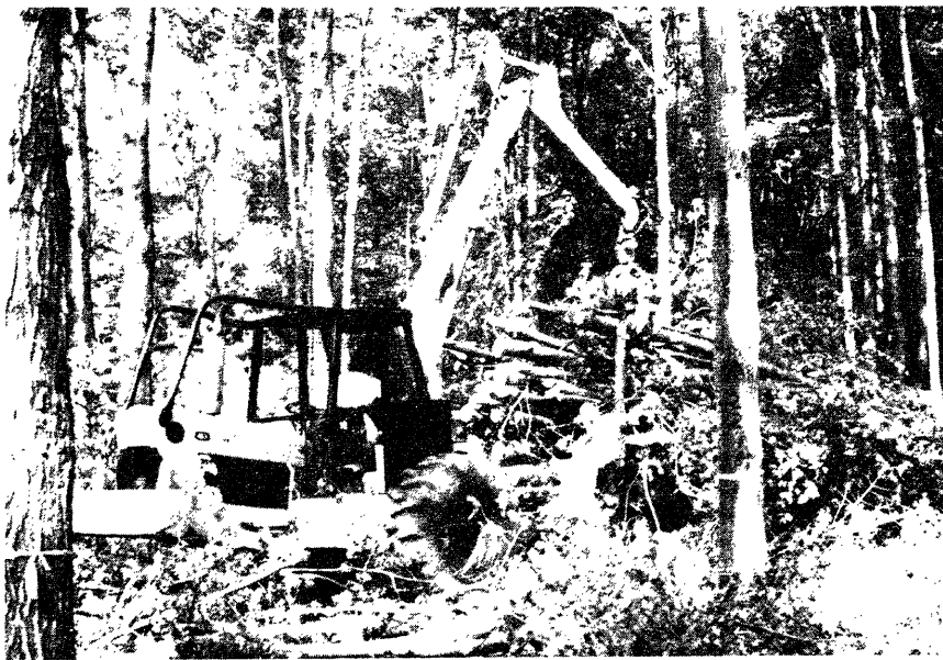
Figure 4.—Gafner Iron Mule forwarder extracting tree sections.
