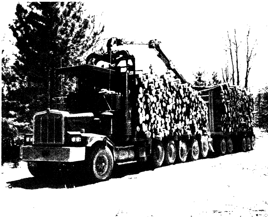
Figure 1.—The 11-axle Kenworth truck-trailer combination used in the study.
