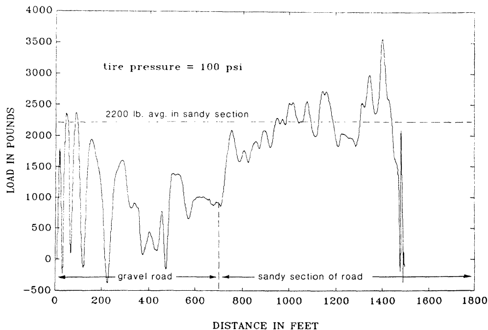
Figure 3.—Dynamic load measured in the trailer pull (rolling resistance) test on a "sugar sand" roadway with trailer tire pressure set at 100 psi. The moisture content of the "sugar sand" was 6 percent.
