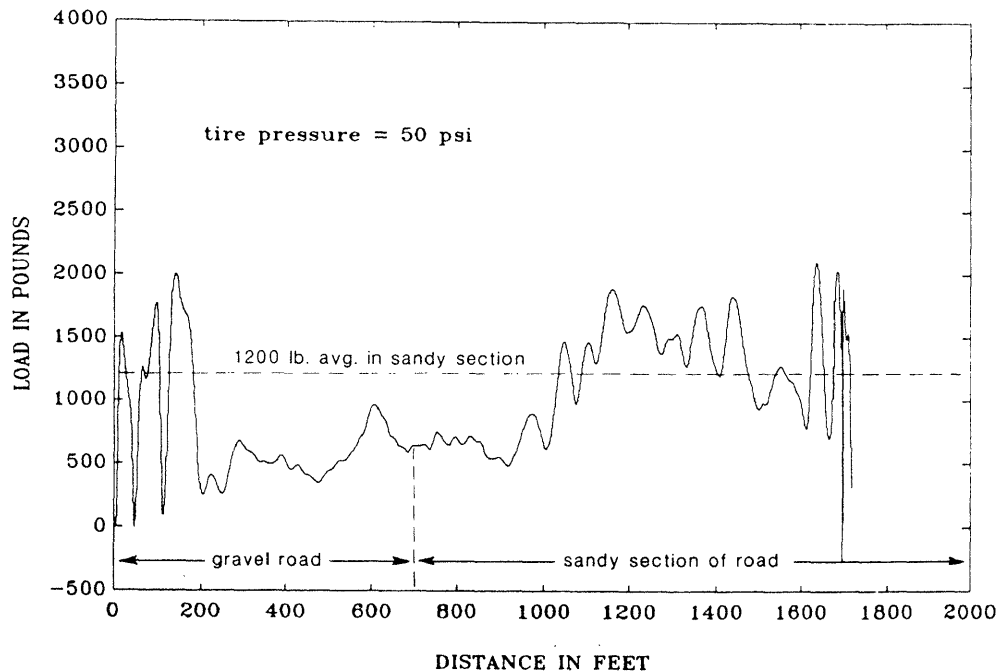
Figure 2.—Dynamic load measured in the trailer pull (rolling resistance) test on a "sugar sand" roadway with trailer tire pressure set at 50 psi. The moisture content of the "sugar sand" was 6 percent.
