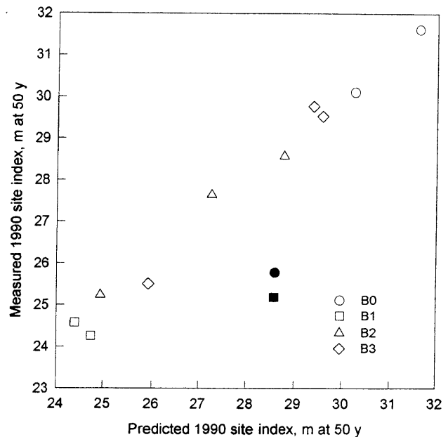
Figure 1.— The relationship between measured 1990 site index and site index predicted from eq. [6b], table 2. The shaded symbols are statistical outliers.
