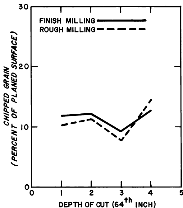
Figure 2.—The relation of chipped grain to a depth of cut, by rough and finish planing.
