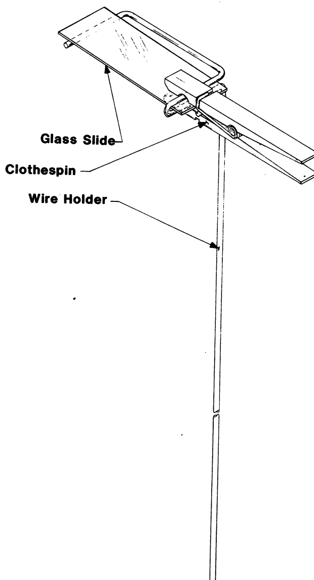
Figure 4.—Spore trap holder.
