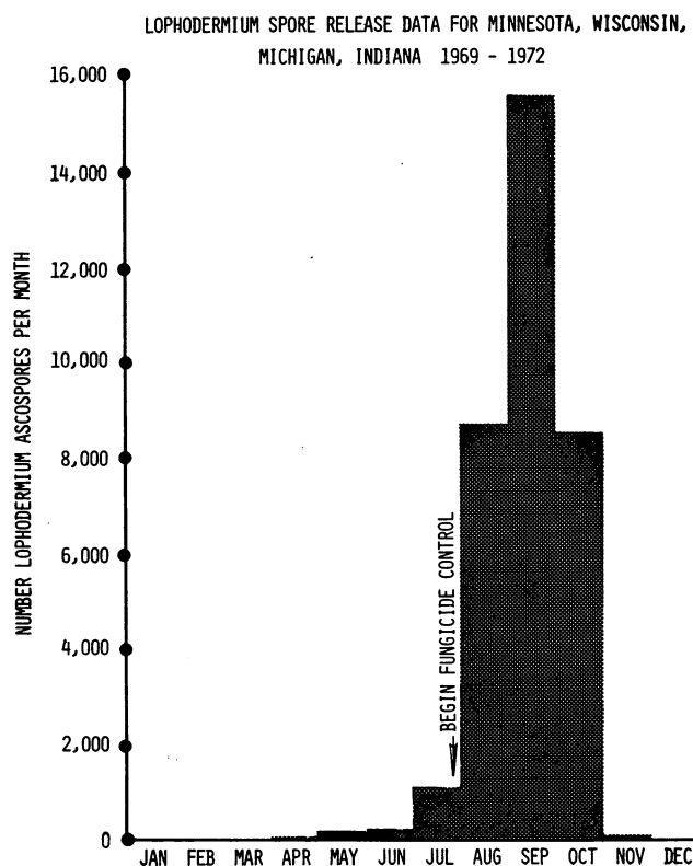
Figure 3.— Lophodermium spore release data for Minnesota, Wisconsin, Michigan, and Indiana showing how data can be combined to produce a regional spore dispersal graph that can help forest manager's initiate controls at the proper times.
