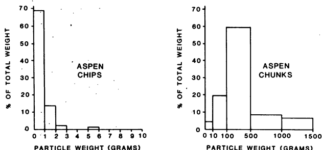
Figure 4.— Aspen particle weight distribution.
