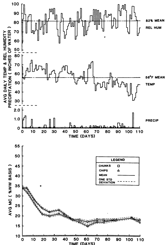
Figure 5.— Ambient conditions during sugar maple experiment and resultant drying curves.
