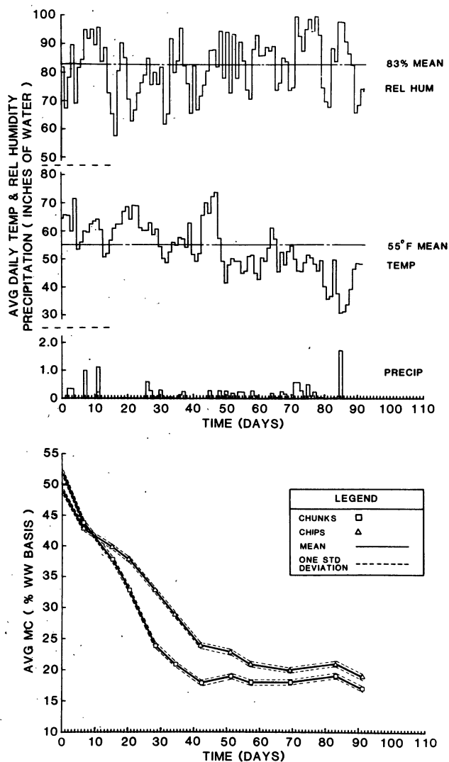
Figure 6.—Ambient conditions during aspen experiment and resultant drying curves.
