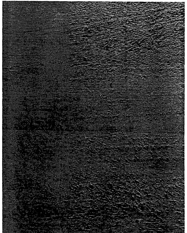
Figure 2.— Surface manufactured by cross-grain knife planing at 10 knife marks per inch, 1/8-inch depth of cut, and 45° rake angle.
