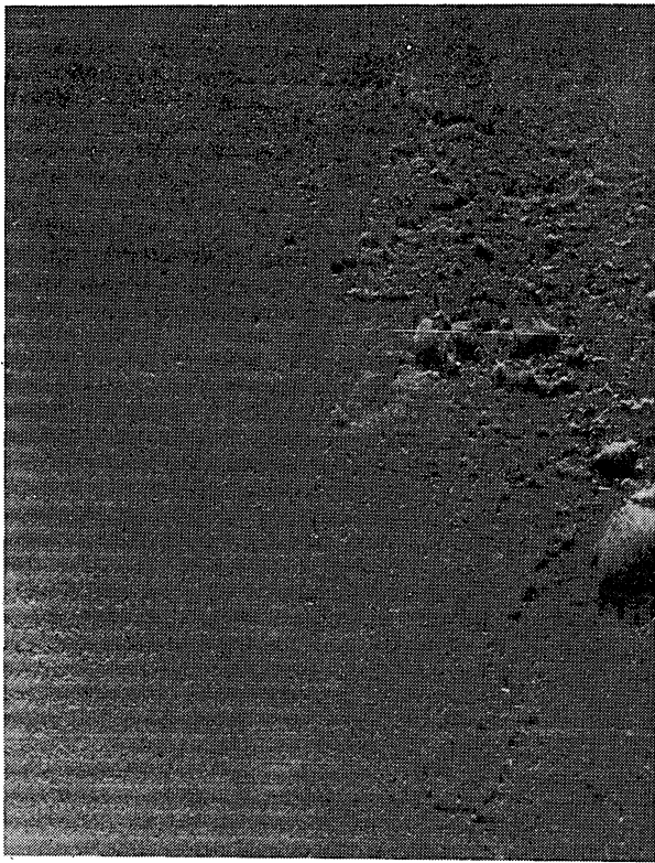
Figure 3.—Surface manufactured by knife planing parallel to the grain with cabinet planer at 20 knife marks per inch, 1/16-inch depth of cut, and 25° rake angle.
