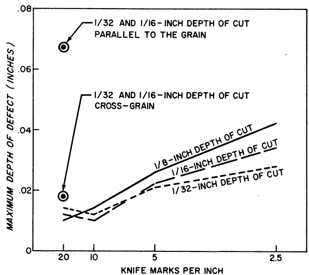
Figure 1.— Circles depict maximum depth of defect on surfaces planed across the grain and parallel to the grain on a cabinet planer with a 25° rake angle. Lines depict maximum depth of defect on surfaces planed across the grain on a molder with a 45° rake angle.
