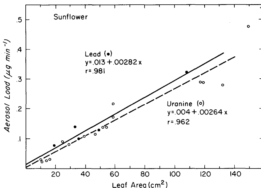
Figure 1. Comparison in aerosol deposition between \text{PbCl}_2 particles of 3.36 \mu\text{m} and uranine dye particles of 6.77 \mu\text{m} diameter on single streamlining leaves of sunflower. Aerosol load is the amount of particulate on the leaf after 10-35 min of deposition expressed on a per minute basis. Leaf area, determined from outline leaf tracings, is equal to the surface area of one side per leaf.
