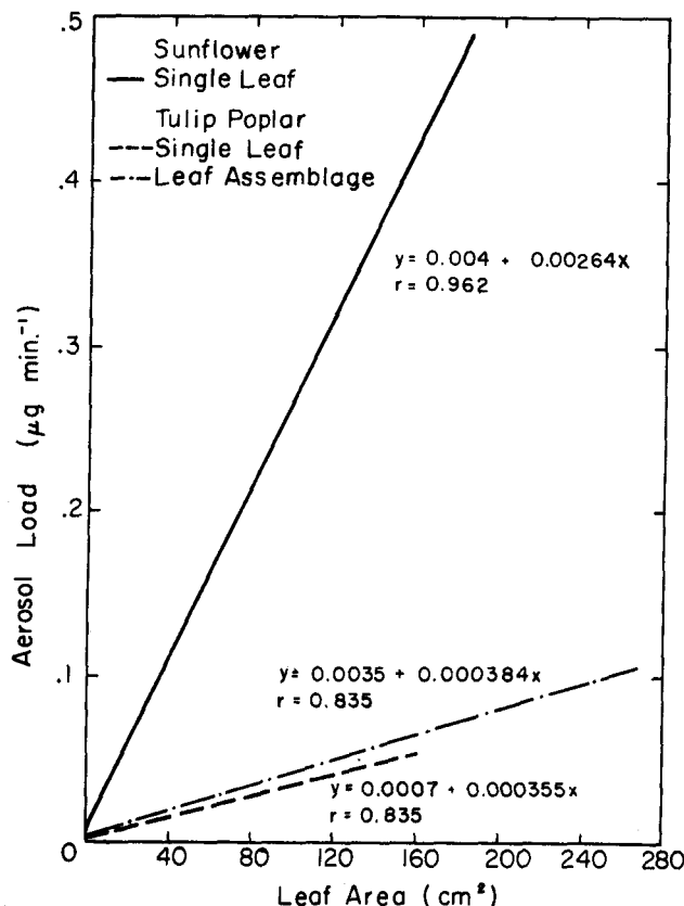
Figure 2. Deposition of uranine dye particles on single leaves and leaf assemblages of tulip poplar compared with single leaves of sunflower. Aerosol load and leaf area are expressed as in Figure 1.
