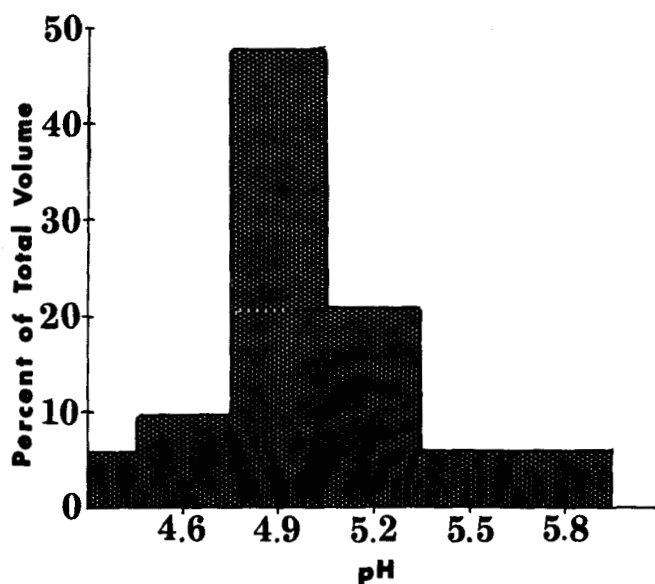
Figure 1. Frequency distribution of rain pH for Lacey, Washington, from November 5 to December 11, 1974.
