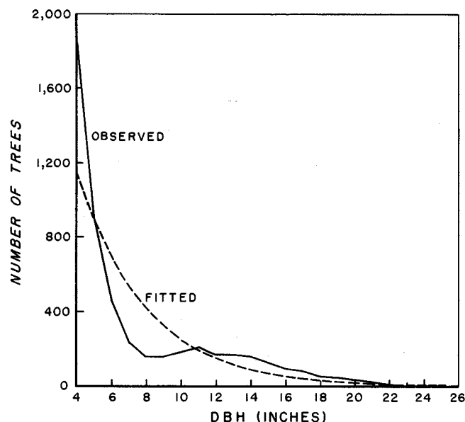
Figure 1.—Observed and fitted doubly-truncated exponential diameter distribution, uneven-aged loblolly-shortleaf pine stand (39 acres).
