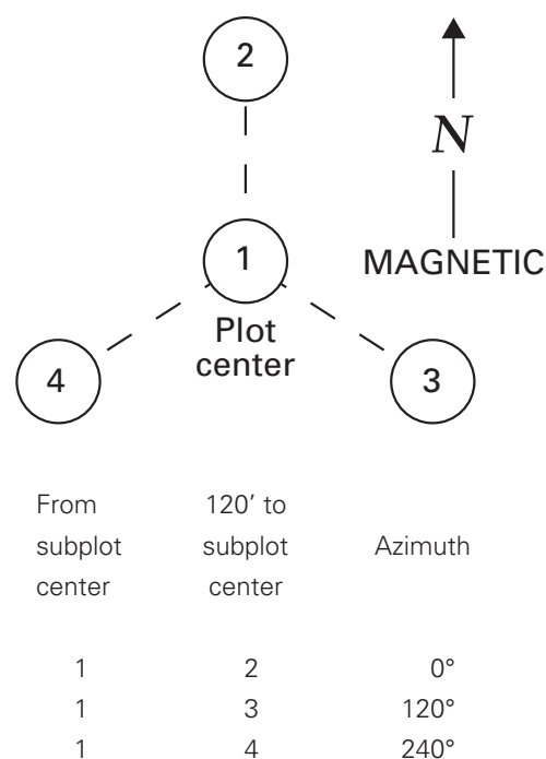
Figure 12.—Standard plot layout for 1998 Illinois inventory.
