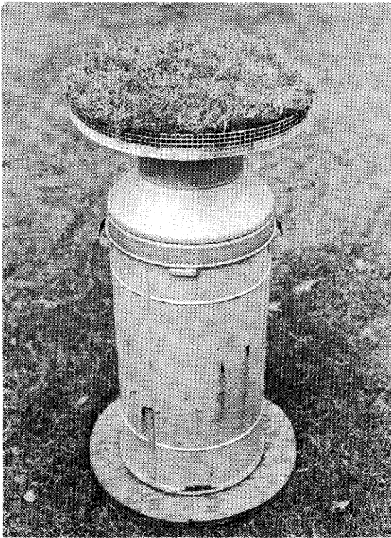
Figure 1. —Recording rain gage modified to measure dewfall. The live turf was used to provide a natural surface for collecting dew.
