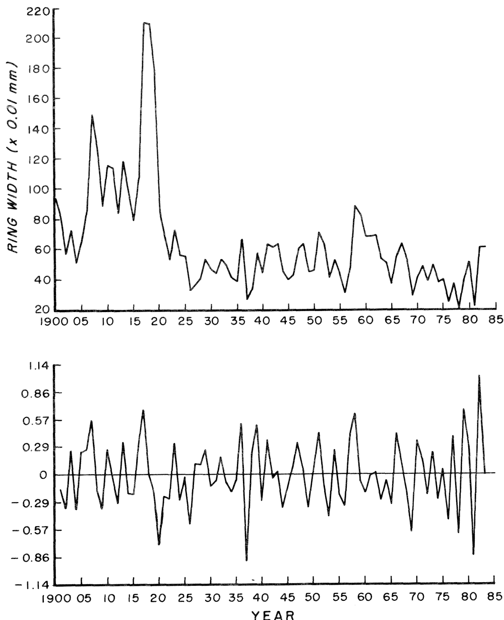
Figure 2.--Ring widths of an older red spruce in raw (upper graph) and standardized (lower graph) form for an old tree. First differences of the natural log were used to produce the lower standardized series.
