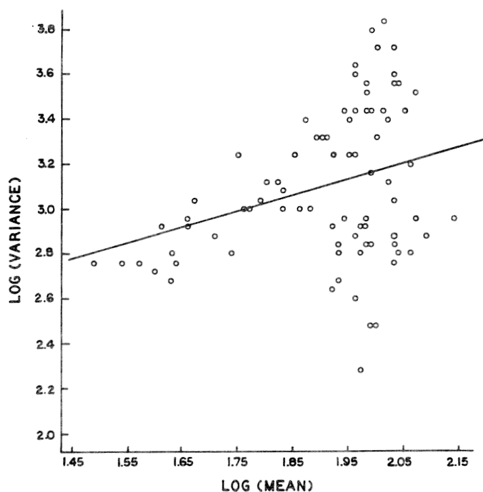
Figure 15.--Variance-mean plots (log-scale) of National Park Service site 316. All regressions are significant at p < 0.01 . This plot shows some nonlinearity.
