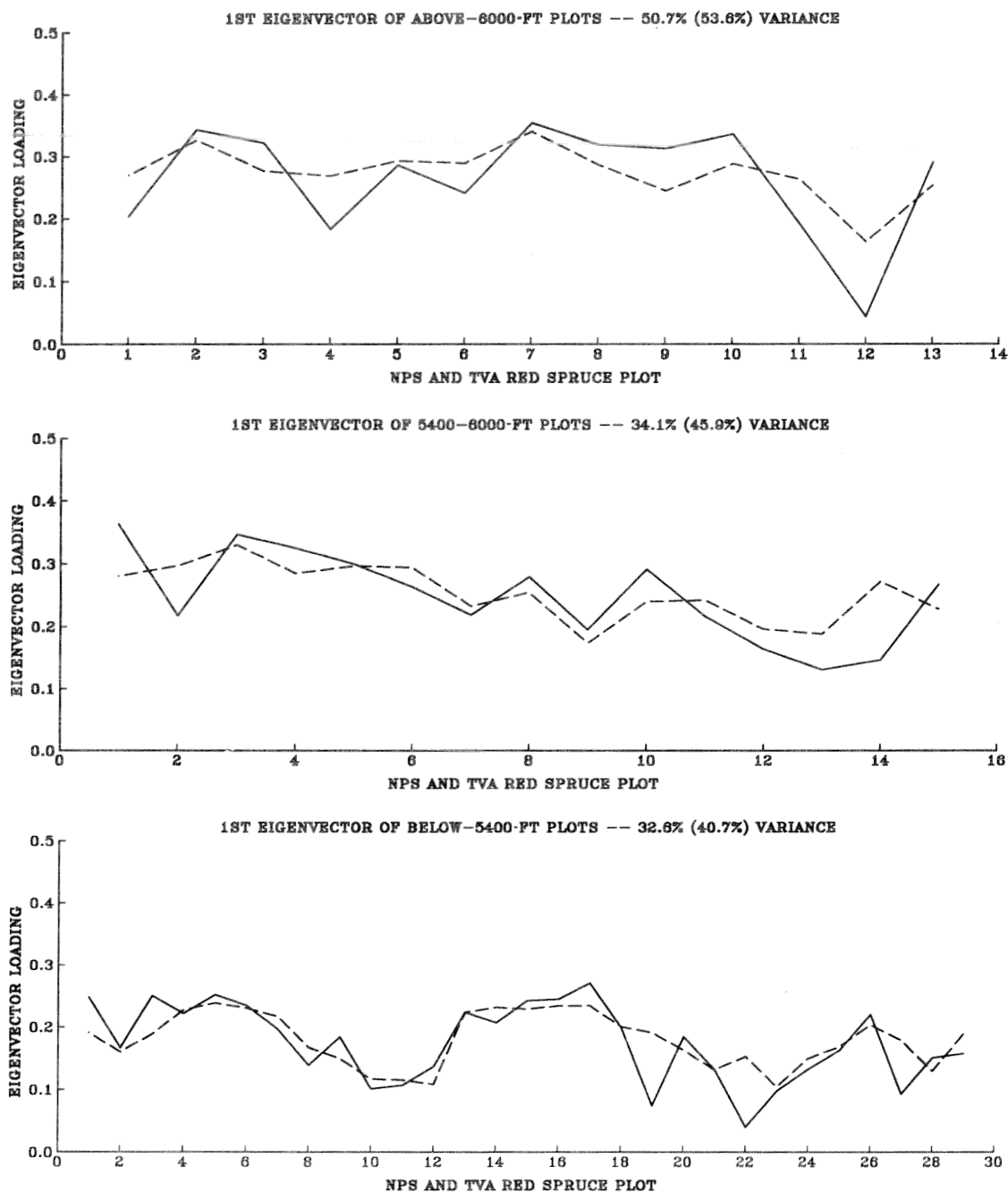
Figure 1.--The eigenvector loadings of the first principal component of each red spruce elevation stratum. The solid line plots correspond to the loadings of the original tree ring index chronologies. The dashed line plots correspond to the loadings of the same series after second-order autoregression has been removed from each one. The eigenvectors were extracted from the correlation matrix. The percent variance accounted for by each eigenvector, original (prewhitened), is indicated.
