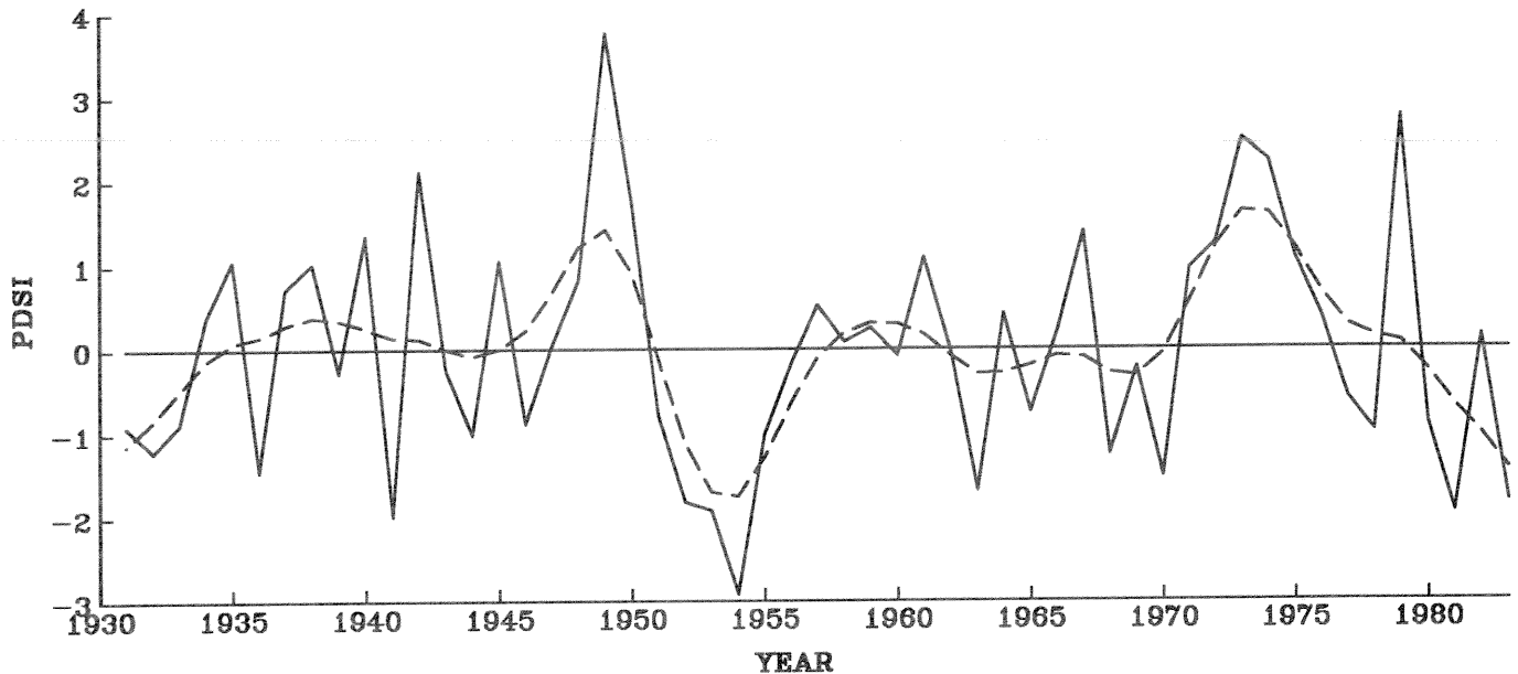
Figure 7.--July, August, and September average Palmer Drought Severity Indices (PDSI) series for the southern Appalachian Mountains. The dashed line highlights variance at frequencies less than 1/10 year.
