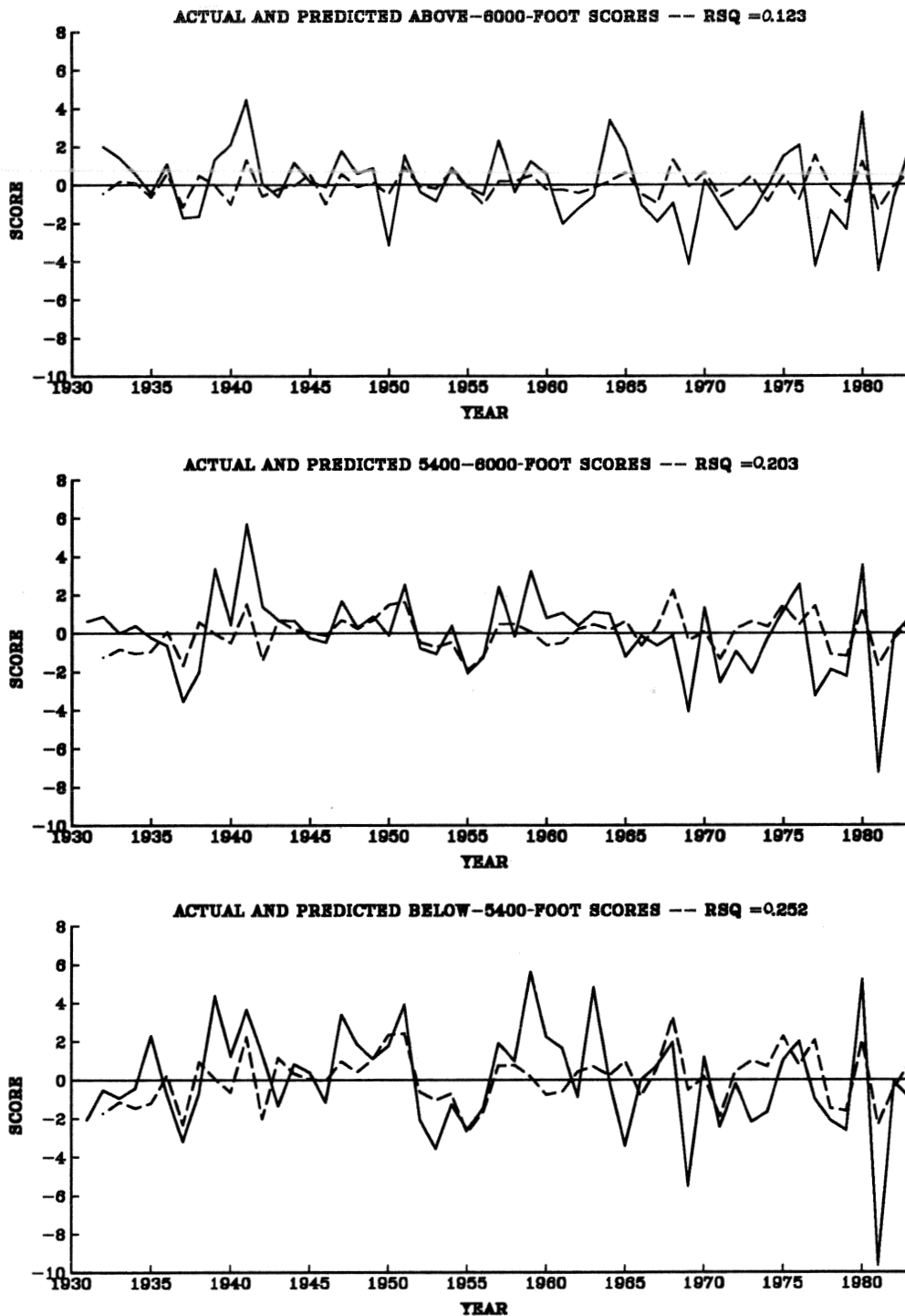
Figure 9.--Actual (solid) and predicted (dash) prewhitened tree ring scores. The predictors in the multiple regression analysis were summer temperature and summer drought. The R^2 of each model is indicated by the RSQ value.
