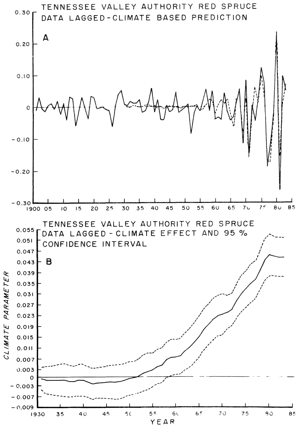
Figure 6.--Time trend predictions: A, Tennessee Valley Authority chronology (solid line) and its climate based prediction (dashed line) using the Kalman filter described by equations (6a), (6b), and (6c); B, the trend in the climate parameter given in equation 6a. The climate variable is a principle component (linear combination) of monthly average rainfall and temperature variables.
