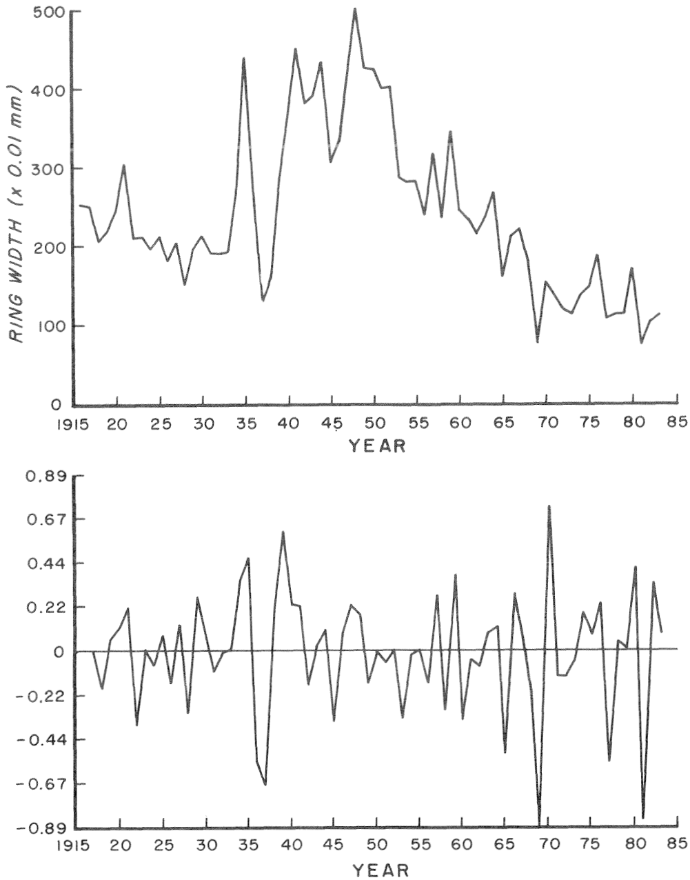
Figure 1.--Ring widths of a relatively young red spruce in raw (upper graph) and standardized (lower graph) form for a young tree. First differences of the natural log were used to produce the lower standardized series.
