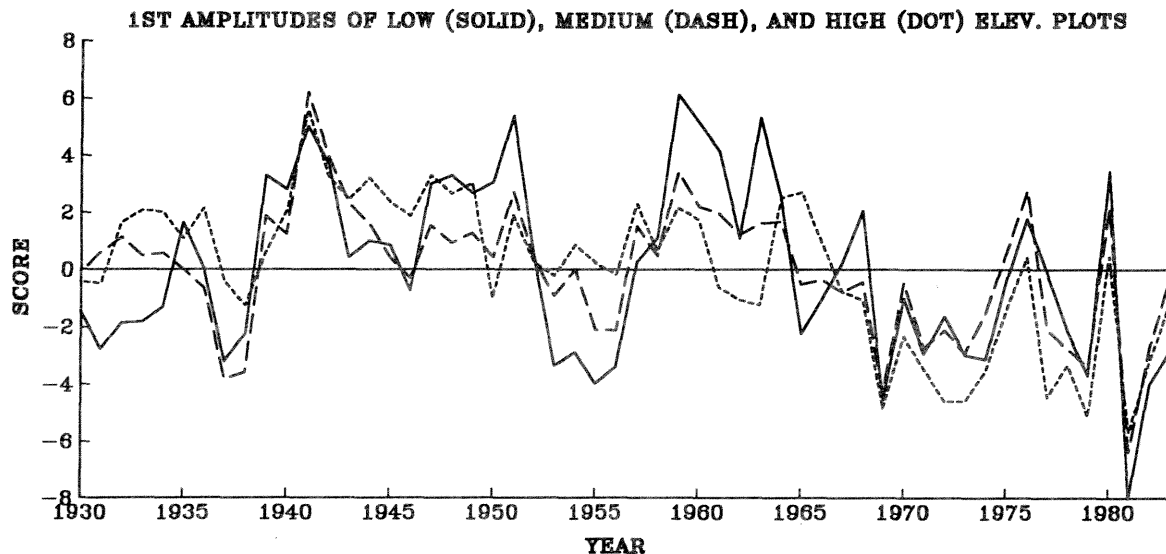
Figure 4.--The amplitudes of the original tree ring indices superimposed on each other. The purpose of this plot is to highlight certain time periods when elevation-related gradients in climate response are likely to be occurring.
