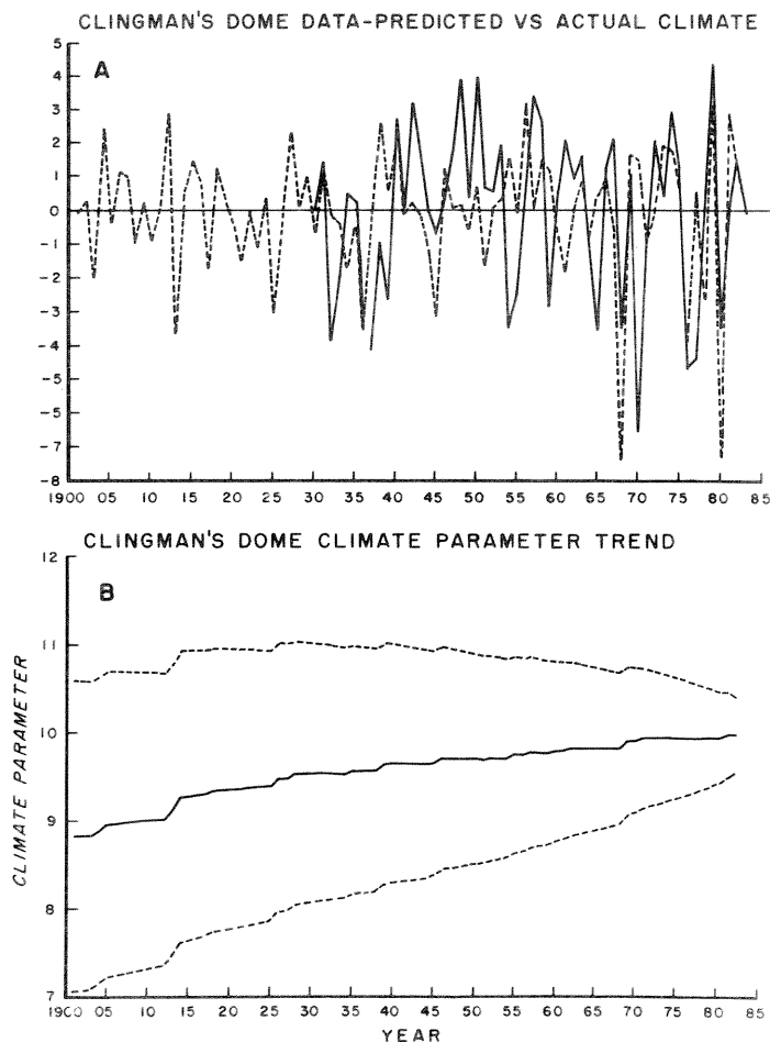
Figure 7.--Climate prediction: A, prediction (dashed line) of past climate obtained from tree ring data using the Kalman filter described by equations (7a) through (7d). The solid line is known climate, which is available back to 1931; B, the climate parameter trend and 95 percent confidence interval. This plot indicates that the uniformitarian principle does not hold here, since the parameter is trending toward zero.
