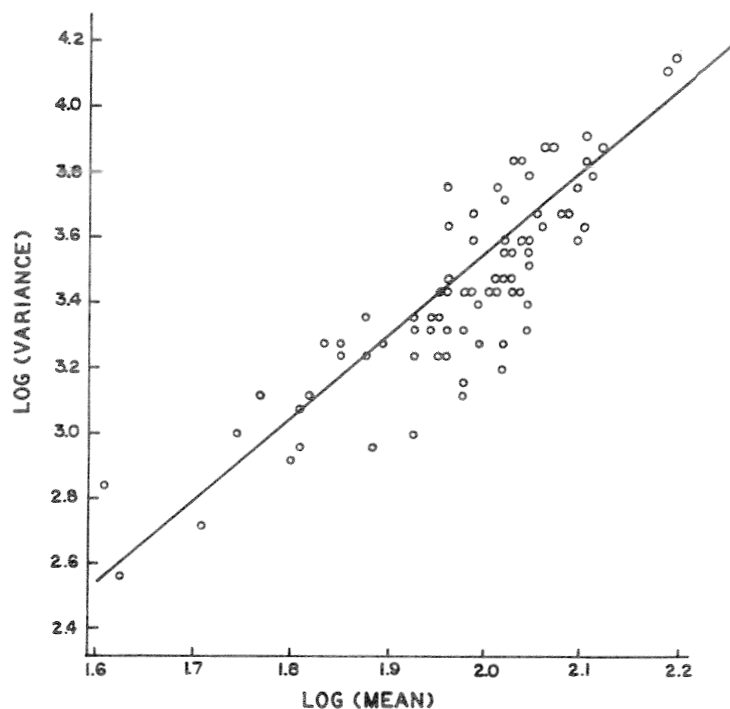
Figure 14.--Variance-mean plots (log scale) of National Park Service site 310. All regressions are significant at p < 0.01 . This plot shows very good regression.
