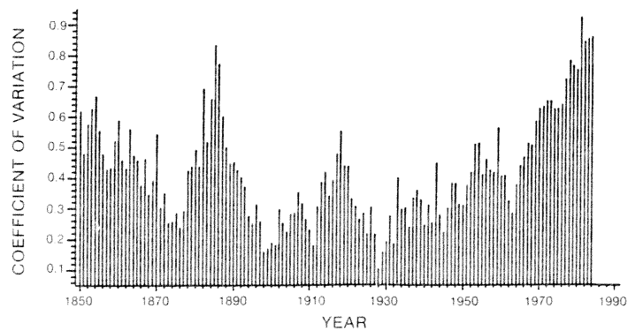
Figure 4.--Time series of mean, variance, and coefficient of variation of tree-ring increments from 1850 to 1984 at Tennessee Valley Authority site 36.
