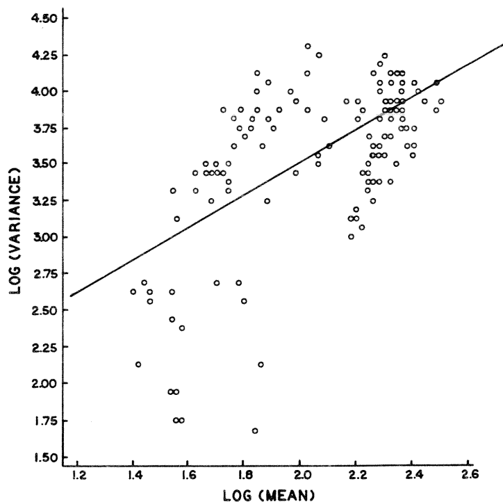
Figure 9.--Variance-mean plot (log scale) of Tennessee Valley Authority site 1. All regressions are significant at p < 0.01 . This plot shows some nonlinearity.
