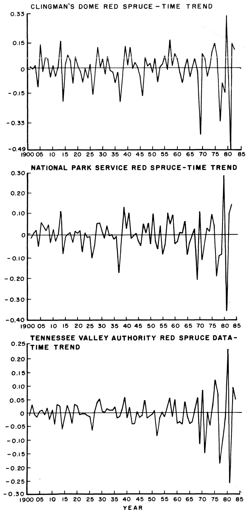
Figure 3.--Standardized chronologies from the Clingman's Dome, National Park Service, and Tennessee Valley Authority data sets. First differences of the log transform were used to standardize each tree ring series. A Kalman filter was used to produce the chronology as described in equations (6a), (6b), and (6c).
