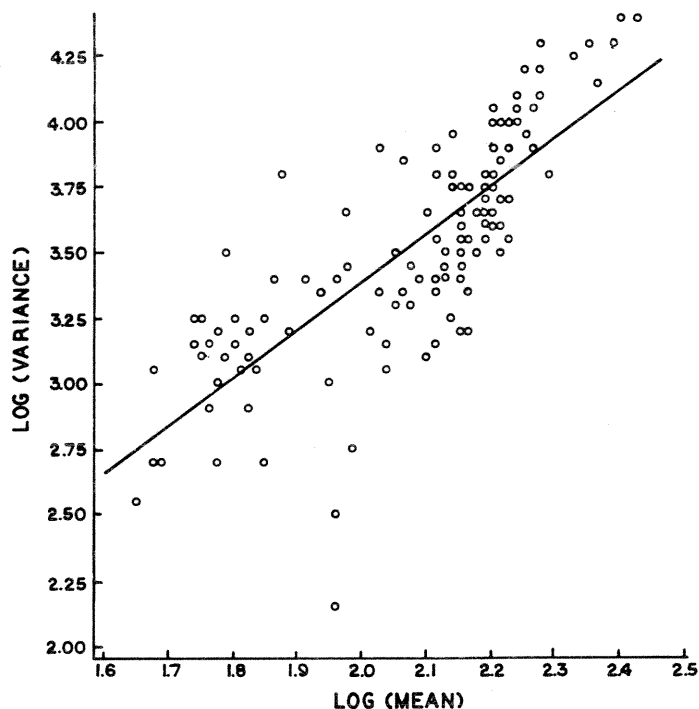
Figure 10.--Variance-mean plot (log scale) of Tennessee Valley Authority site 9. All regressions are significant at p < 0.01 . This plot shows very good regression.
