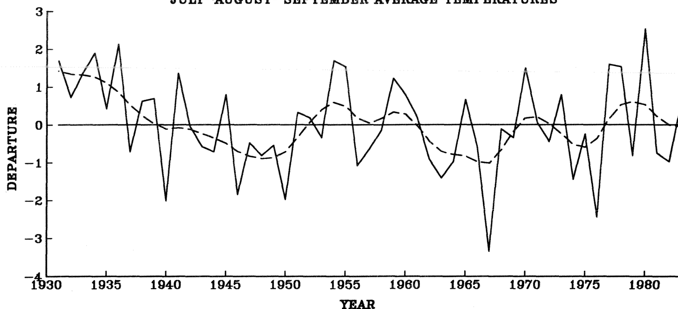
Figure 5.--July, August, and September average temperatures for the southern Appalachian Mountains since 1931. The dashed line highlights variance at frequencies of 1/10 year or less.
