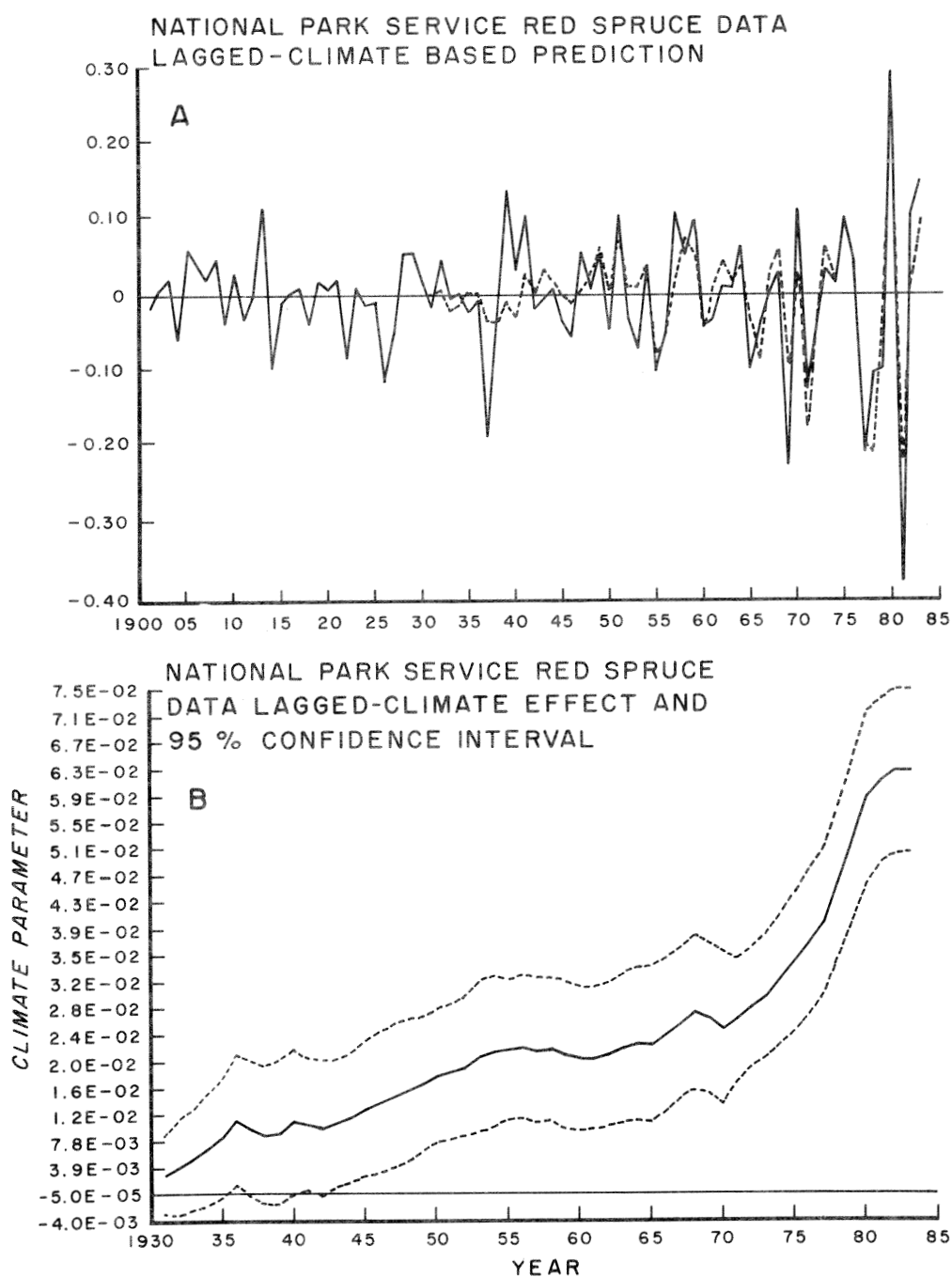
Figure 5.--Time trend predictions: A, National Park Service chronology (solid line) and its climate based prediction (dashed line) using the Kalman filter described by equations (6a), (6b), and (6c); B, the trend in the climate parameter with 95 percent confidence intervals, given in equation (6a). The climate variable is a principle component (linear combination) of monthly average rainfall and temperature variables.
