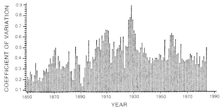
Figure 3.--Time series of mean, variance, and coefficient of variation of tree-ring increments from 1850 to 1984 at Tennessee Valley Authority site 23.
