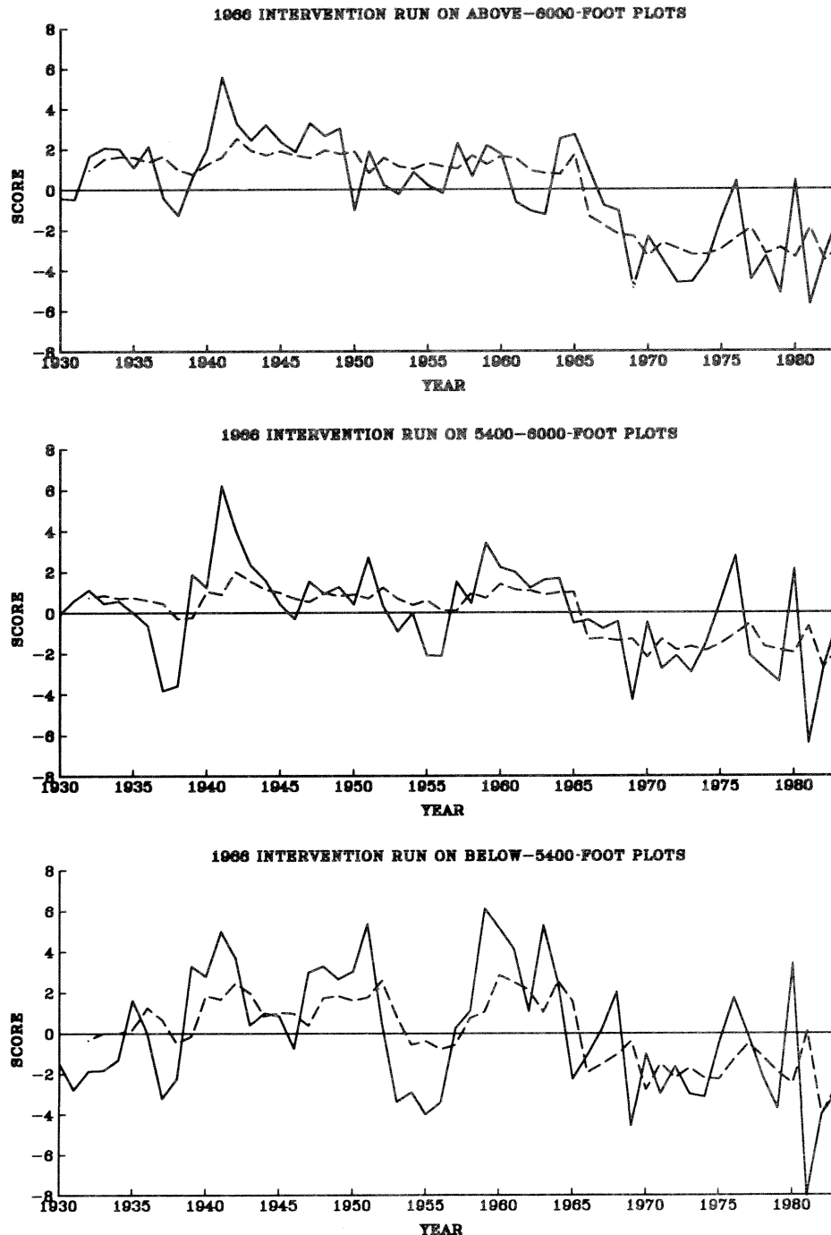
Figure 3.--The actual (solid) and estimated (dash) tree ring scores based on fitting a step intervention model to each series. The date of the intervention is 1966.
