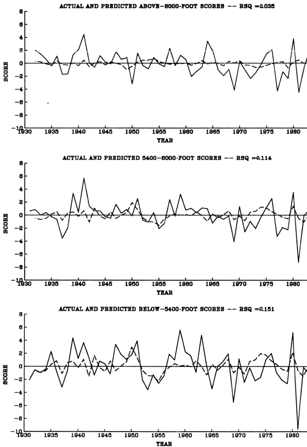
Figure 8.--Actual (solid) and predicted (dash) prewhitened tree ring scores. The summer PDSI series (fig. 7) was used as the predictor of tree rings. The R^2 of each model is indicated by the RSQ value.
