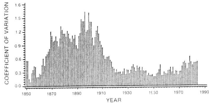
Figure 1.--Time series of mean, variance, and coefficient of variation of tree-ring increments from 1850 to 1984 at Tennessee Valley Authority site 1.
