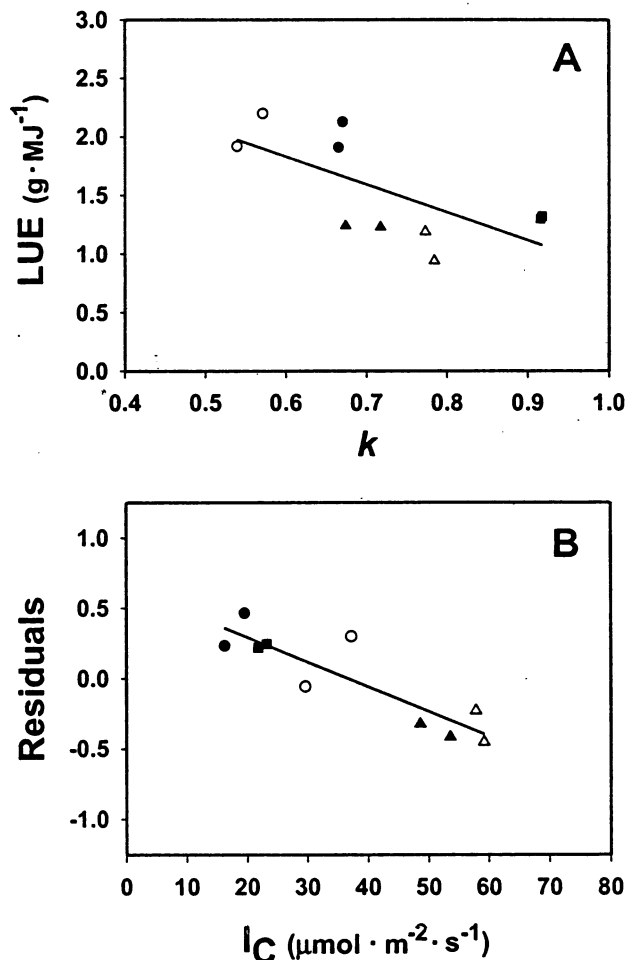
Fig. 1. Relations between (A) light-use efficiency (LUE) and canopy light-extinction coefficient ( k ) ( r^2 = 0.45 , P = 0.03 ), and between (B) residuals of the LUE versus k regression and leaf-compensation irradiance at the canopy base ( I C ) ( r^2 = 0.78 , P = 0.0007 ). Genotype symbols: 252-4, solid circles; D-105, open circles; Bucky, solid triangles; DN-34, open triangles; NM-6, solid squares.
