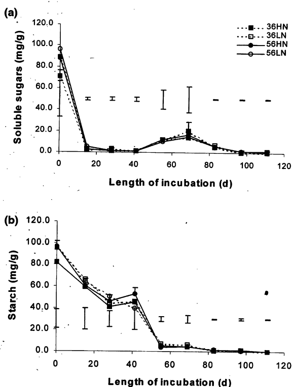
Fig. 1 Mean ( N=4 to 5 ) soluble sugar (a) and starch (b) concentrations in aspen leaf litter grown at ambient and elevated atmospheric \text{CO}_2 and two levels of soil N availability, incubated for 111 d at 25^\circ\text{C} . Bars are SE. I-beams are Fisher's least significant difference (LSD) for each a posteriori comparison of means. Figure legend: factorial combinations of atmospheric \text{CO}_2 partial pressure (36, 56 Pa), and high and low soil N availability (HN, LN), respectively.
