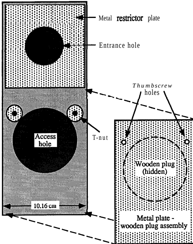
FIGURE 1. Front view of modified, artificial Red-cockaded Woodpecker cavity with a partial metal restrictor plate attached. Metal plate-wooden plug assembly is offset to show 7.7 cm access hole and placement of t-nuts in exterior of artificial cavity.
