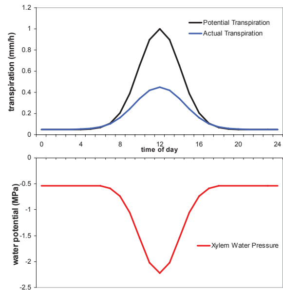
Figure 1: The difference between potential transpiration and actual transpiration expressed as xylem pressure (MPa).
