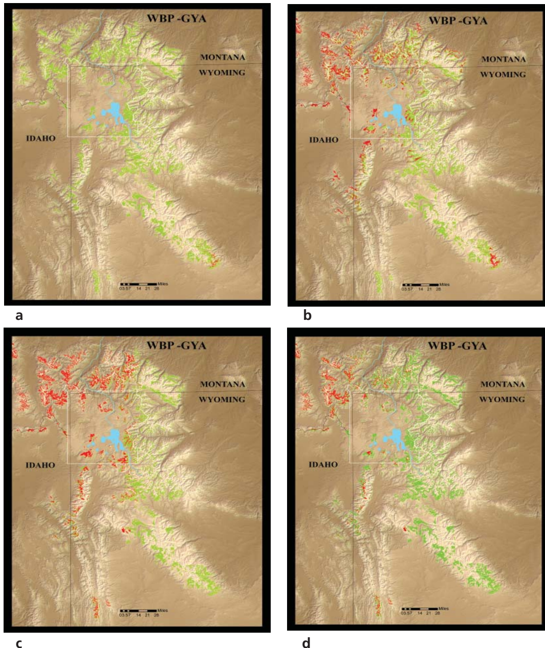
Figure 2. Simulations of mountain pine beetle adaptive seasonality for the greater Yellowstone area. Yellowstone National Park is outlined in white. Red indicates whitebark pine with probability of adaptive seasonality \geq 0.5 . a: Pre-warming climate based on temperature normals for 1951-1980. b: Current climate base on 1981-2010 normals [historic and VEMAP (Kittel et al. 1995) projected climate]. c: Projected warming (VEMAP) based on 2031-2060 normals. d: Historic normals (1921-1950) centered on the 1930s.
