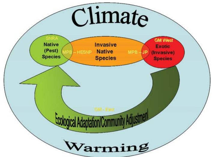
Figure 1. The historically exclusive concepts of native and exotic species are still valid; however, the rapid environmental change resulting from factors like climate warming are blurring the boundaries between these traditional categories. Changing climate has allowed some opportunistic species to invade new, heretofore-inaccessible, habitats. The interconnected relationship shown will be illustrated by four examples.
