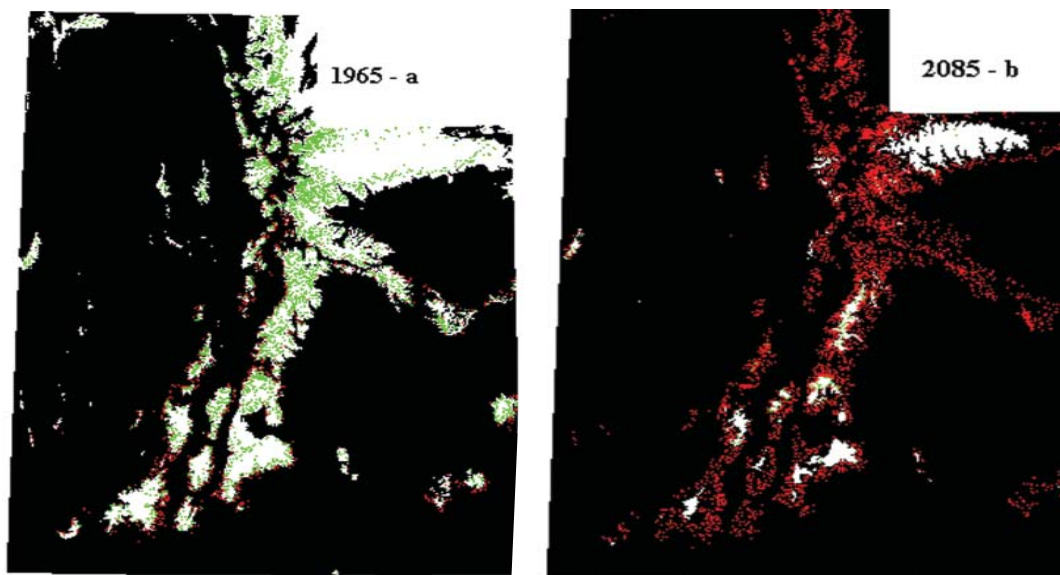
Figure 3. Black area indicates adaptive climate ( P \geq 0.5 ) for gypsy moth establishment. White area indicates climate is not adaptive ( P \leq 0.5 ) for gypsy moth establishment. Green indicates aspen in white area, red is aspen in the black area. Under current climatic conditions, approximately 10 percent of the aspen in the state was at high risk for establishment, and most of this was at the fringe of the aspen distribution. By end of the century more than 90 percent of aspen is projected to be at high risk.
