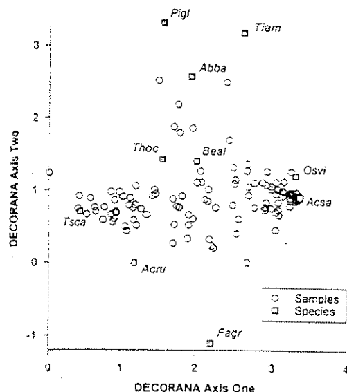
Fig. 4 Detrended Correspondence Analysis ordination of 138 plots measured in 1992-94. Symbols and species codes as in Fig. 3.
