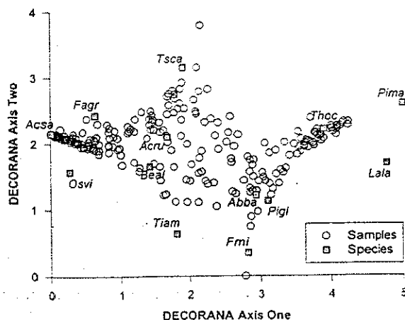
Fig. 3 Detrended Correspondence Analysis ordination of 240 plots measured in 1935 or 1948. Data are 1935 measurements except for 15 'transitional' plots which were not measured in 1935, but for which 1948 data were available. Filled circles are plot locations on first two axes of DCA ordination. Squares show DCA ordination of primary species on same axes. Species codes are: Abba = Abies balsamea , Acru = Acer rubrum , Acsa = Acer saccharum , Beal = Betula alleghaniensis , Lala = Larix laricina , Fagr = Fagus grandifolia , Frni = Fraxinus nigra , Osvi = Ostrya virginiana , Pigi = Picea glauca , Pima = Picea mariana , Thoc = Thuja occidentalis , Tiam = Tilia americana , Tscs = Tsuga canadensis .
